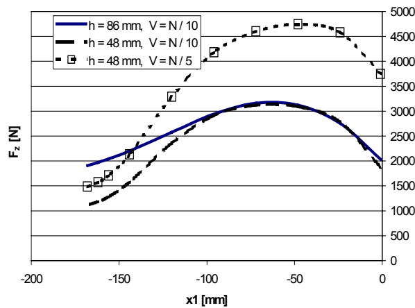
Figure 7: Tension force in the screw
