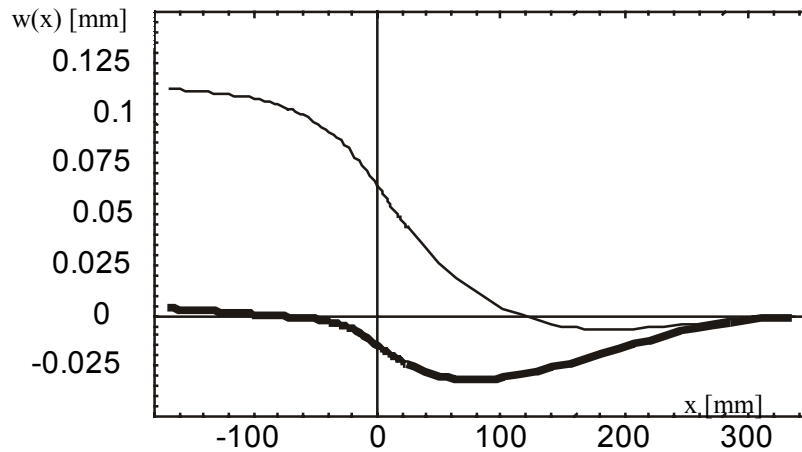
Figure 6: Deformation figure of reinforced (fat line) and non reinforced (thin line) beam model
