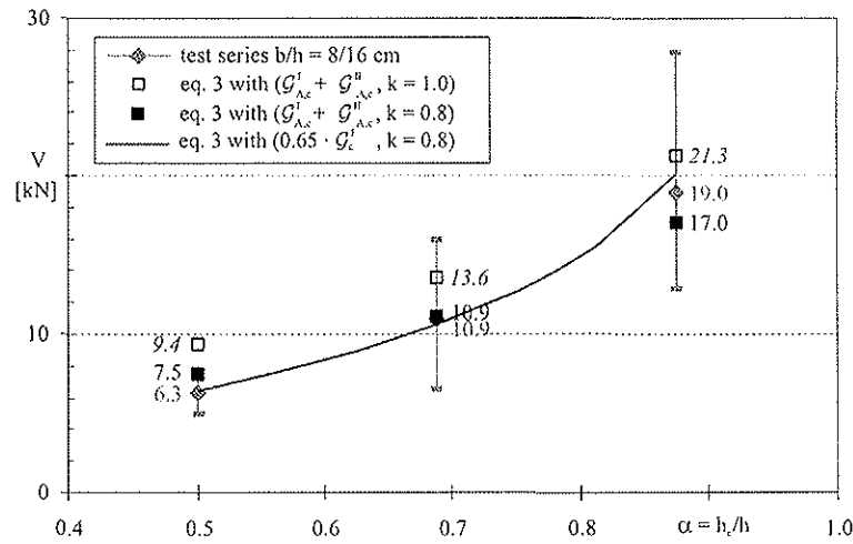
Figure 8 Experimental shear force capacities of the glulam series b/h = 8/16 cm in comparison to the calculated capacities according to eq. (3)
