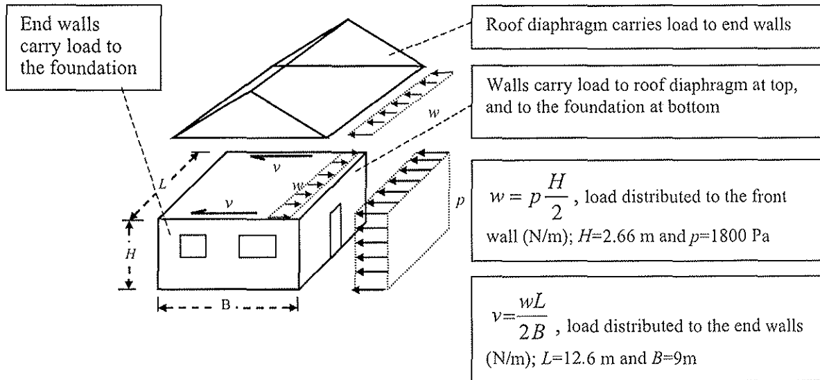
Figure 12: Lateral load distribution due to wind load
