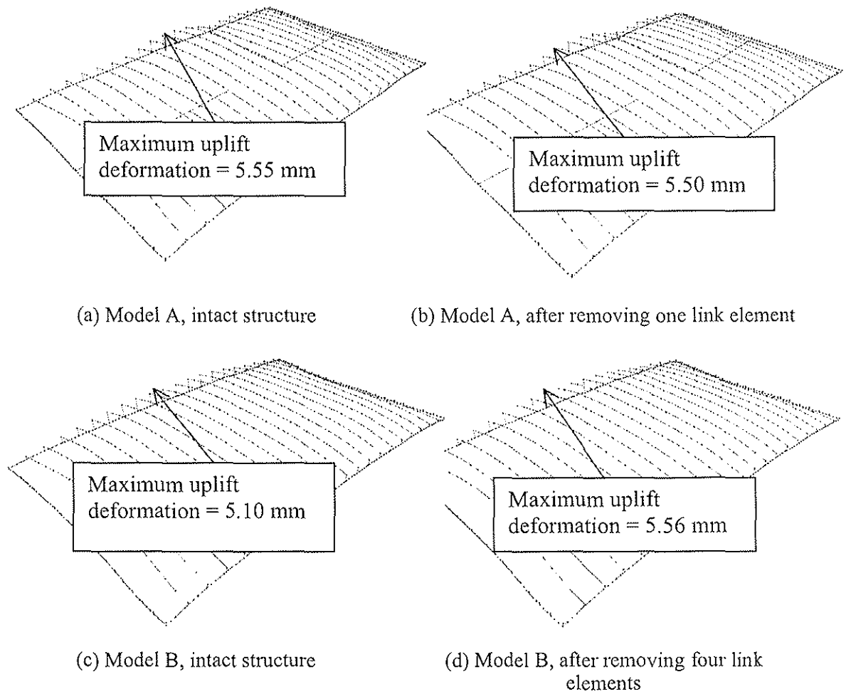
Figure 7: Deformed shapes at the roof-to-wall junction
