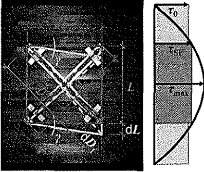
Fig. 4: Shear field and declaration of \tau_0 , \tau_{max} and \tau_{SF}
