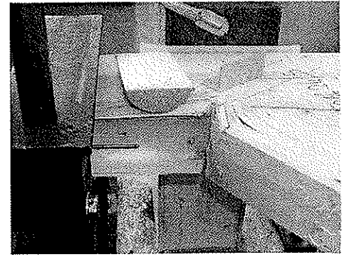
Figure 5 : Mixed failure: compression in contact zone and shear in notch (series with \beta = 55^\circ ).
