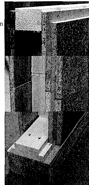
Fig. 4 Details of Prefabricated Timber Wall Element System
