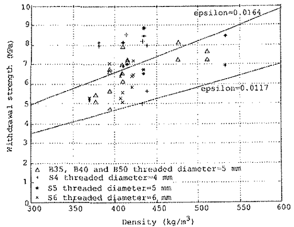
Figure 2. Withdrawal strength for screws. F_{ax} = \epsilon d \pi (l_e - d) \rho . The upper line represents the mean value, the lower the characteristic value. (Hansen, 2002).
