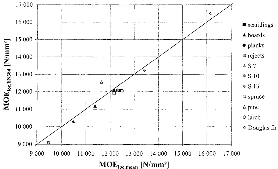
Fig. 8: MOE_{loc,EN384} over MOE_{loc,mean} , n = 3947 specimens.
