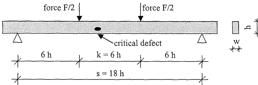
Fig. 1: 4-point-bending test acc. to EN 408.
