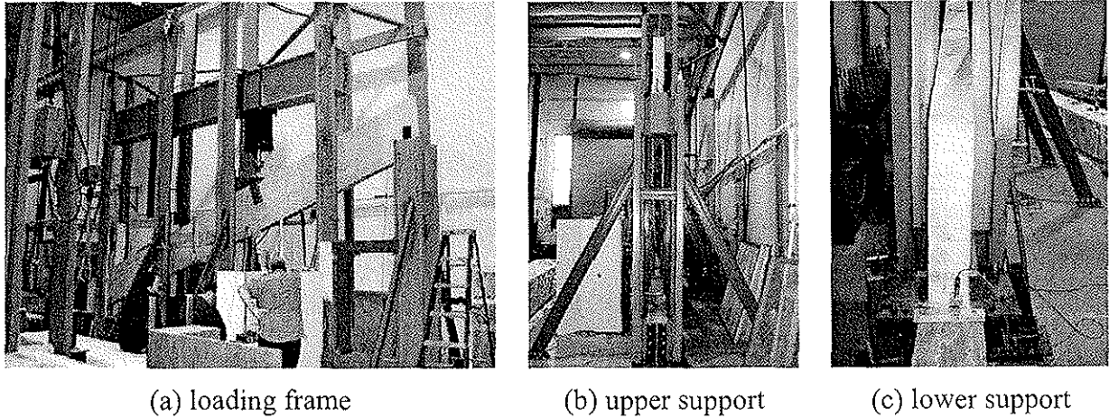
Figure 3: Test apparatus
