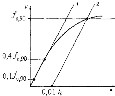
Figure 4. Load-deformation curve for compression perpendicular to the grain, definition of compression strength f_{c,90} at 1% off set.
