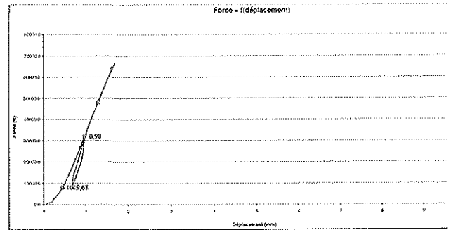
Figure 7 : Load/displacement curve for test with \beta = 25^\circ (specimen 2, Serie2).
