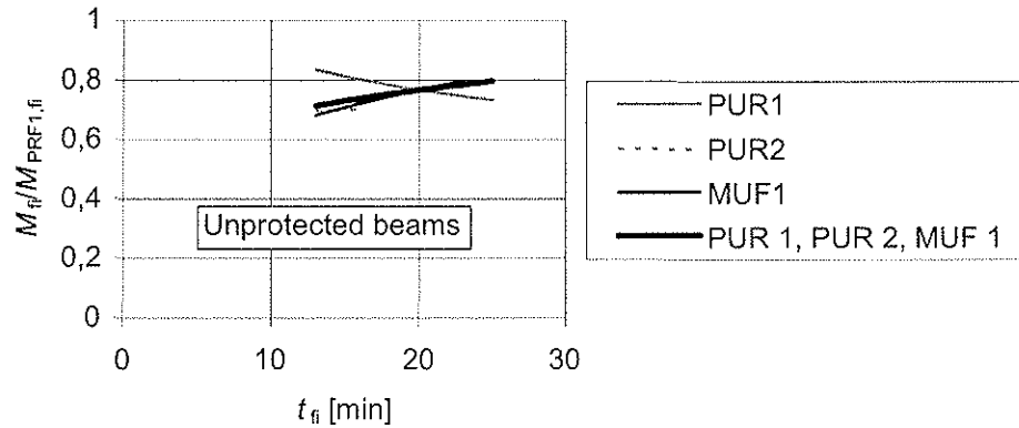
Figure 13 – Relative moment resistance of unprotected beams: Comparison of series PUR 1, PUR 2 and MUF 1 with series PRF 1.
