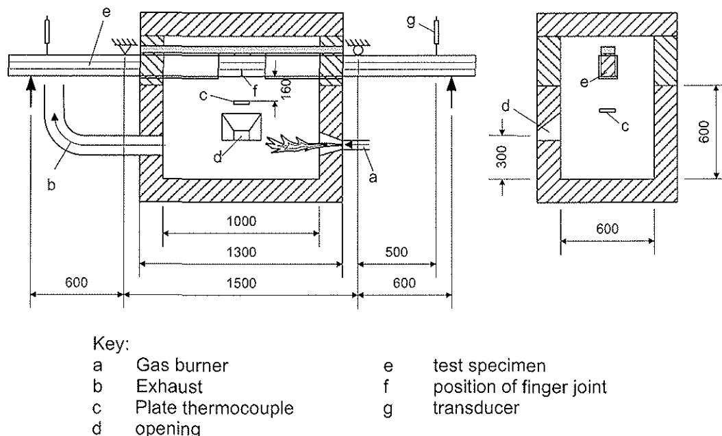
Figure 6 – Test set-up: Small-scale furnace and position of supports and load introduction
