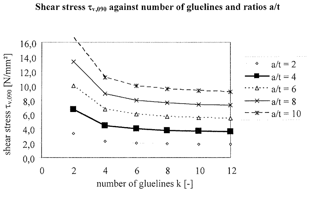
Fig. 5 Shear stress \tau_{v,90} against number of gluelines k and ratios a/t
