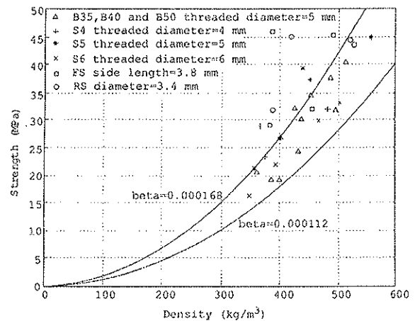
Figure 4. Embedment strength perpendicular to the grain for nails and screws. F_e = \beta d \rho^2 . The upper line represents the mean value, the lower line represents the characteristic value for all types. The nails alone could be assigned higher values. (Hansen, 2002).
