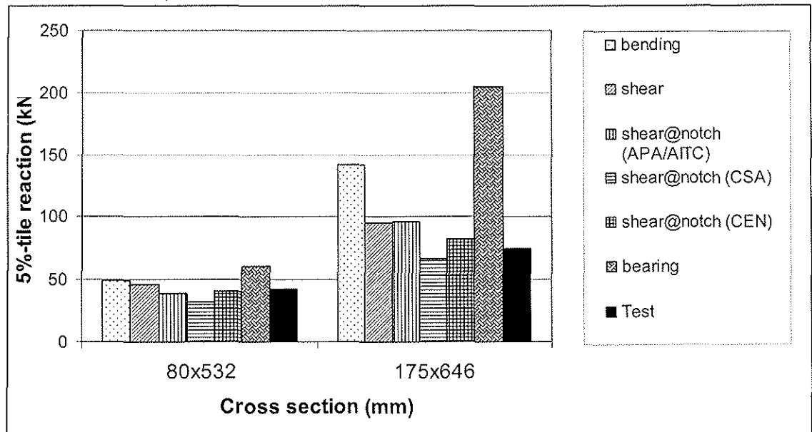
Figure 7: 5-percentile reaction forces, comparison of code expected and test values for 'standard term' load conditions
