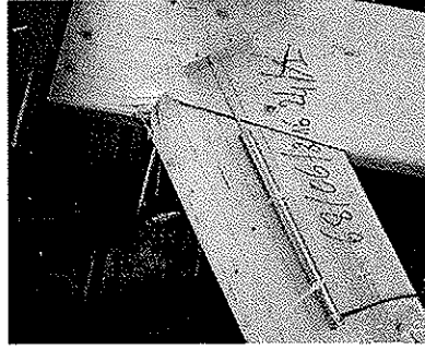
Figure 4 : Compression failure in contact zone of elements A and B (series with \beta = 55^\circ ).
