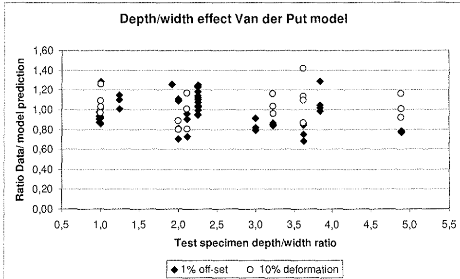
Figure 15: Effect of specimen depth and width ratio.
