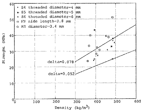
Figure 1. Pull-through strength for nails and screws. F_{head} = \delta d_{head}^2 \pi / 4 \rho . The upper line represents the mean value, the lower the characteristic value. (Hansen, 2002).
