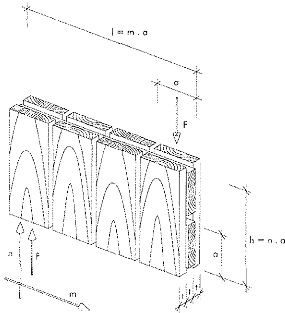
Fig. 4 Cross laminated timber element as shear field
