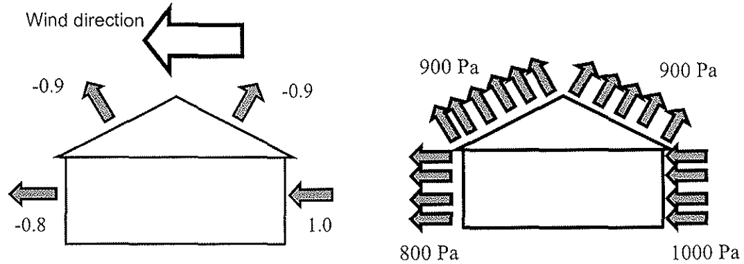
(a) Values of wind pressure coefficient C_qC_p
