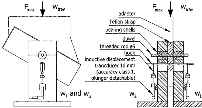
Figure 2.1: Test configuration
