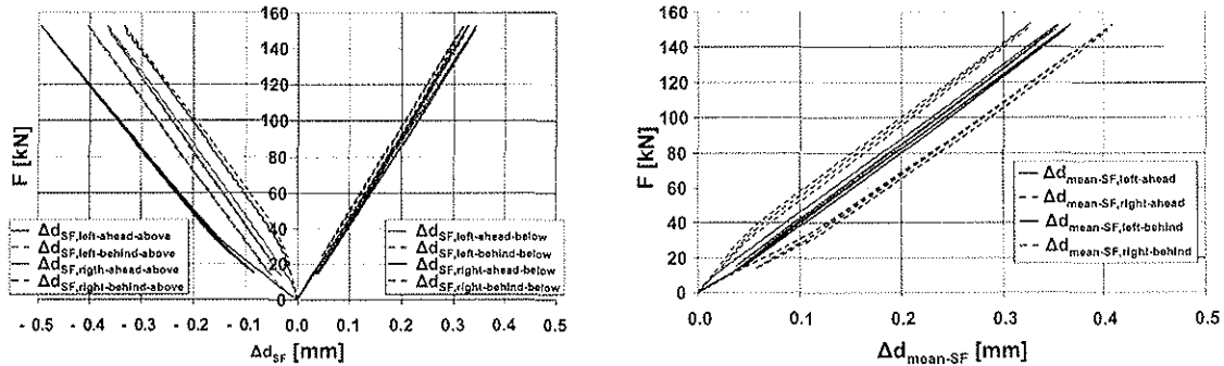
Fig. 7: Bending test diagrams: measurement of extensions of shear-field diagonals in relationship to applied force (applied force corresponds to 50 % of estimated F_{\text{max,mean,est}} ) – elongation of each shear-field diagonal measurement (left), mean elongation of each shear-field diagonal (right)
