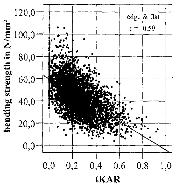
Fig. 5: Bending strength versus tKAR, n = 3899 specimens.
