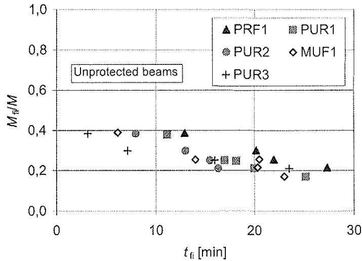
Figure 9 – Relative bending resistance (load ratio) vs. time to failure of unprotected beams
