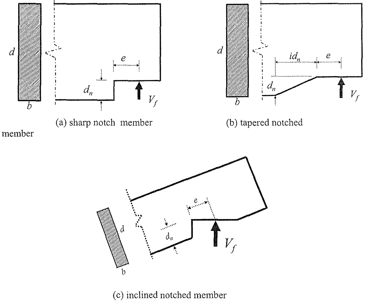
Figure 1: Notched geometry
