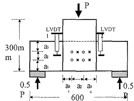
Figure 2: Layout of screws or nails in LVL loaded perpendicular to strong axis
