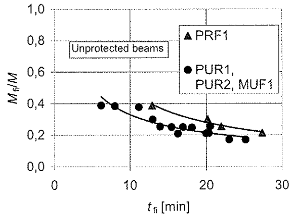
Figure 12 – Fitting of regression curves to test results
