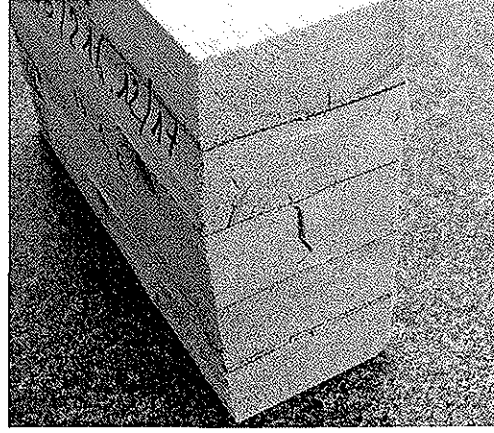
Figure 9 : specimen after failure (280*225*90 mm 3 .)
