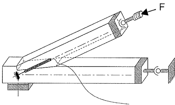
Figure 2 : test configuration.
