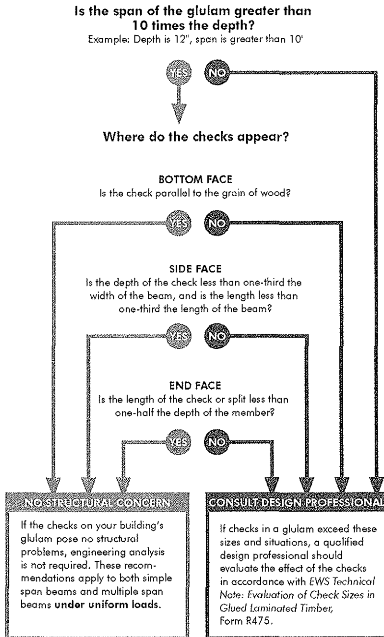
Figure 9. Guidelines for evaluating glulam checks
