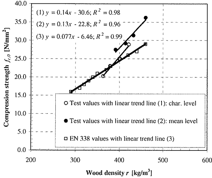
Fig. 8: Relationship between compression strength parallel to the grain f_{c,0} and wood density \rho : test results and EN 338 values.
