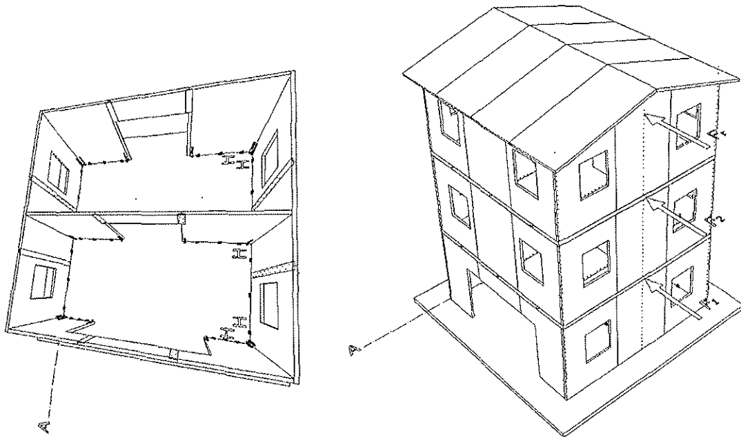
Figure 4: Distribution of holddown anchors and steel angles at ground floor and distribution of seismic forces at each floor. In the left side picture, the holddown anchors marked with H are those taken into account in the design.
