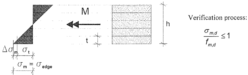
Figure 2 Assumed stress distribution over a GLT cross section due to bending for the verification process
