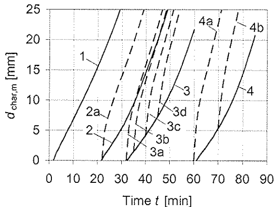
Figure 11 – Charring depth vs. time in the middle of the flange
