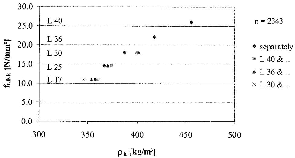
Figure 4: Relationship between f_{t,0,k} and \rho_k for different strength classes and strength class combinations.
