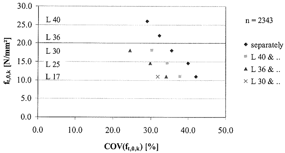
Figure 3: Relationship between f_{t,0,k} and COV(f_{t,0,k}) for different strength classes and strength class combinations.
