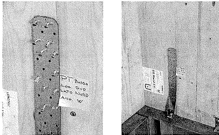
Figure 5: Holdown failure after Nocera Umbra 1.2g test.
