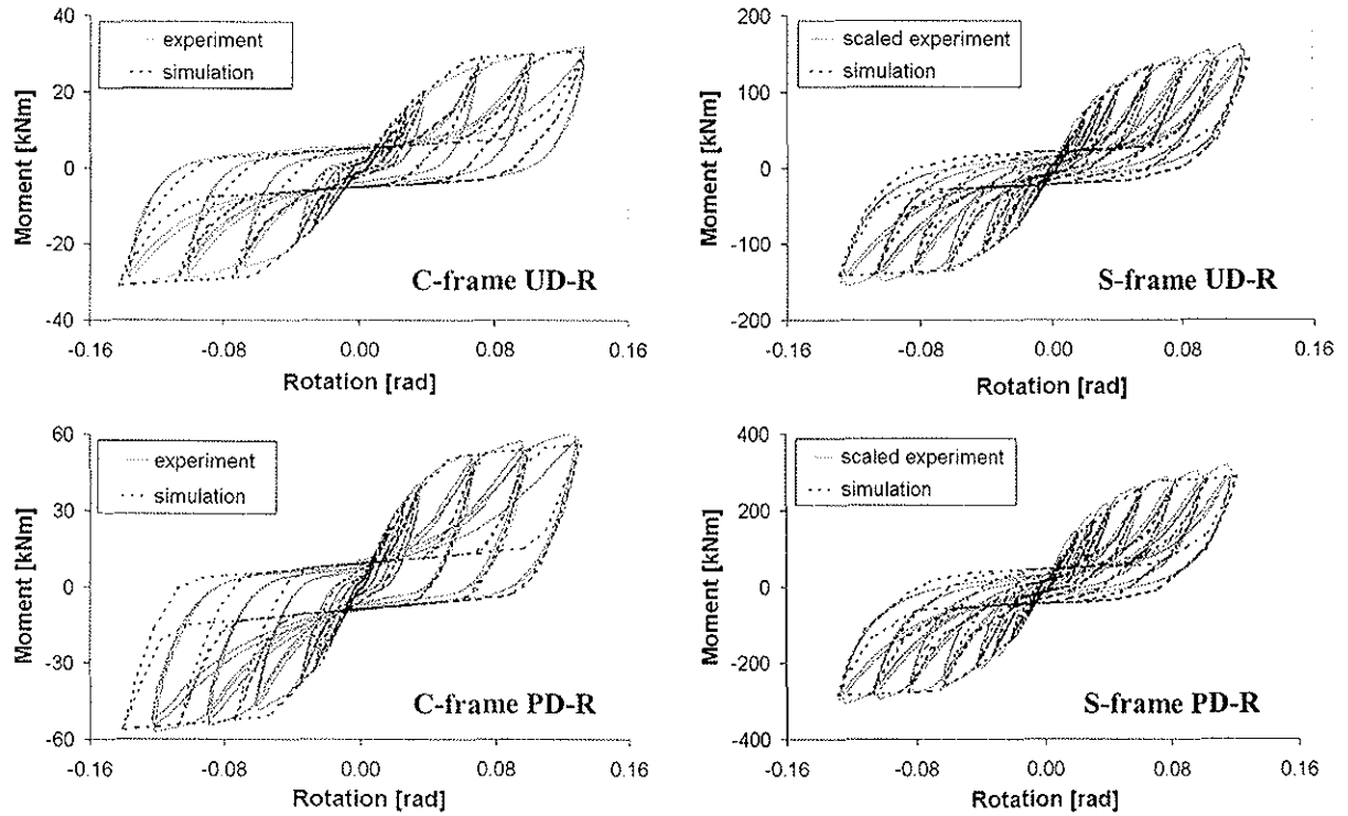
Figure 1. Moment-rotation relationship of the simulation versus experiment
