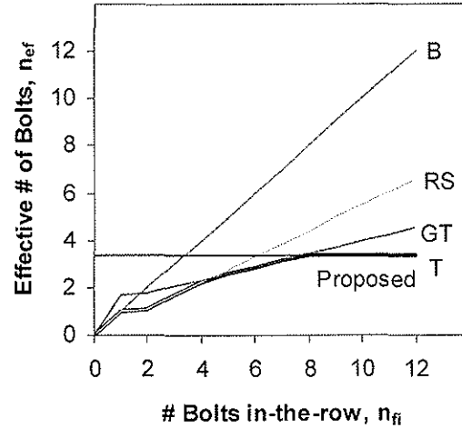
Figure 5 – Effective Number of Fasteners for Proposed Design Approach
