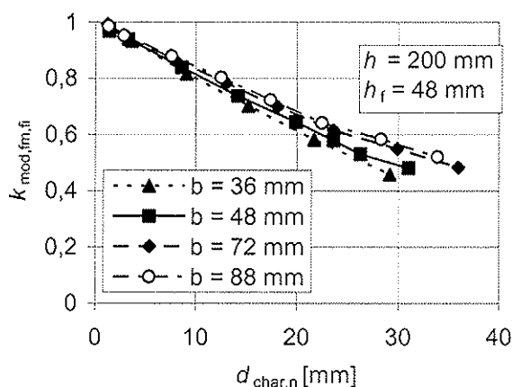
Figure 21 – Effect of flange width on modification factor for bending strength
