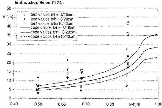
Fig. 5: Comparison of fracture loads with 5%-quantile and the values of DIN 1052:2004-08 with f_{v,k}=0,7 \cdot 3,5 \text{ N/mm}^2 Fig. 6: Comparison of fracture loads with 5%-quantile and the method by Gustafsson with G_c = 0,3 \text{ N/mm}
