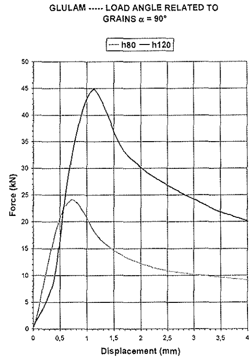
(b) Test Load Angle \alpha = 90^\circ
