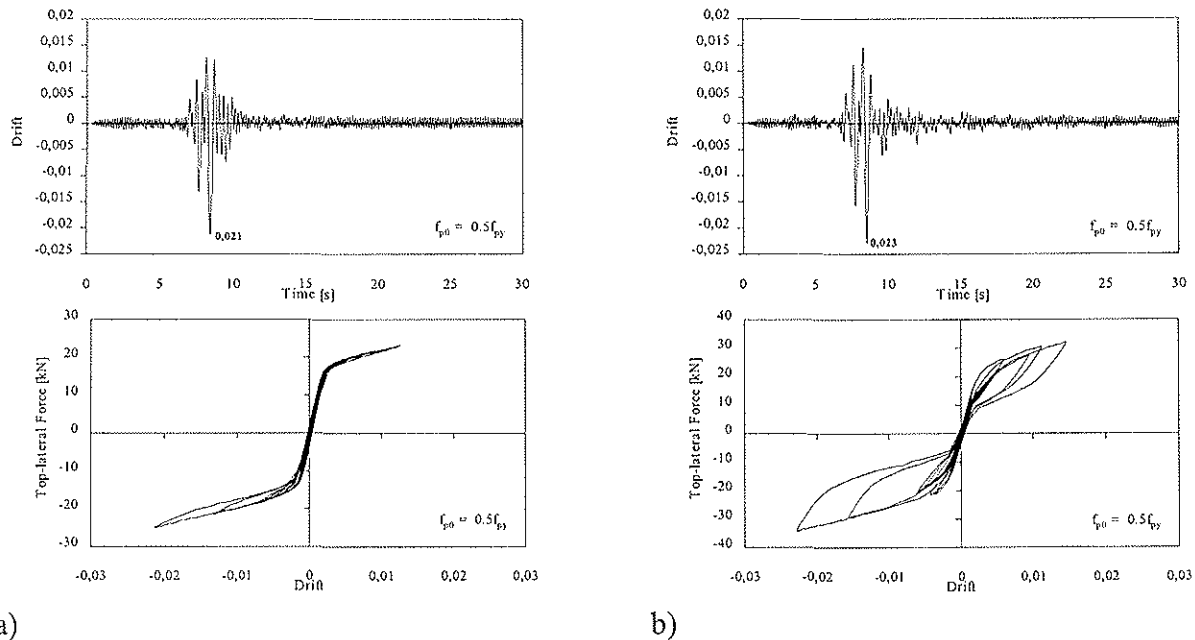
Figure 10 Pseudo-dynamic experimental test response of cantilever column-to-foundation systems a) unbonded post-tensioned only (under 100% input motion) b) hybrid system (under 150% input motion)
