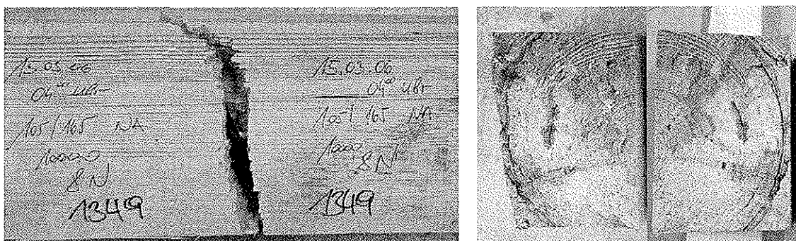
Fig. 4: Tensile strength = 6.4 \text{ N/mm}^2 due to compression damage of the timber (Spec.Nr.1349)
