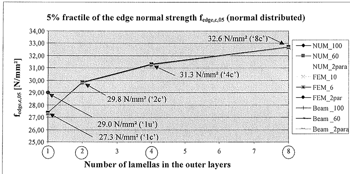
Figure 11 5% fractile of edge normal strength f_{edge,c,05} calculated with different methods and for different widths of the elements
