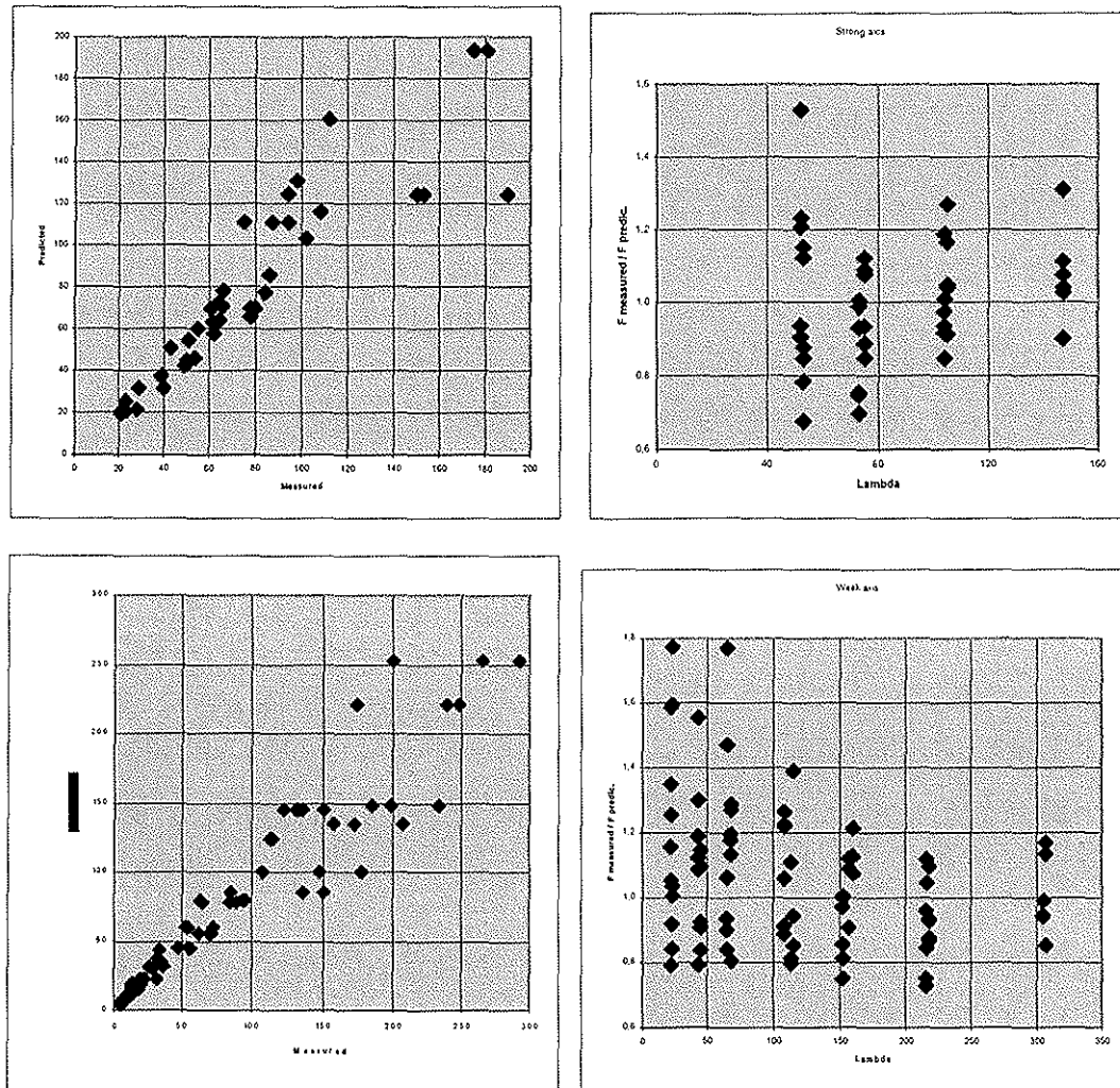
Figure 5.1 Measured versus predicted mean load-carrying capacity, and the ratio between these F_{\text{measure}}/F_{\text{predic.mean}} versus the geometric slenderness ratio for a column deflecting partly in the strong direction, partly in the weak direction. Mean values are calculated from the characteristic ones.
