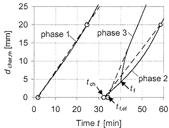
Figure 12 – Modelling of charring depth by linearization at different charring phases 1, 2 and 3
