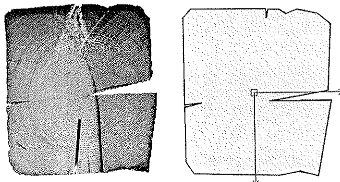
Figure 1-2 Typical cross-section of test specimen
