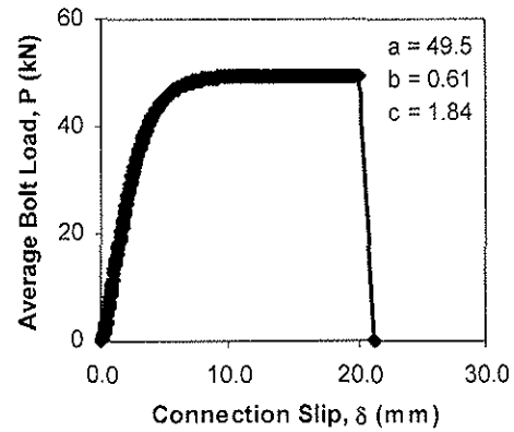
Figure 2 – Single 19.1 mm Bolt Load-Slip Curve in 80 mm S-P Glulam
