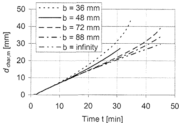
Figure 15 – Effect of flange width on charring depth in the middle of the flange (charring phase 1)
