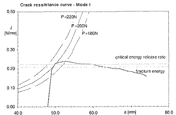
Fig. 2: Crack resistance curve for mode I with the specific energy levels, RL-crack system
