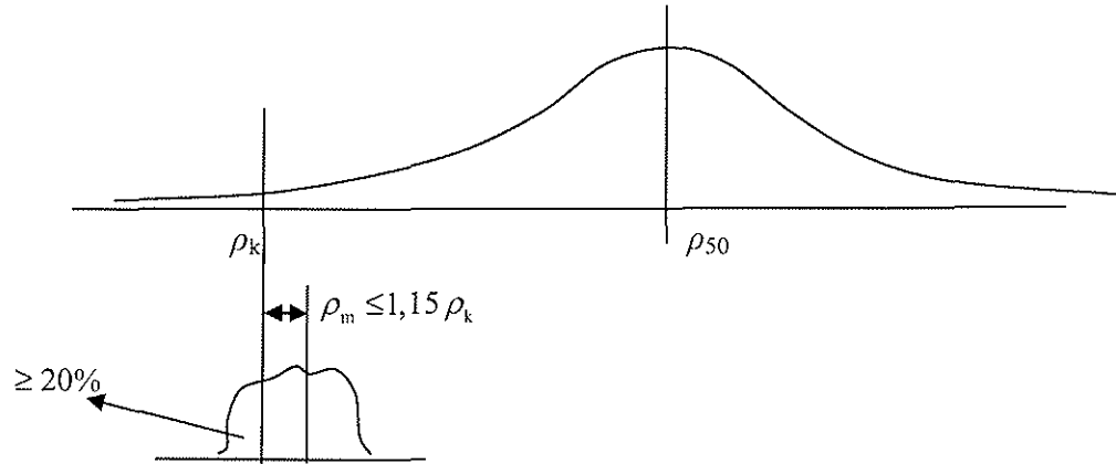
Figure 1: Graphical representation of the density requirements in method 1
