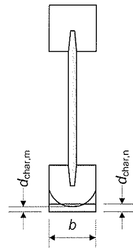
Figure 2 – Determination of the notional (equivalent) charring depth
