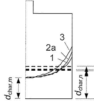
Figure 18 – Real and notional charring depths in flange for charring phases 1 (curve 1), 2 (curve 3) and 3 (curve 2a); for curve numbering see Table 1
