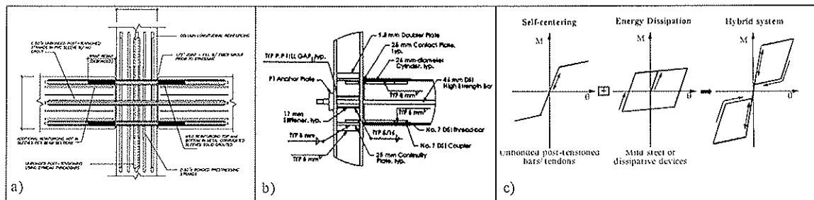
Figure 2. Hybrid solutions: a) for precast concrete frame systems (PRESSSS program, Priestley et al., 1999); b) for steel moment resisting frames (Post-Tensioned Energy Dissipation, PTED, Christopoulos et al. 2002b); c) idealised flag shape hysteresis loop.
