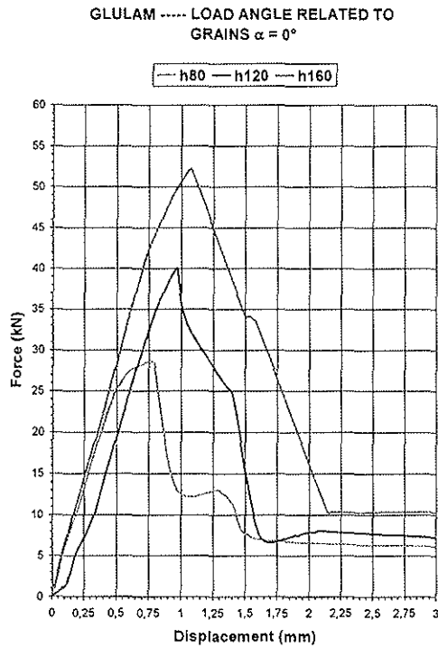
(a) Test Load Angle \alpha = 0^\circ
