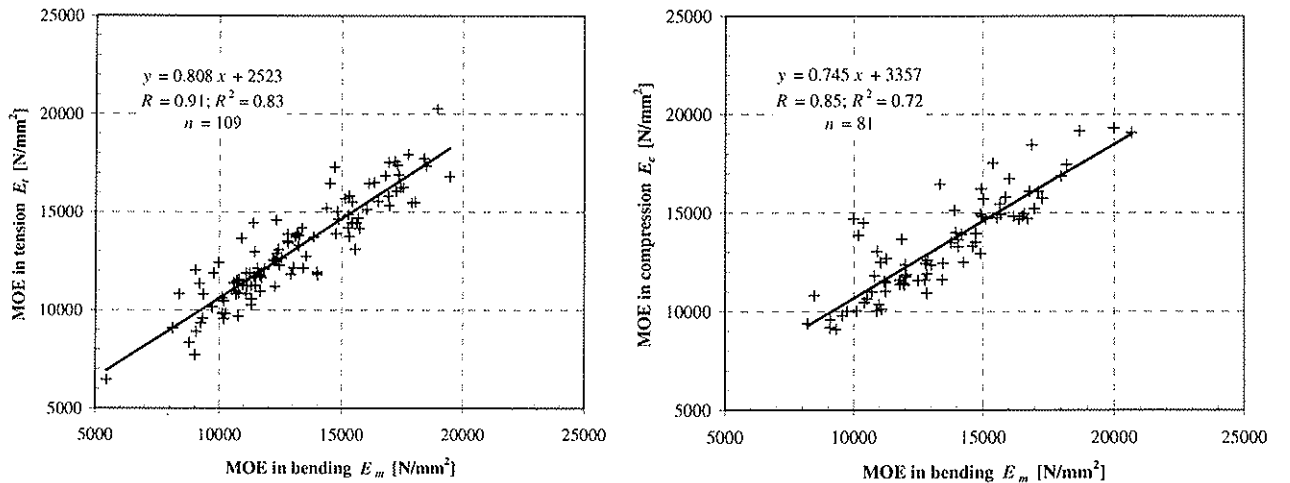
Fig. 10: Flexural MOE E_m versus tensile MOE E_t (left) and versus MOE in compression E_c (right) for Swiss grown Spruce structural timber with cross section 80/160 mm.
