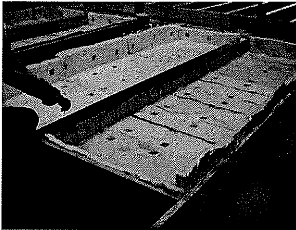
Figure 1. An FRP beam positioned in the test element
