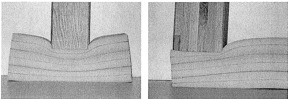
Fig. 2: Illustration of the supporting effect of wood fibers beside the direct loaded area by means of a loaded cellular material
