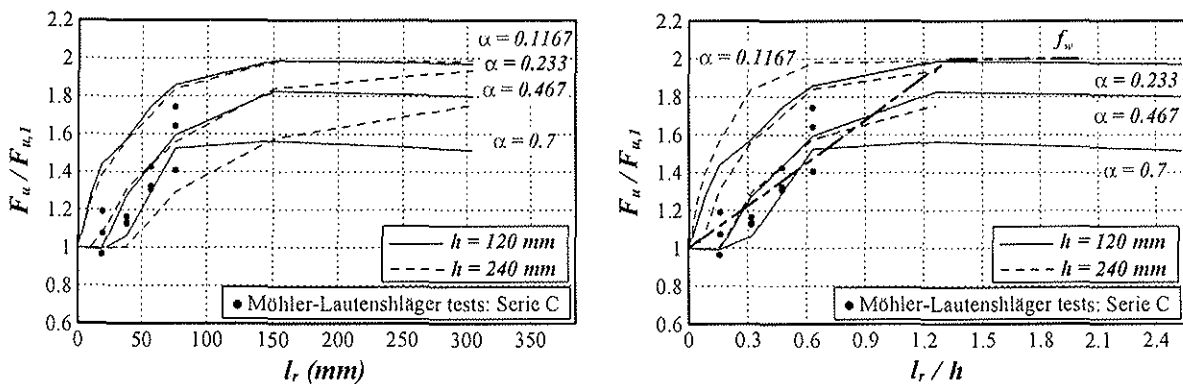
Figure 9 – Strength increase of specimens with 1 row of 2 fasteners as a function of the connection width l_f (left) and the ratio l_f/h (right).
