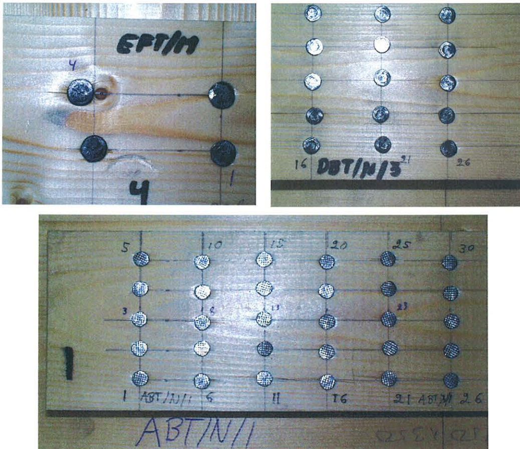
Figure 4 Examples on the biggest cracks of the nailing test specimens.
