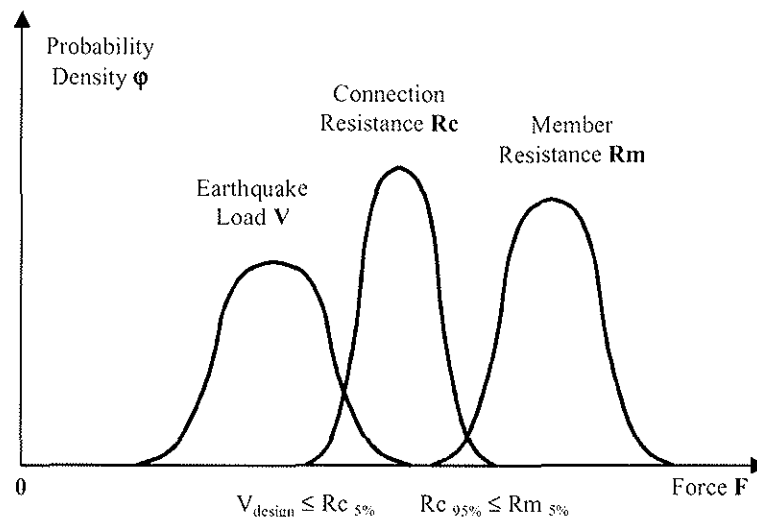
Figure 5. Graphical presentation of the logic behind the capacity design procedures
