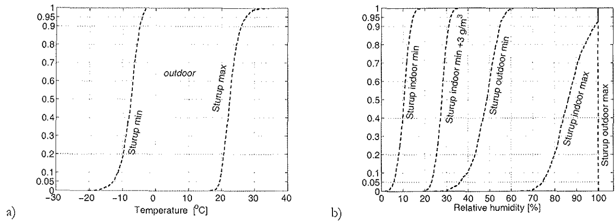
Fig. 4. Cumulative distribution functions (CDF) of annual minimum and maximum of temperature and relative humidity for Sturup. The added vapour concentration due to indoor moisture production is set to 3 \text{ g/m}^3 .
