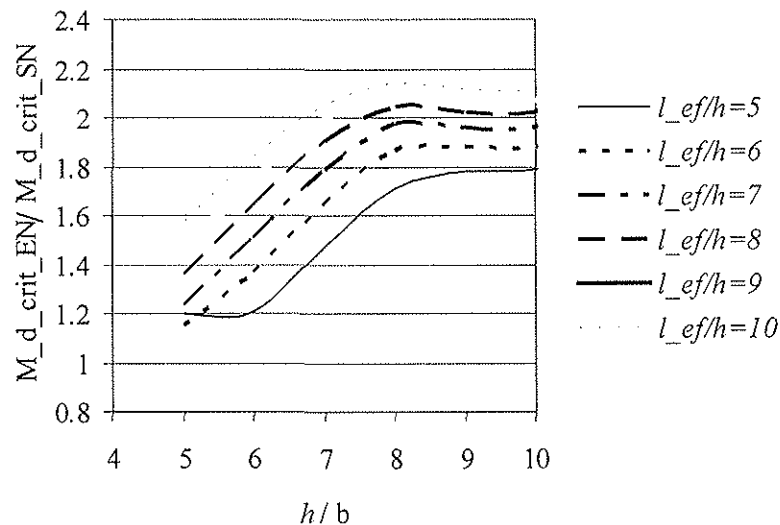
Fig. 3.3 Ratios of critical bending moments calculated according Eurocode 5 and SNIIP for different sizes of glulam beams
