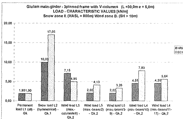
Fig. 11. A comparison of the results of characteristic load values calculation in accordance with the different standards. Estimating for snow zone II and wind zone B
