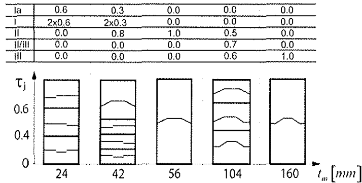
Figure 5 The componental (failure mode) sensitivities \tau_j for different middle member thickness.
