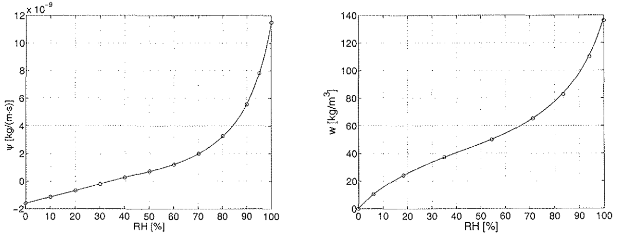
Fig. 3. Relations between RH, moisture content and the Kirchhoff potential for spruce in the tangential direction. Circles ('o') represent digitized points from hardcopy figures; lines are fitted polynomial functions.
