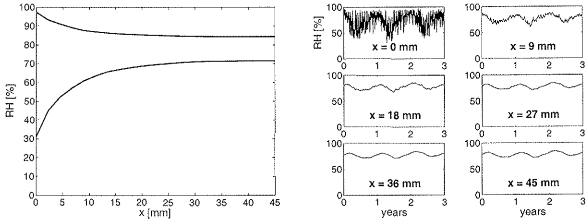
Fig. 6. Results from penetration depth calculations based on a 3 year long simulation sequence recorded in Stockholm (1961-1963). The left plot shows the extremes of the varying moisture profile, and the right plot shows the variation in time at different positions in the cross-section (position 'x' refers to the lower insulated boundary line shown in Fig. 2, i.e. x = 0 is in the lower left corner of the shaded quarter).
