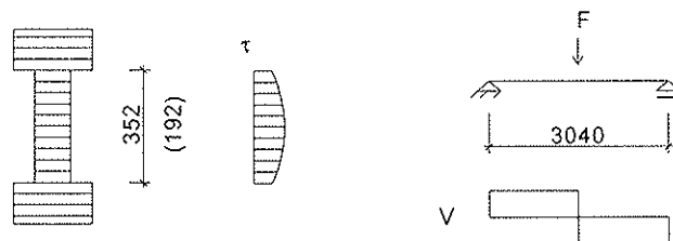
Fig. 2.3: Test configuration of Schickhofer [2]
