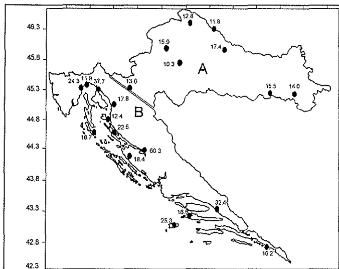
Fig. 7. A new wind map of Croatia (see zone B) in accordance with EC1
