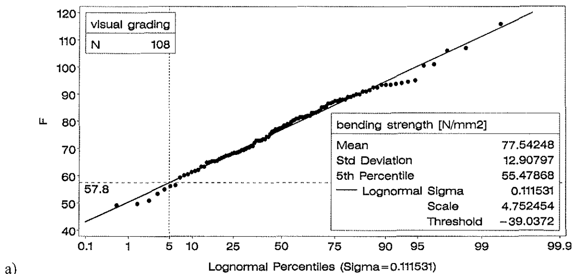
Fig. 4 Experimental data versus fitted lognormal density function; visual grading (a)
