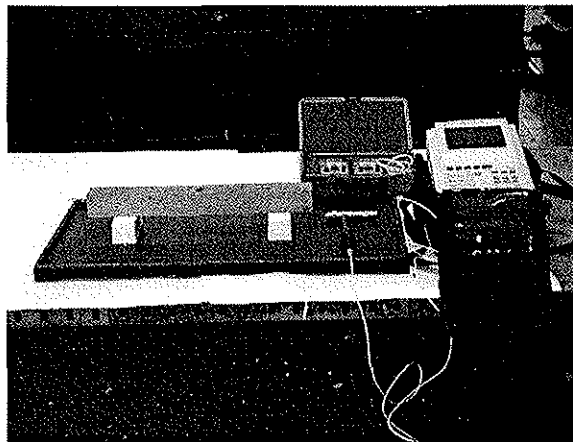
Fig 1: Determination of MOE by spectral analyser.
