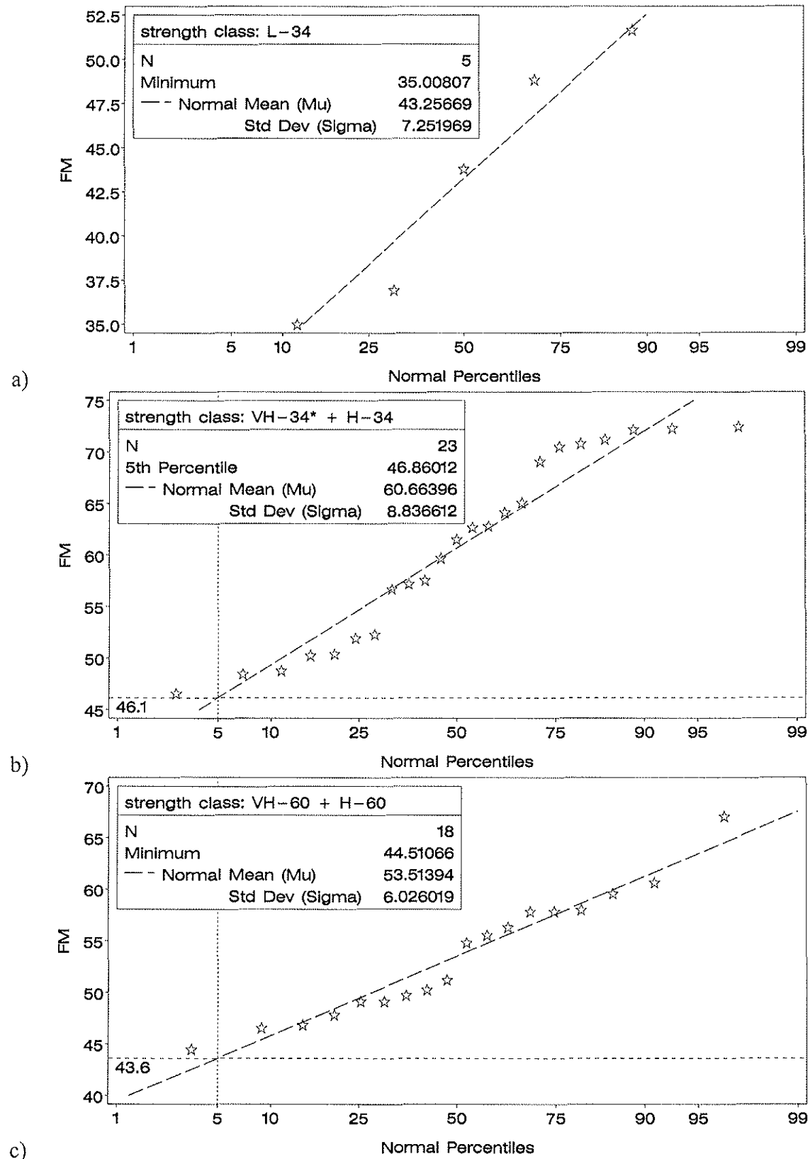
Fig. 2 experimental data versus fitted normal density function; strength class L-34 (a), VH-34 + H-34 (b) and VH-60 + H-60 (c) *A poorly manufactured finger joint in the outermost lamella caused a strength value of 32,7 N/mm 2 . Hence this value is disregarded.
