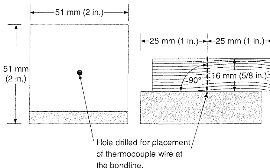
Figure 3. Top view (left) and side view (right) of drilled hole for thermocouple placement
