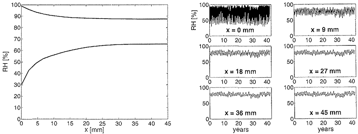
Fig. 7. Results from penetration depth calculations based on a 43 year long simulation sequence recorded in Stockholm (1961-2003). The left plot shows the extremes of the varying moisture profile, and the right plot shows the variation in time at different positions in the cross-section (position 'x' refers to the lower insulated boundary line shown in Fig. 2, i.e. x = 0 is in the lower left corner of the shaded quarter).
