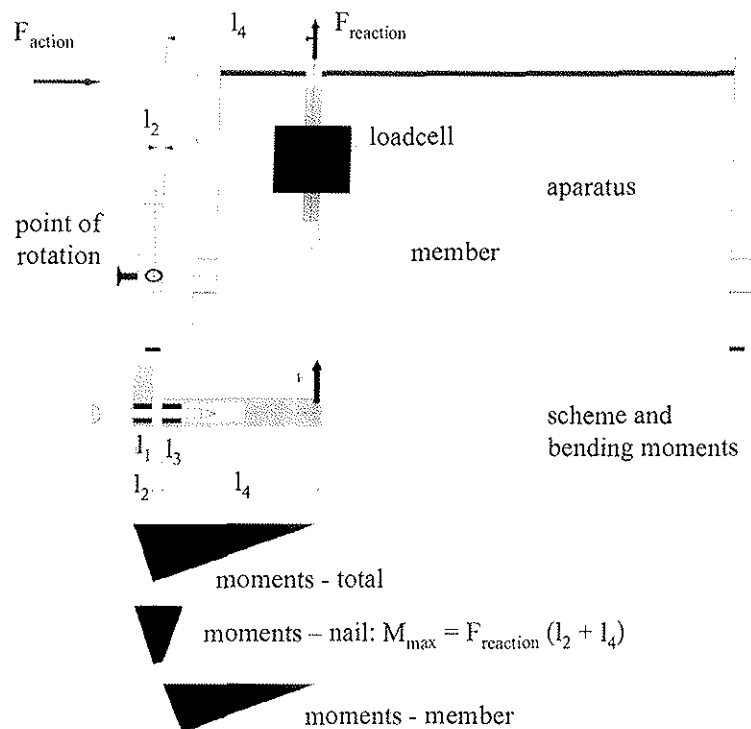
Figure 6: Nail bending apparatus. Remark: The shear force in the fasteners equals F_{\text{reaction}} . The (axial) tensile forces in the fastener are avoided.
