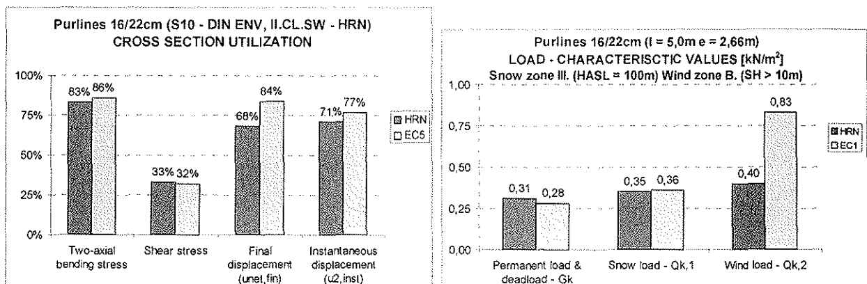
Fig. 8. Purlins of the glulam structure - snow zone III, wind zone B A comparison of the results of cross section utilisation and loads
