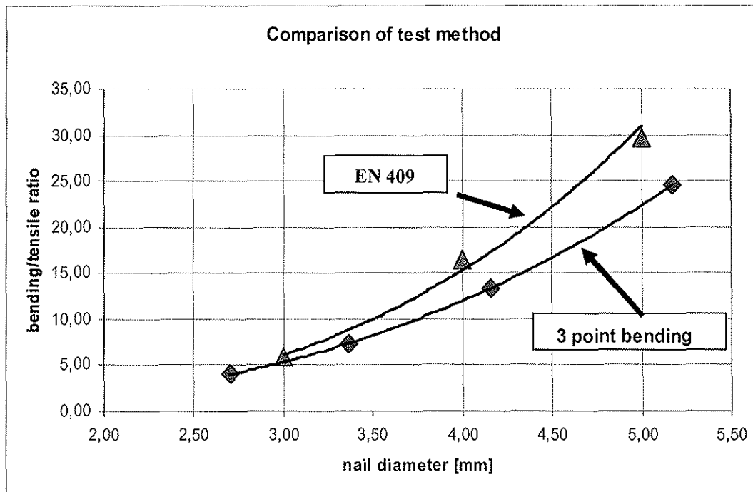
Figure 11: Comparing the EN409 method with the three point bending test. The latter is performed without correction of the bending moment for the rotation of the nail axes.
