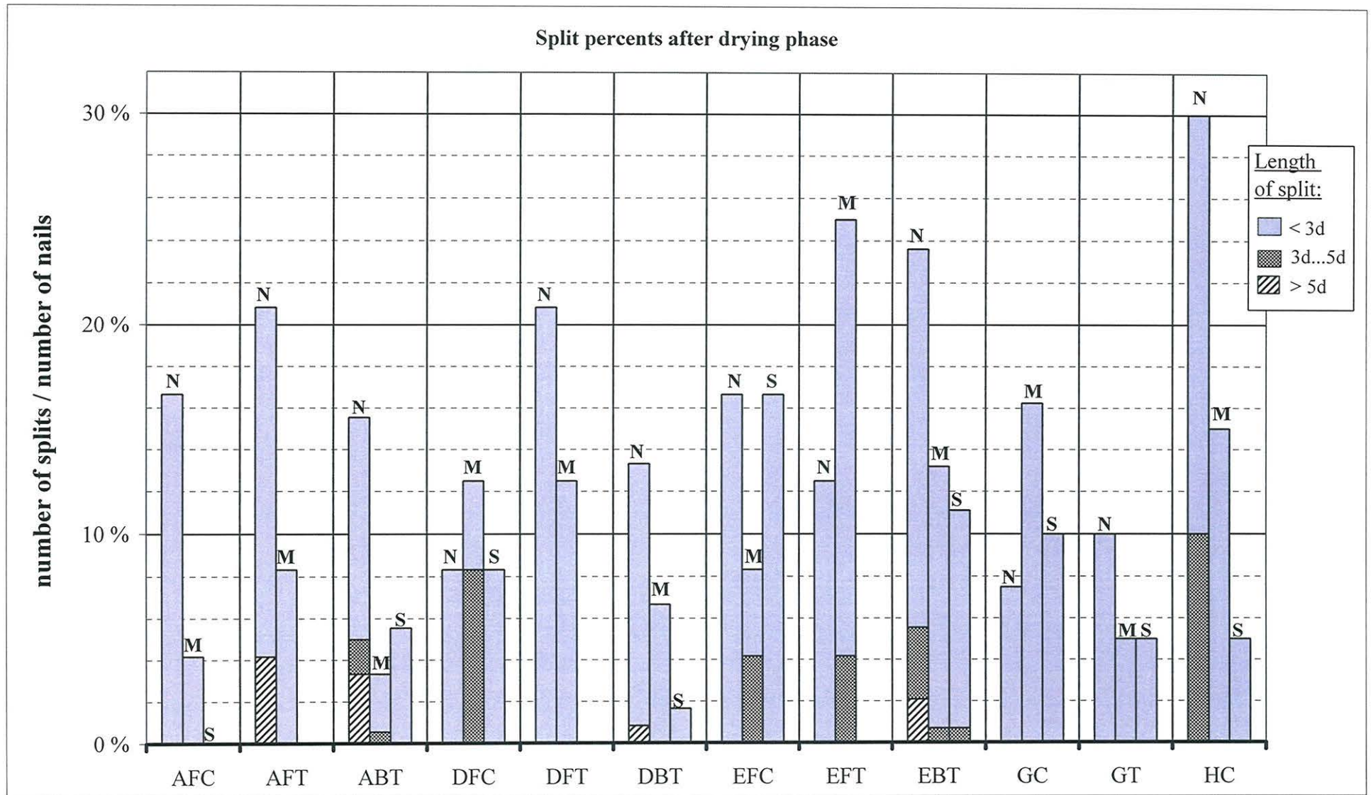
APPENDIX: Summary of the cracking results of splitting test specimens measured after drying phase.
