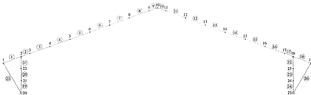
Fig. 6. Model of the main girder of a timber structure used for its computed design
