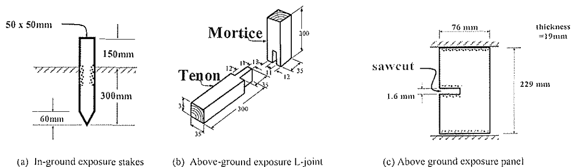
Figure 5. Examples of standard test specimens for assessing the durability of timber.
