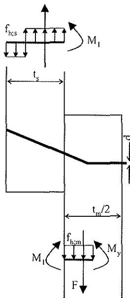
Figure 1: Failure mechanism leading to equations (2) and (3)
