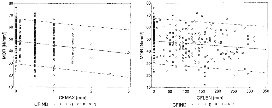
Fig. 6. Effect of the axial 'width' (CFMAX, left) and the circumferential length (CFLEN, right) of the largest CF on the modulus of rupture (MOR). The solid line indicates the linear regression line, the dotted lines enclose the 90% confidence band for individual predicted values for the beams with CF.
