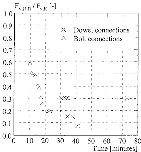
Figure 8 Load ratio versus time to failure for the carried out connections with dowels in comparison to connections with bolts
