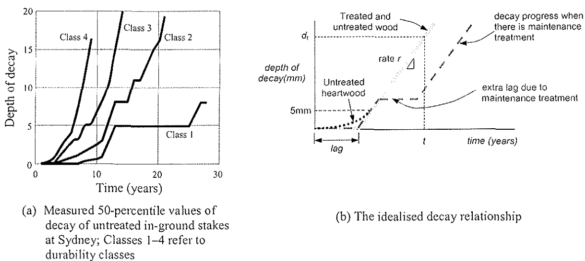
Figure 6. Decay of in-ground stakes
