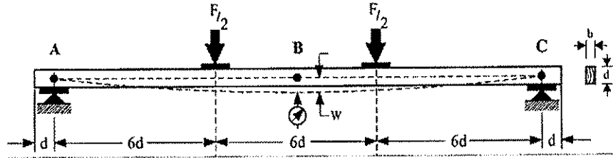
Figure 1. Bending test arrangement according to ISO/DIS 13910
