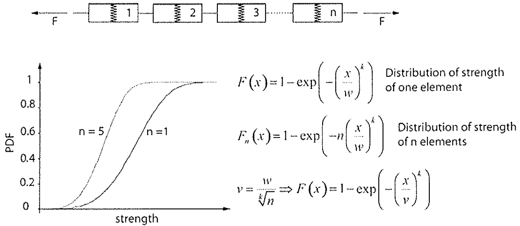
Fig. 7: Weibull's weakest link theory to model the strength probability distribution of a serial system of n identical brittle solids.
