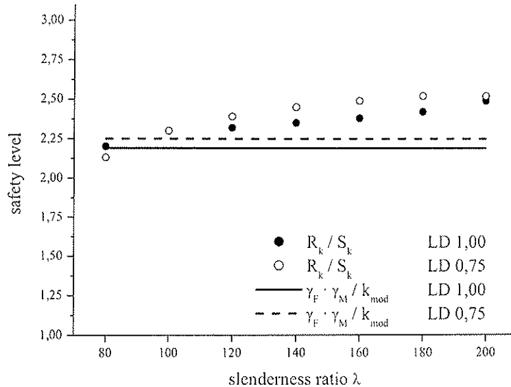
Fig. 7: Comparison between the safety levels (equation (1)) from the results of virtual experiments taking hygrothermal long-time effects into account with reference to DIN 1052 [1] –model column method (modifying factor k_{creep}^* )- with b/h = 16/16 cm in service class 2 (see [3])
