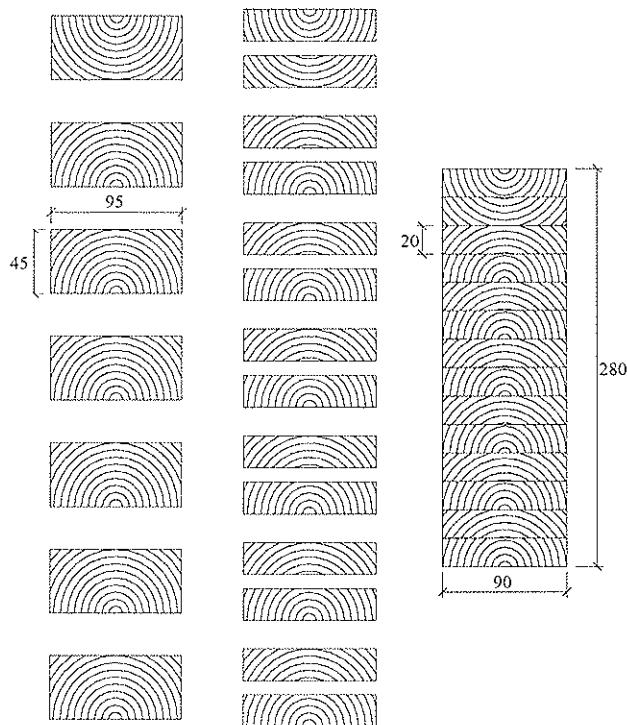
Fig. 2. Lamellae, sawing pattern and cross section.
