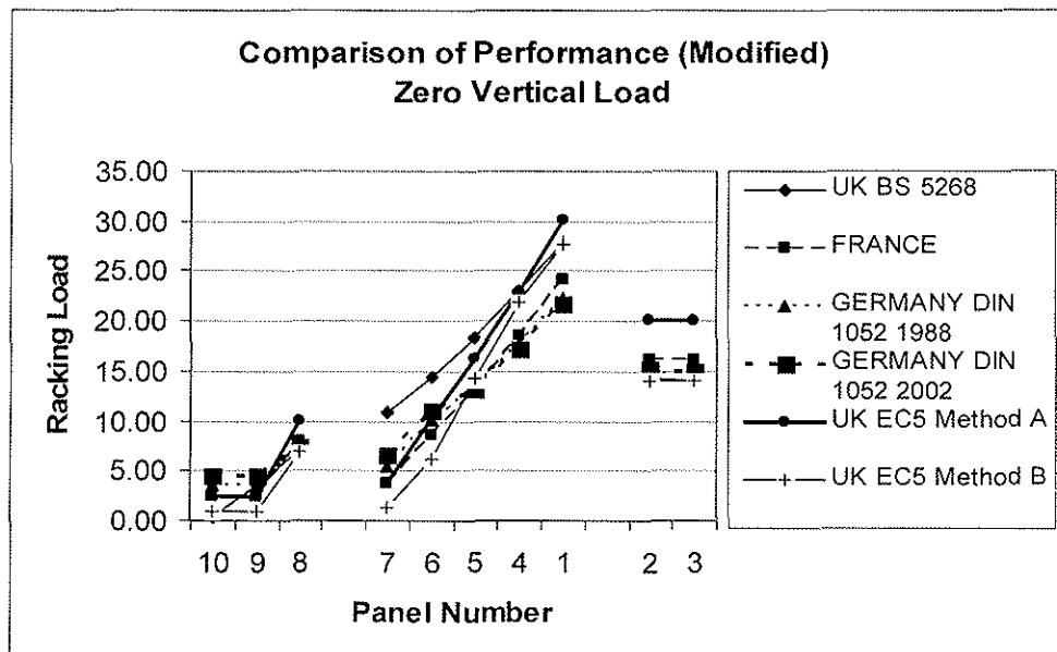
Figure 1: Comparison of Current Design Methods at Zero Vertical Load
