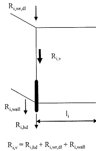
Figure 9.8 Vertical restraint R_{i,v}
