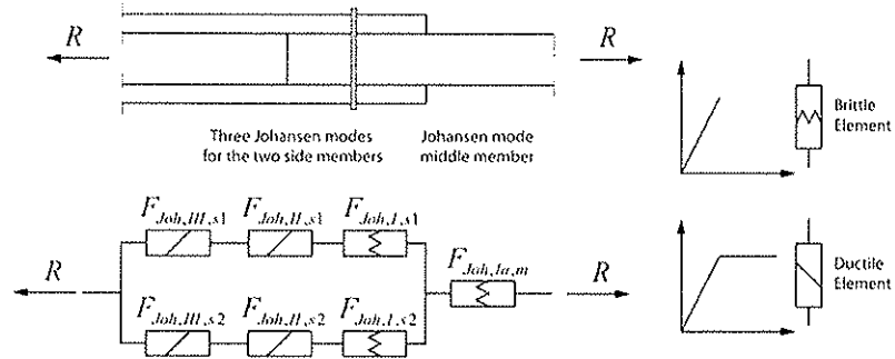
Figure 3 Interaction of failure modes
