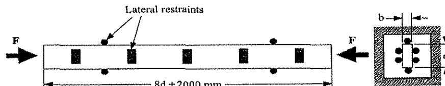
Figure 4. Configuration of compression test according to ISO/DIS 13910.
