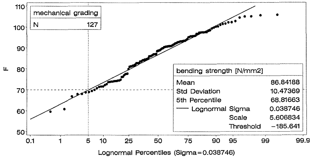
b) Fig. 4 (Continuation) experimental data versus fitted lognormal density function; mechanical grading (b)
