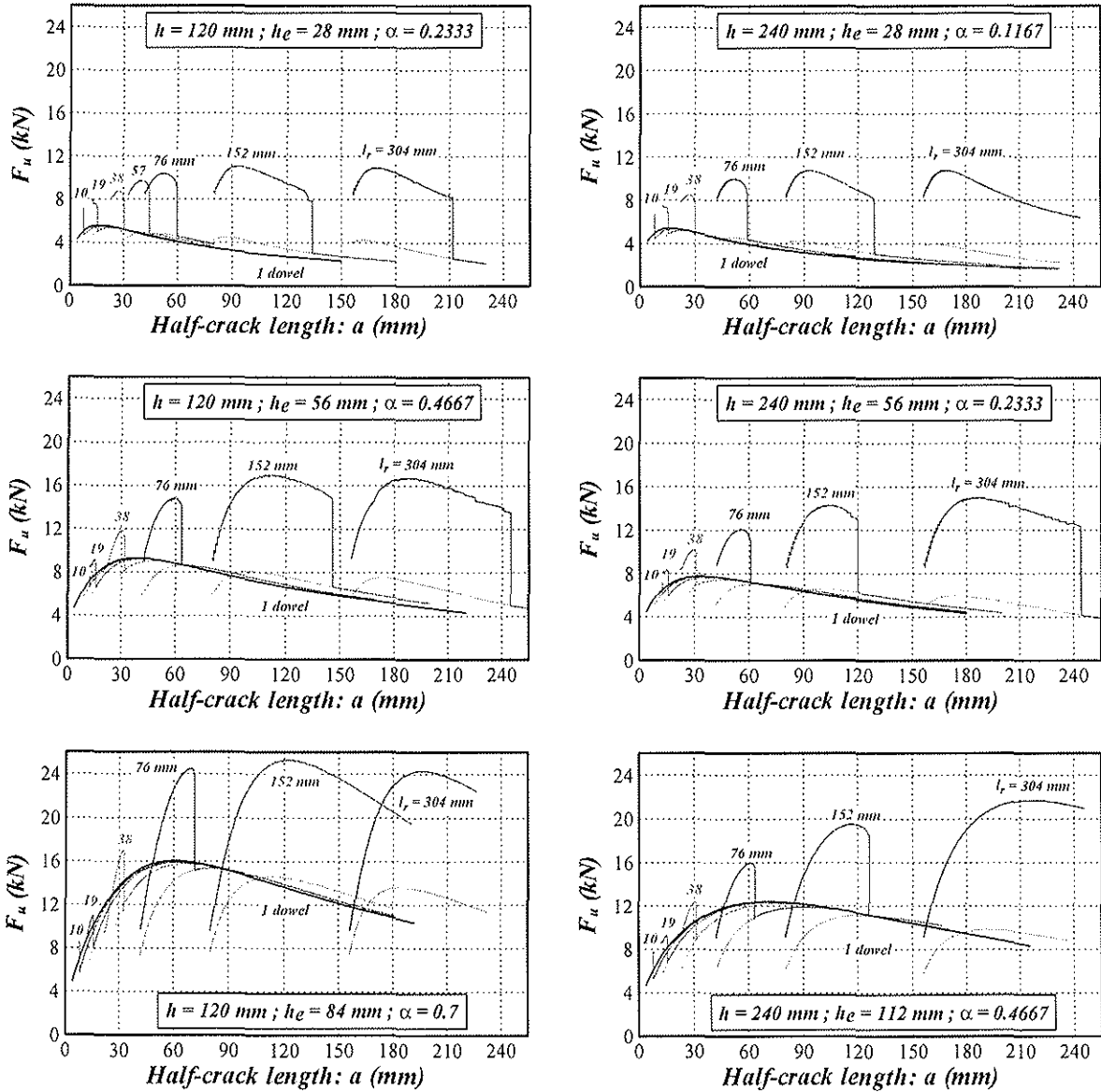
Figure 8 – Numerical failure splitting loads of beams loaded at mid-span by connections made with 2 fasteners at different spacing ( l_f ) versus half-crack length (half distance between furthest crack tips).
