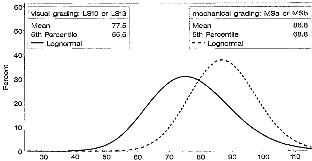
Fig. 5 lognormal density curve of finger joint bending strength (N/mm²); visual grading in comparison with mechanical grading
