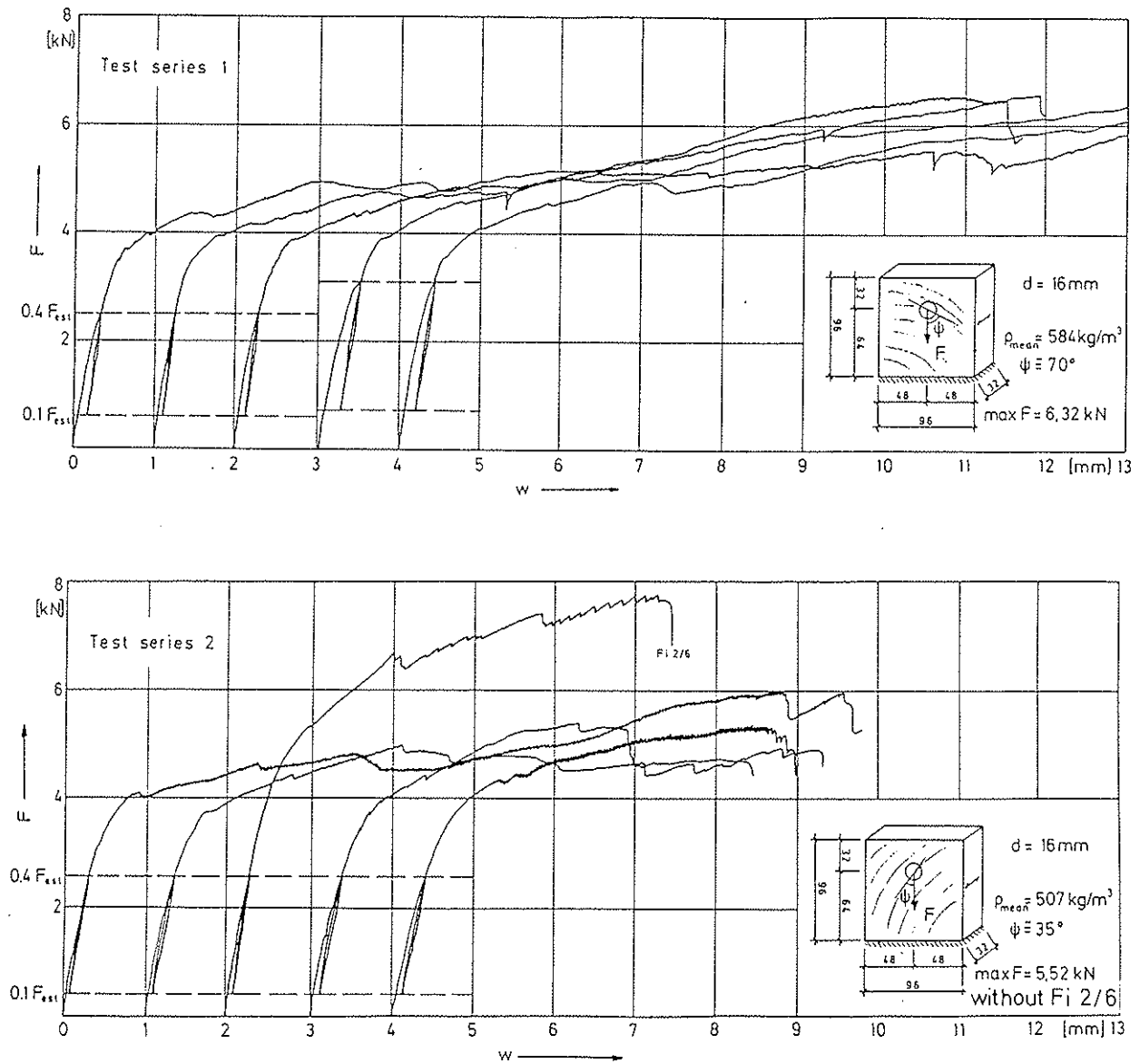
Fig.6: Load-deformation curve of specimens with a dowel-type fastener loaded in compression perpendicular to grain in a prebored hole parallel to grain
