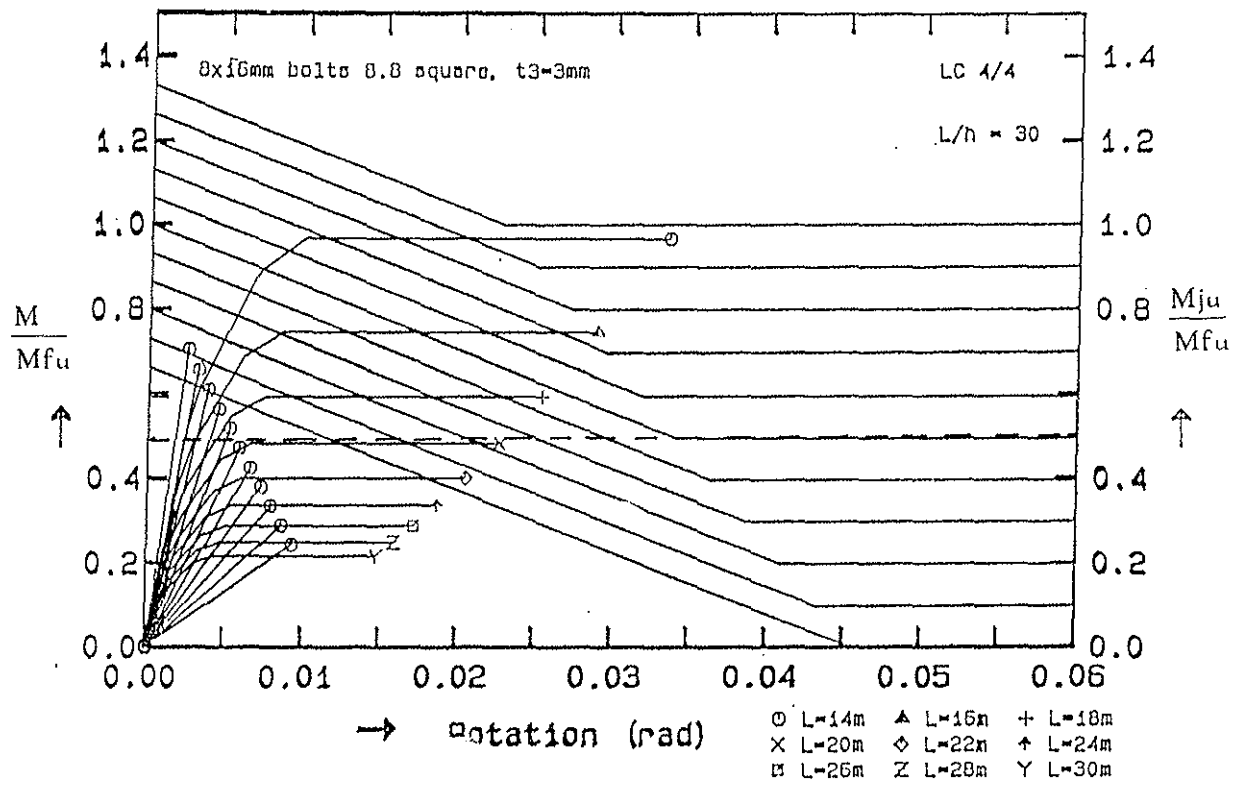
fig. 10: Combination of rotation requirements and moment-rotation curves of steel reinforced joints of fig. 9
