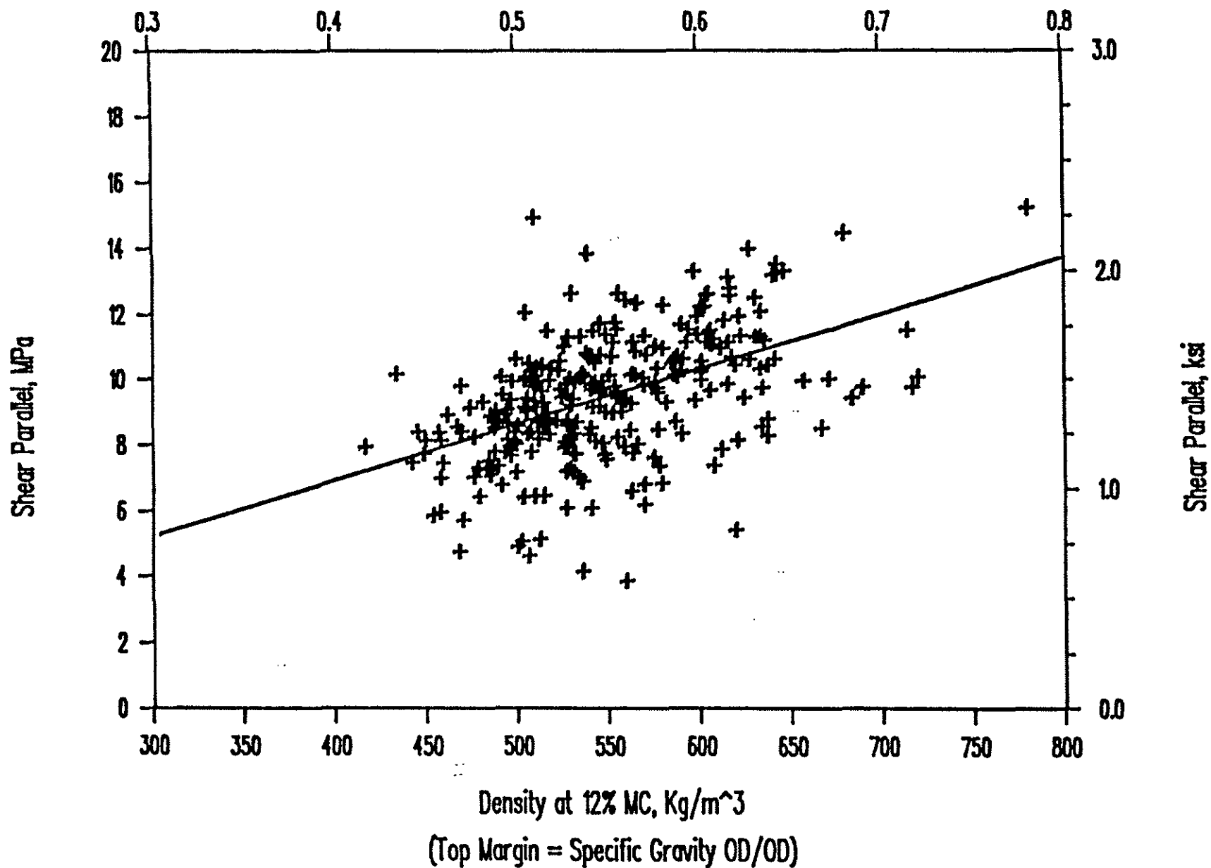
Figure 9.--Relationship between shear strength parallel to the grain and density for Southern Pine lumber at 12% moisture content.
