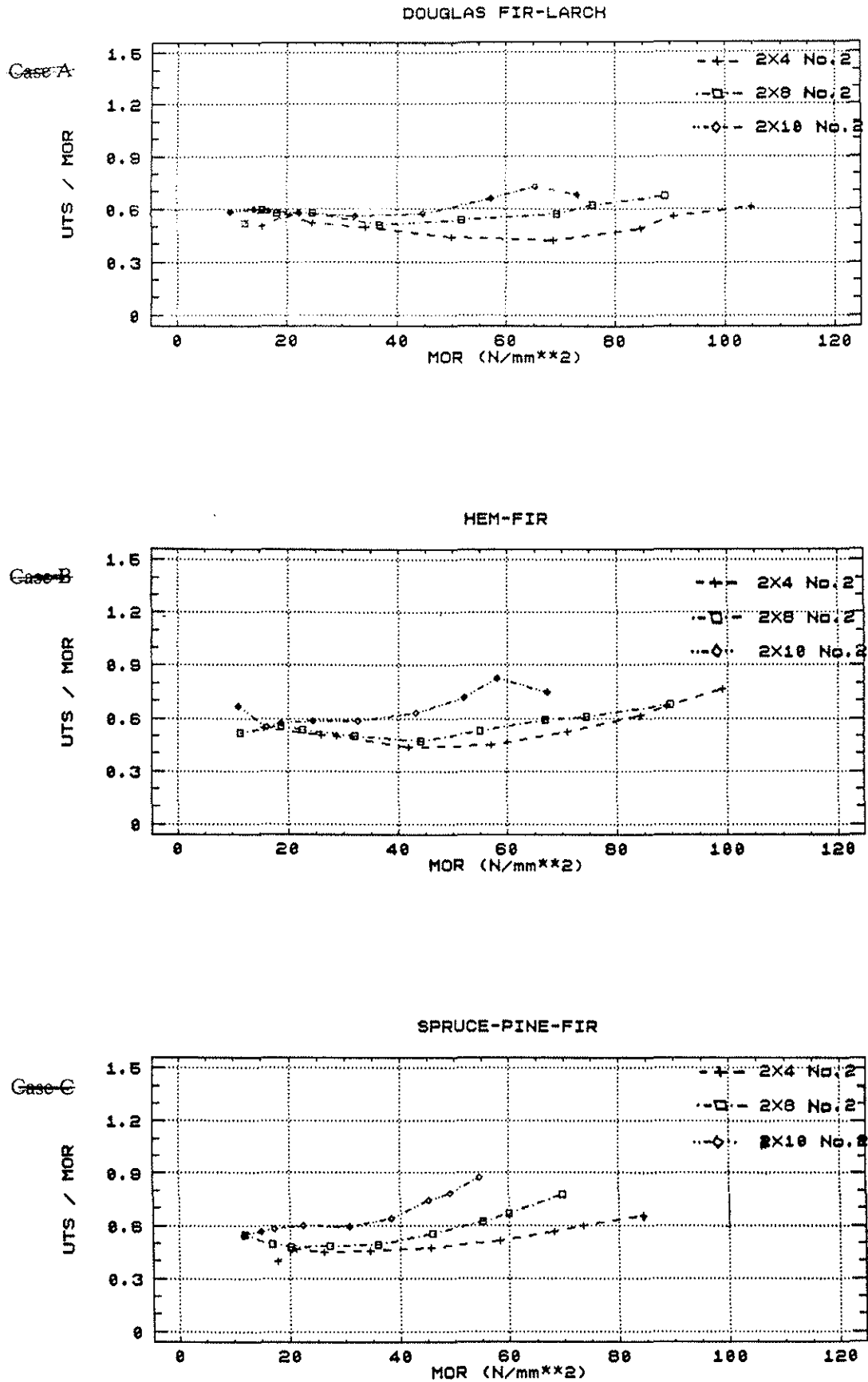
Figure 2. Tension/Bending Property Ratios for D Fir-L, Hem-Fir and S-P-F, No. 2 Grade.
