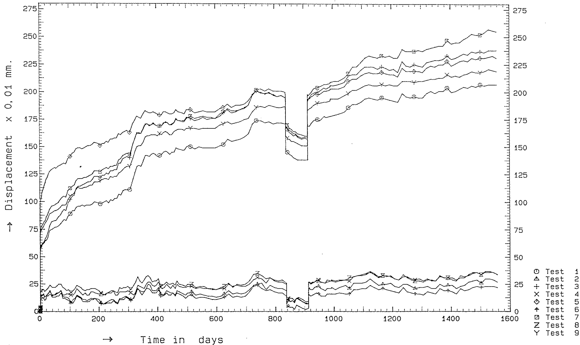
fig.3: Creep results of joints with shearplates and steelplate reinforced joints. The data of the reinforced joints is found at the bottom of the graph. During the first 2 years the load level was 40% afterwards 50%.
