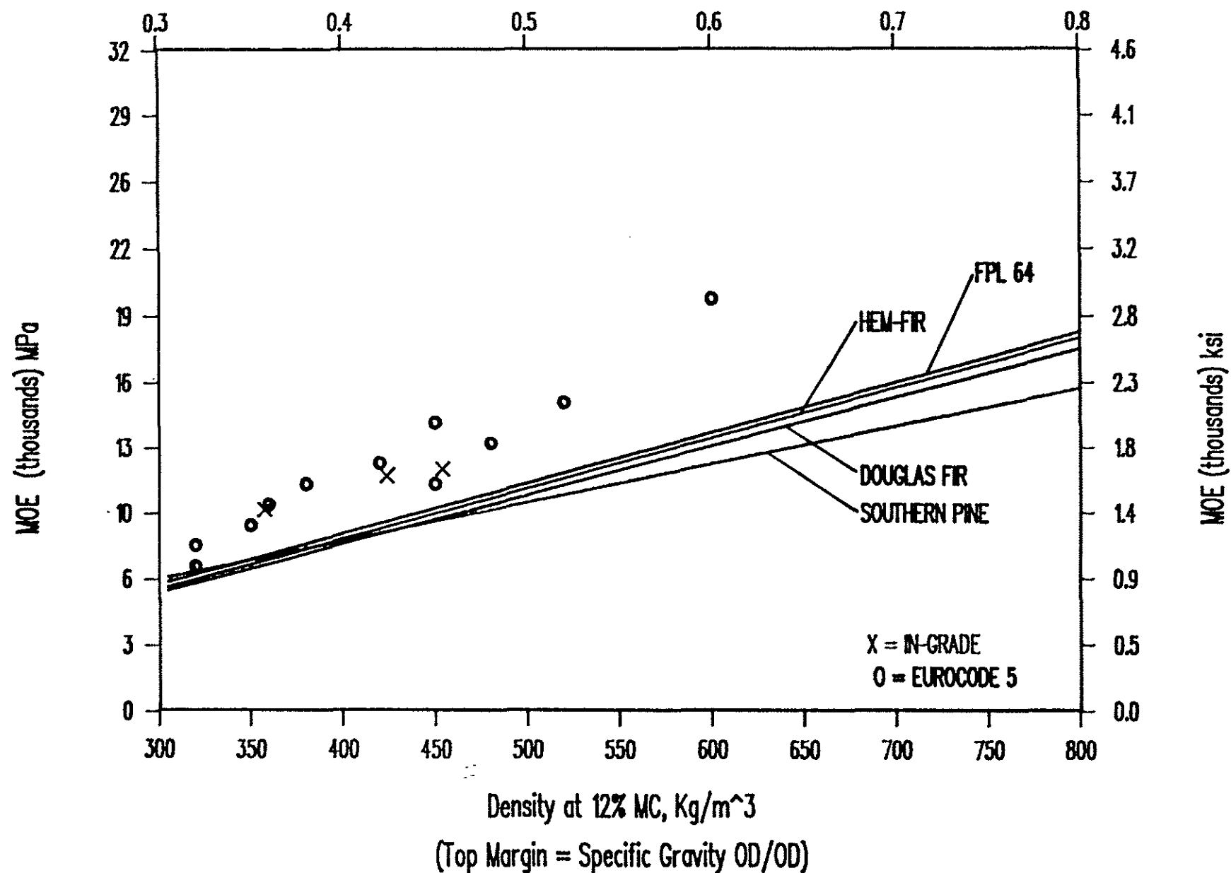
Figure 5.--Relationship between modulus of elasticity and density at 12% moisture content.
