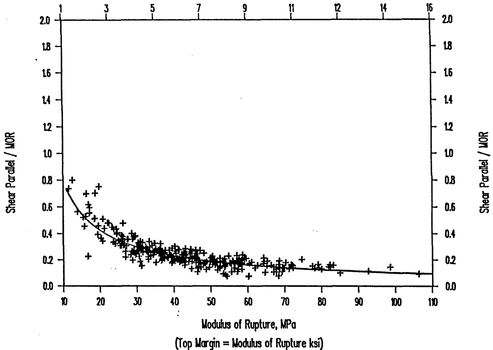
Figure 8.--Relationship between shear strength parallel to the grain and modulus of rupture for Southern Pine lumber at 12% moisture content.
