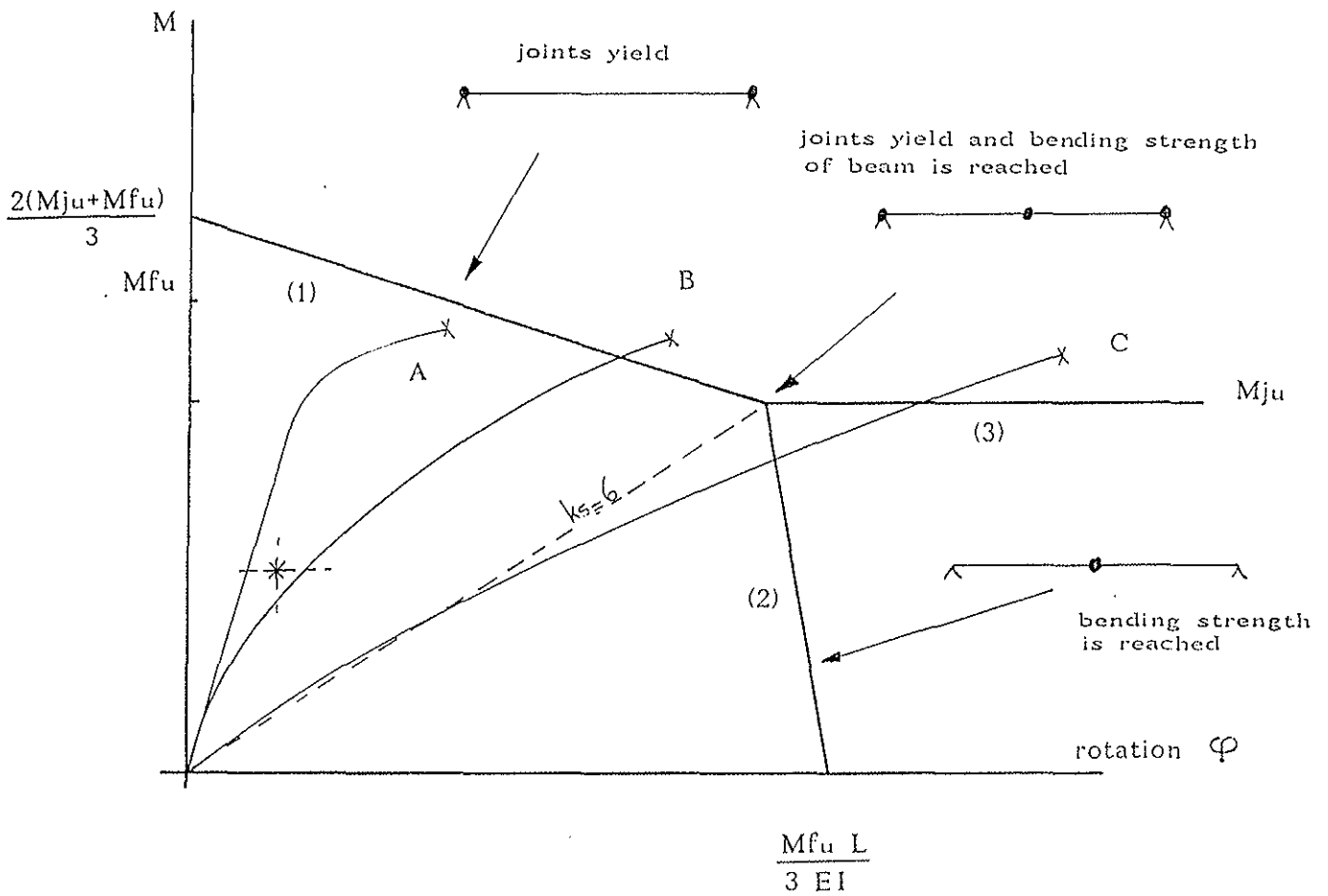
fig.3 : Requirements for rotation capacity
