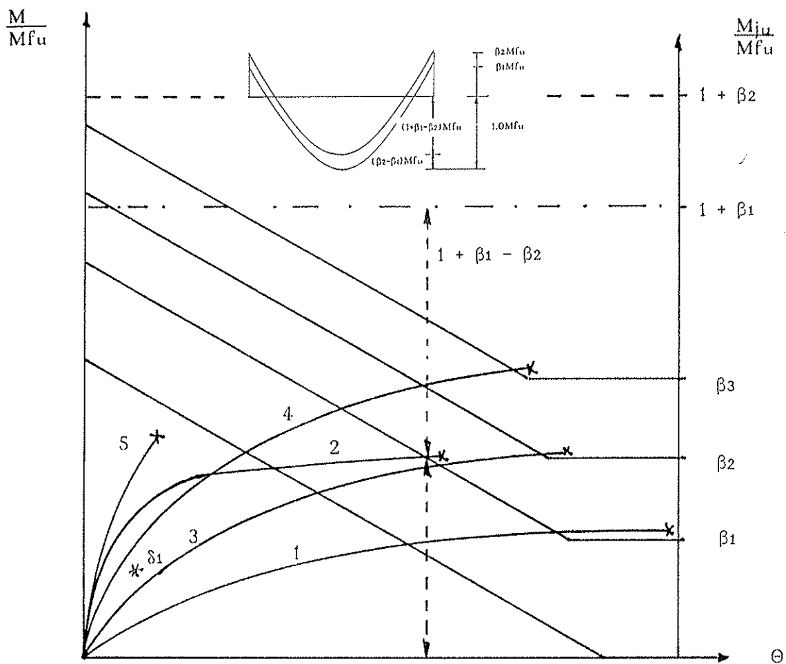
fig.7: Moment-rotation requirements combined with several moment-rotation curves.
