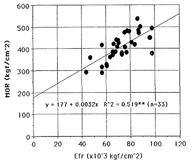
Figure 4. Relationship between E_{fr} and MOR
