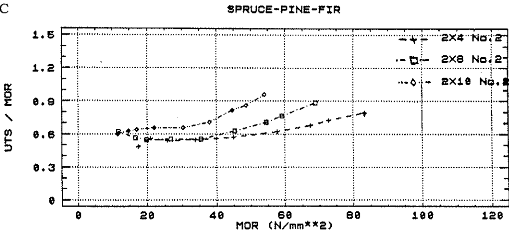
Figure 6. Tension/Bending Property Ratios for Case A, B, C Test Configurations - S-P-F, No. 2 Grade.
