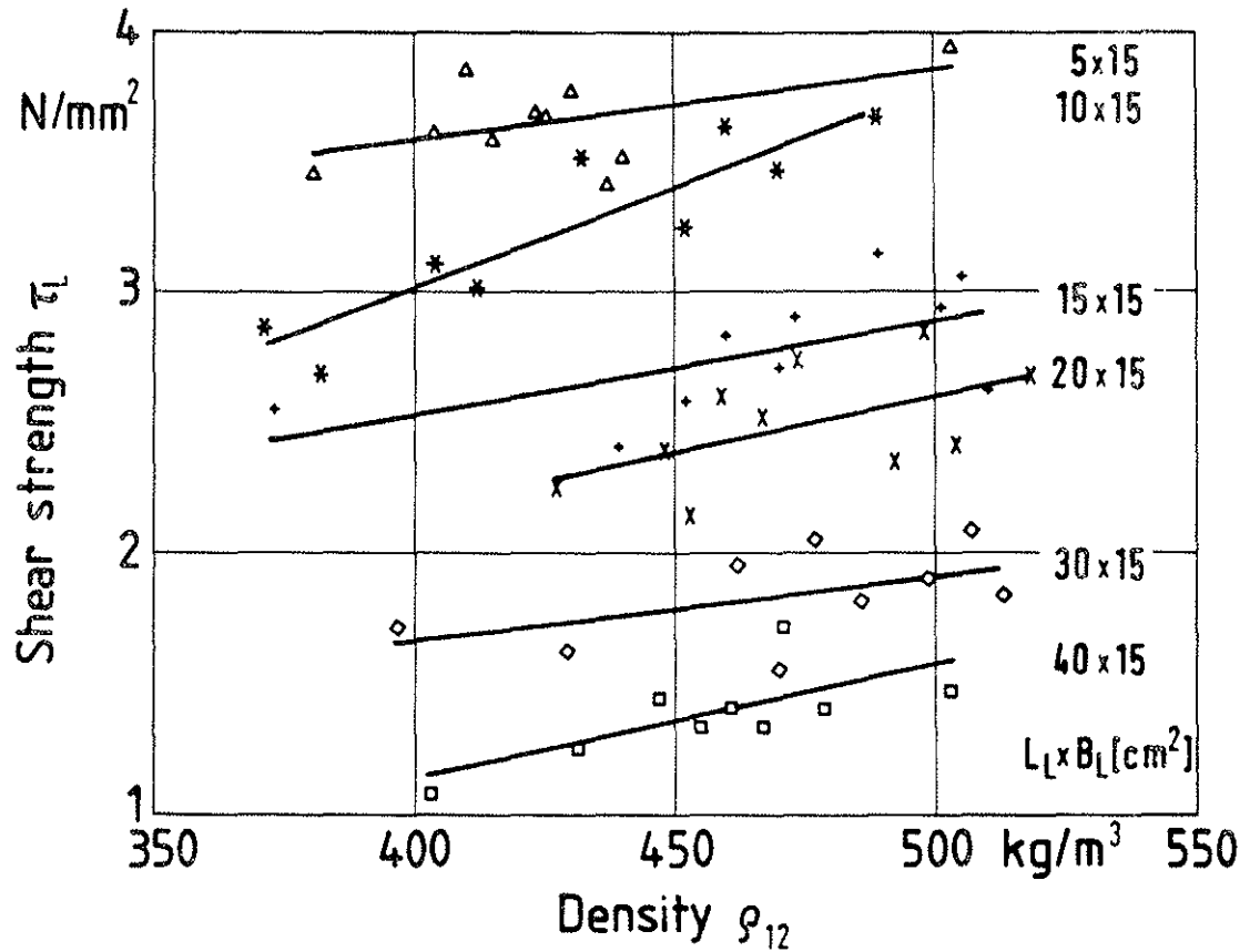
Figure 12: Effect of density \rho_{12} on shear strength \tau_L for different sizes of glued area ( A = L_L \cdot B_L , \alpha = 0^\circ , l_{e1} = 5 \text{ cm} )
