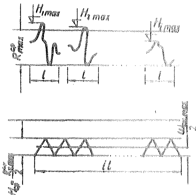
Figure 2. Irregularity of the plywood surface: a) actual profiles of the irregular surface of the plywood test specimen on l investigated sections with a basic length l; b) model of the profile of the investigated irregular plywood surface
