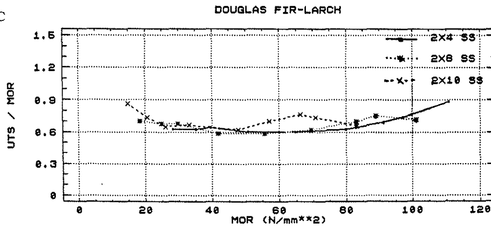
Figure 9. Tension/Bending Property Ratios for Case A, B, C Test Configurations - D Fir-L, Select Structural Grade.
