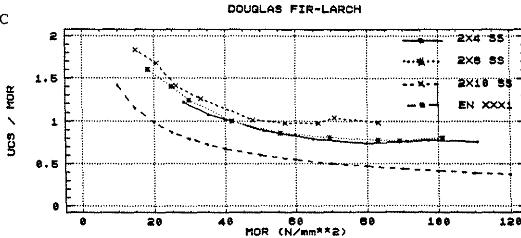
Figure 11. Compression/Bending Property Ratios for Case A, B, C Test Configurations - D Fir-L, Select Structural Grade.
