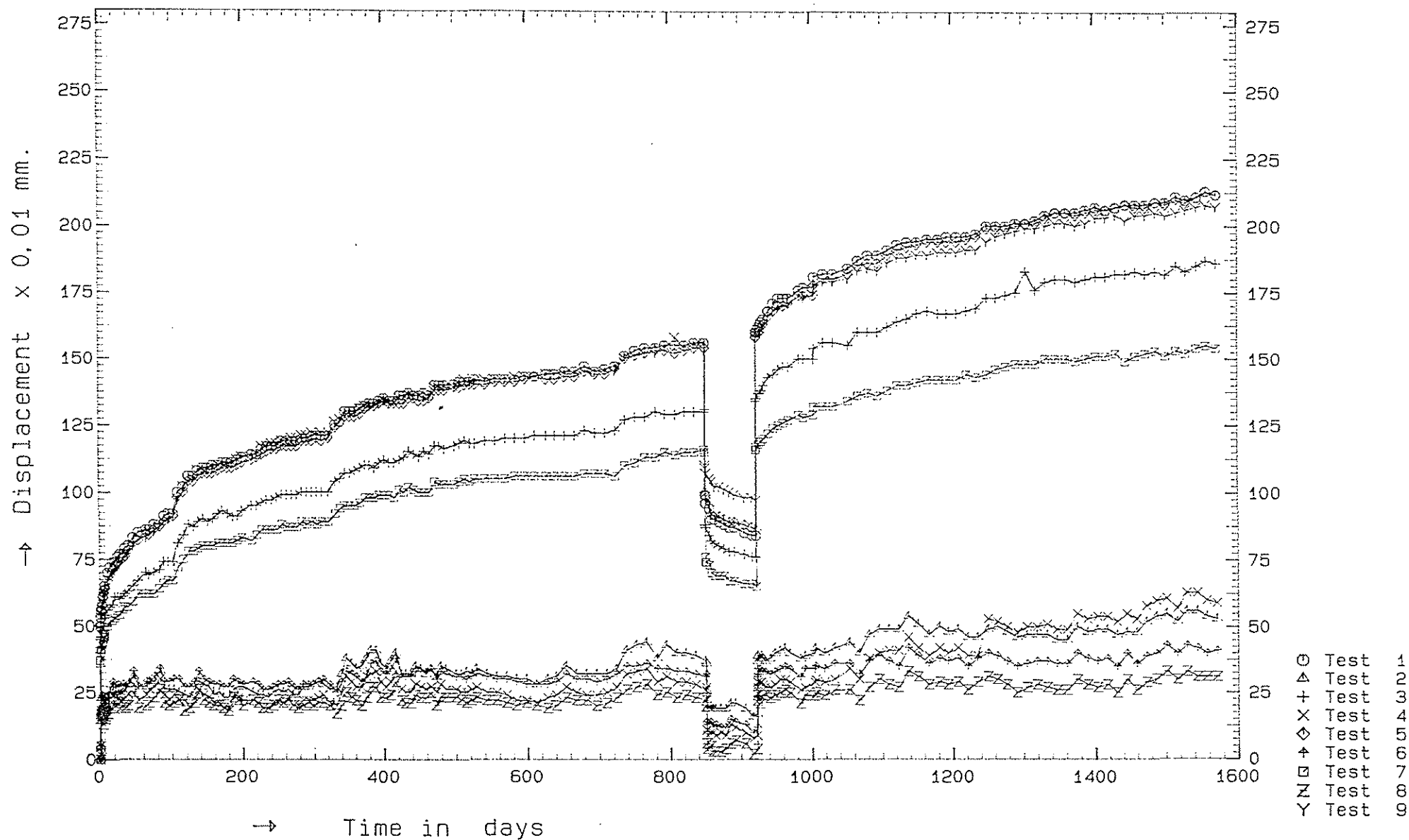
fig.3: Creep results of joints with nails and steelplate reinforced joints. The data of the reinforced joints is found at the bottom of the graph. During the first 2 years the load level was 40% afterwards 50%.
