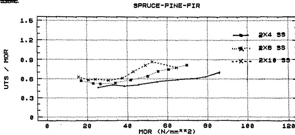
Figure 1. Tension/Bending Property Ratios for D Fir-L, Hem-Fir and S-P-F, Select Structural Grade.
