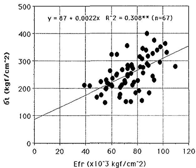
Figure 3. Relationship between E_{fr} and tensile strength ( \sigma_t )
