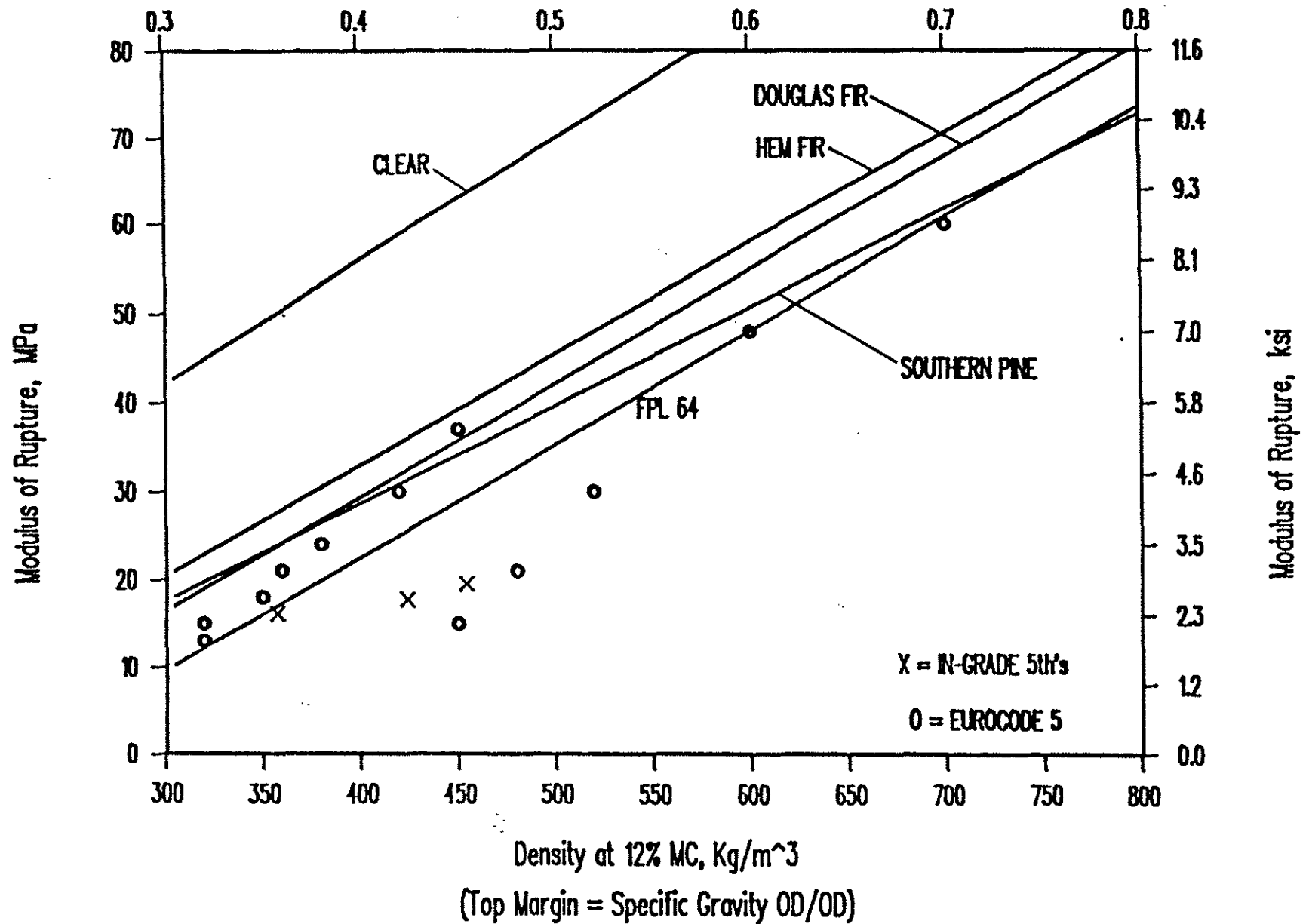
Figure 4.--Relationship between modulus of rupture and density at 12% moisture content.
