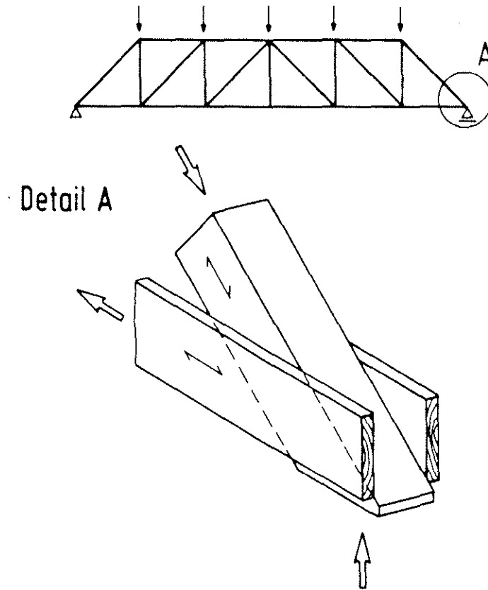
Figure 1: Truss (schematic). A: heel joint
