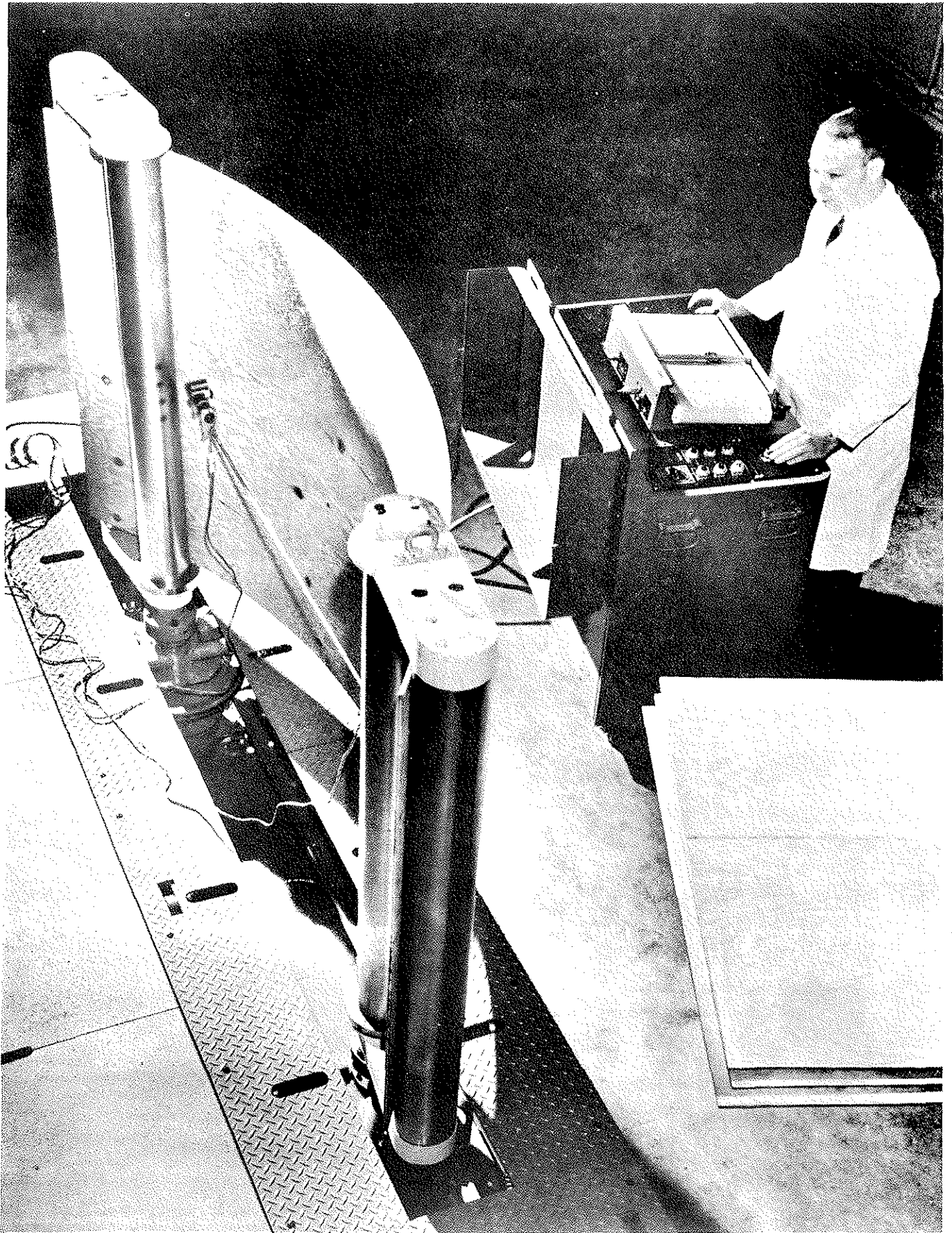
Bending test for stiffness and strength.
