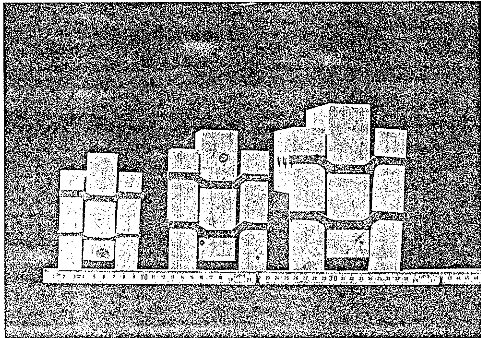
Fig. 4: Failure mode 4 with four bending failures of the dowels
