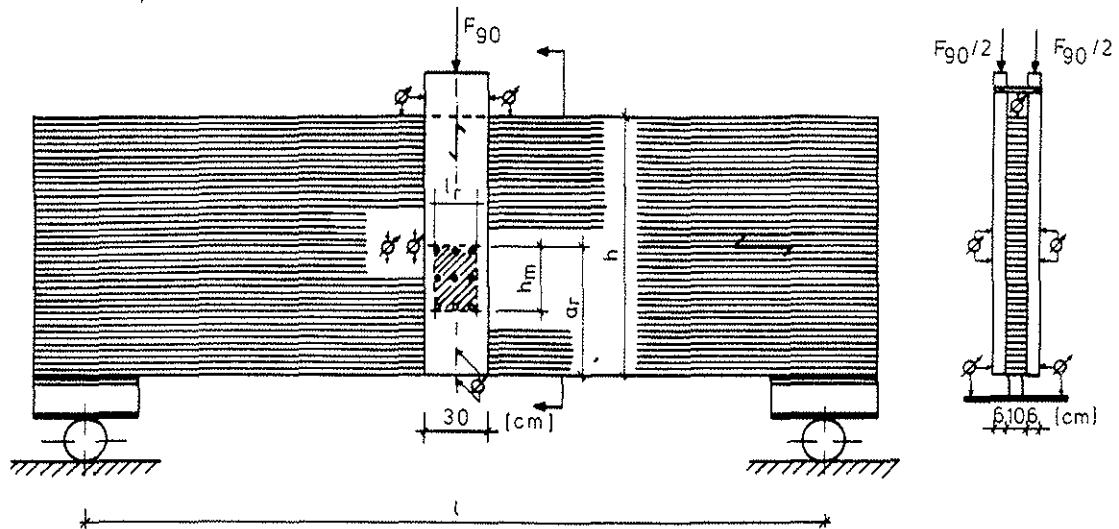
Fig. 2: Test set-up for testing joints loaded perpendicular to grain of glulam beams ( Möhler / Siebert [3] ).
