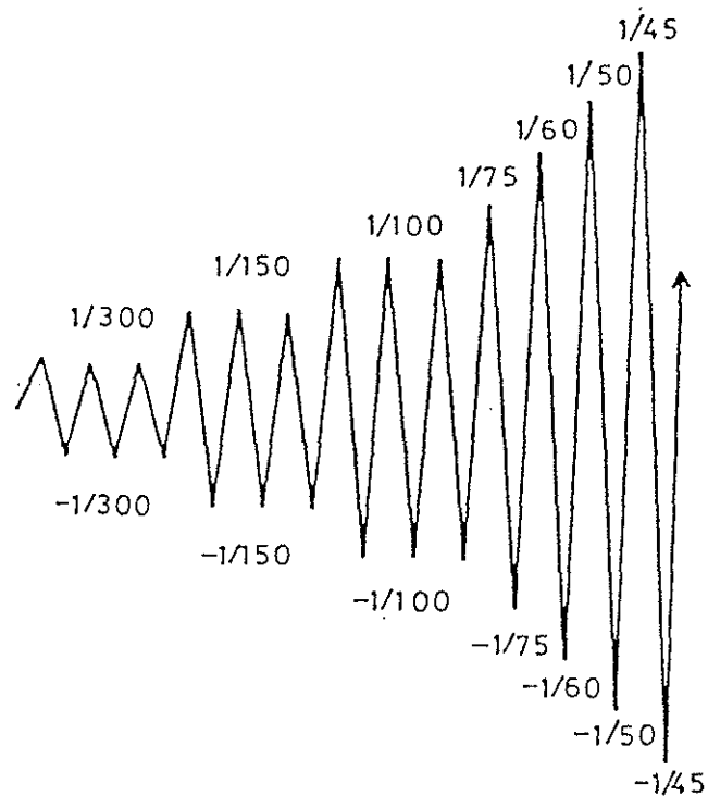
Fig.3 LOADING HISTORY (Values represent the ratio of the deflection to span)
