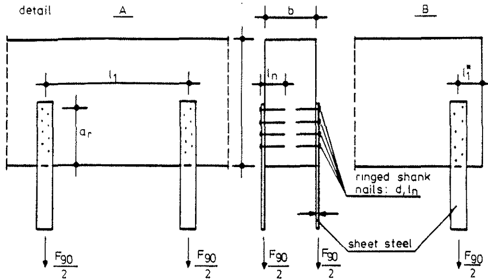
Fig. 3: Test set-up for steel-to-wood joints loaded perpendicular to grain (Ehlbeck / Görlacher [4]).
