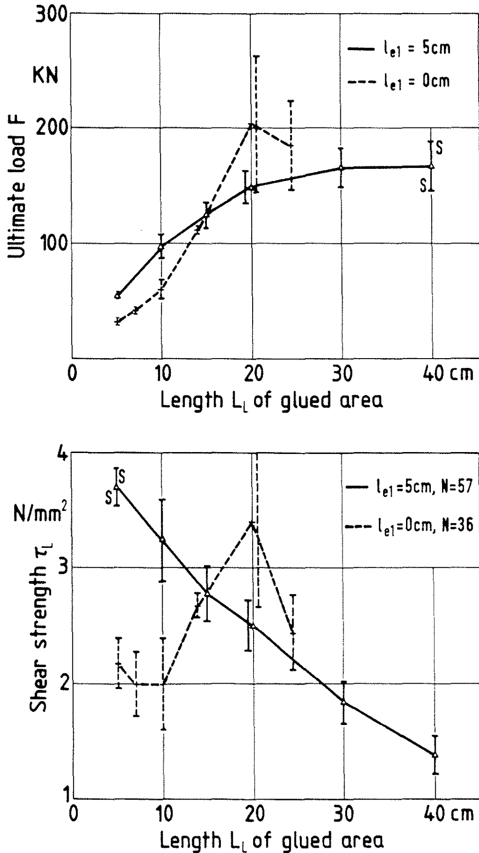
Figure 6: Effect of length L_L of glued area a) on ultimate load F and b) on shear strength for specimens without and with end distance ( l_{e1} = 0\text{ cm} , l_{e1} = 5\text{ cm} , \alpha = 0^\circ ) s = standard deviation
