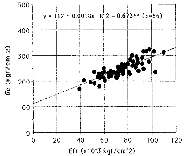
Figure 2. Relationship between E_{fr} and compressive strength ( \sigma_c )
