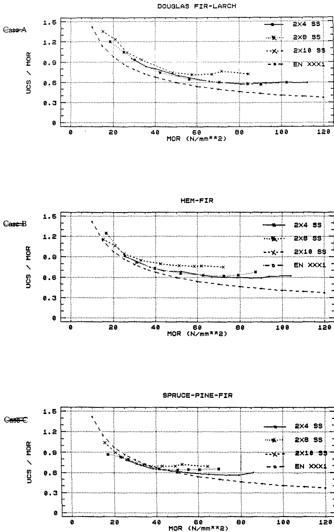
Figure 3. Compression/Bending Property Ratios for D Fir-L, Hem-Fir and S-P-F, Select Structural Grade.
