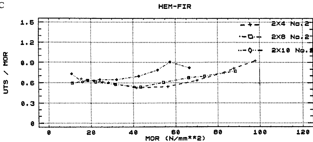
Figure 14. Tension/Bending Property Ratios for Case A, B, C Test Configurations - Hem-Fir, No. 2 Grade.
