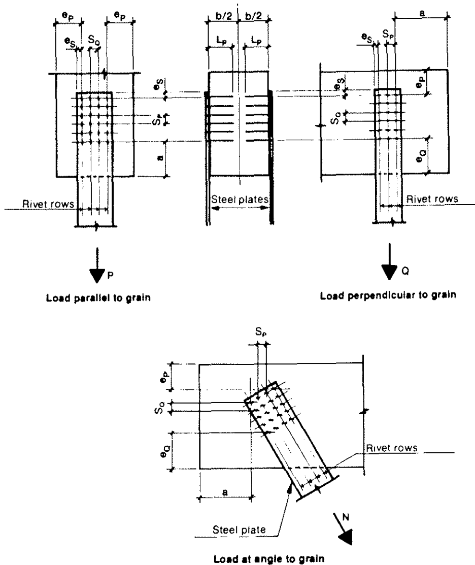
Minimum End and Edge Distances for Glulam Rivet Joints
