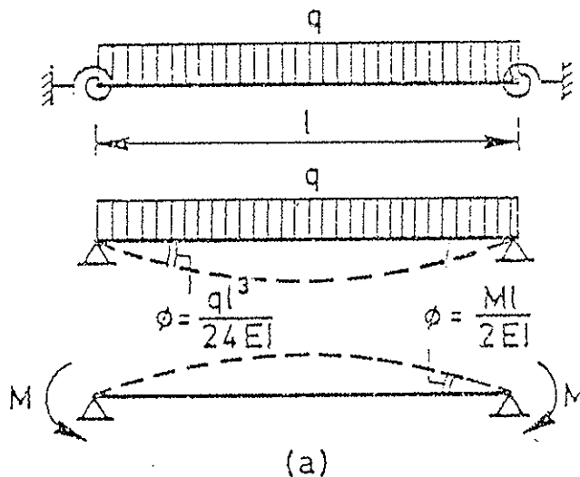
fig 1: Beam in braced frame
