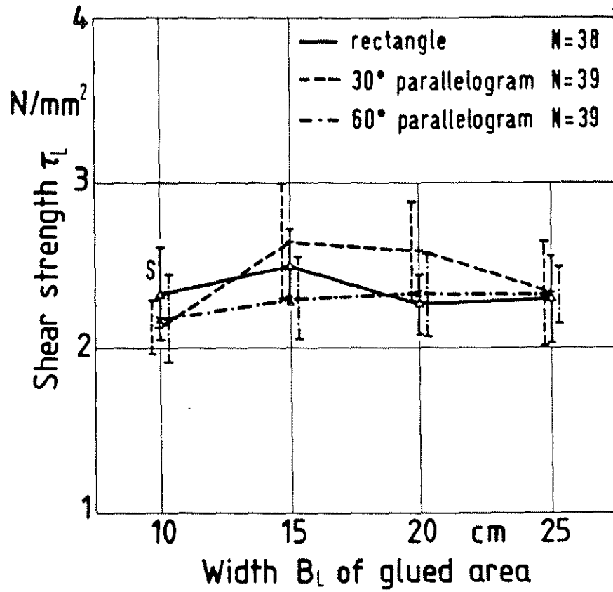
Figure 7: Effect of width B_L of glued area on shear strength \tau_L ( l_{e1} = 5 cm, \alpha = 0^\circ , L_L = 20 cm) s = standard deviation
