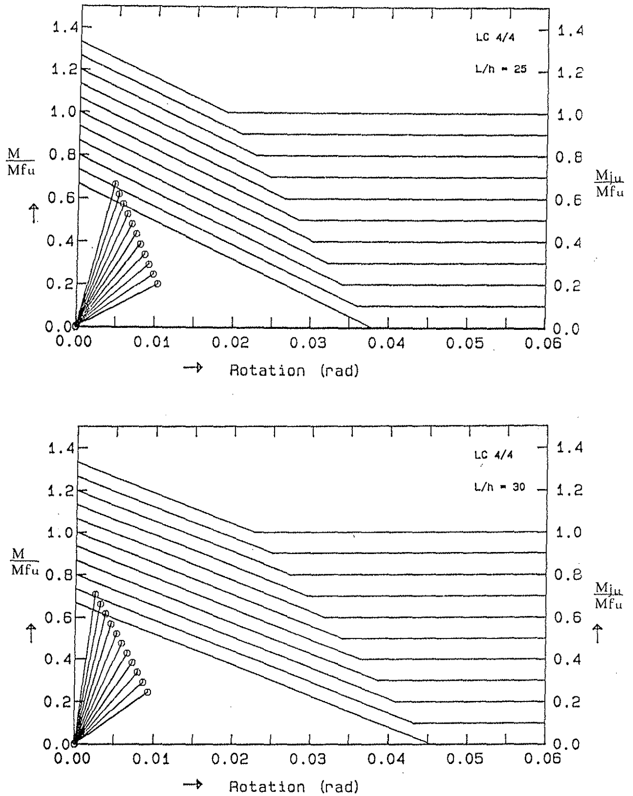
fig.4: Normalized moment - rotation graph with \beta increments of 0.1 Timber grade LC 4/4 (Eurocode5): L/h = 25 and 30
