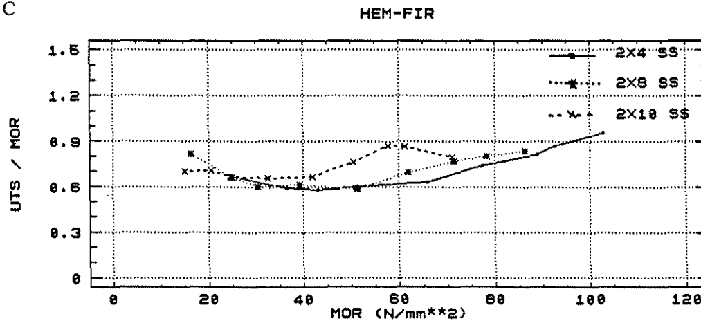
Figure 13. Tension/Bending Property Ratios for Case A, B, C Test Configurations - Hem-Fir, Select Structural Grade.
