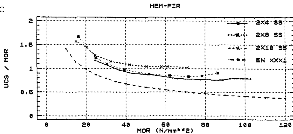
Figure 15. Compression/Bending Property Ratios for Case A, B, C Test Configurations - Hem-Fir, Select Structural Grade.
