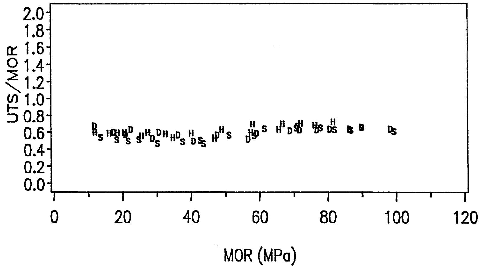
Figure 7.--Relationship between ultimate tensile stress parallel to the grain and modulus of rupture for In-Grade data at 12% moisture content.
