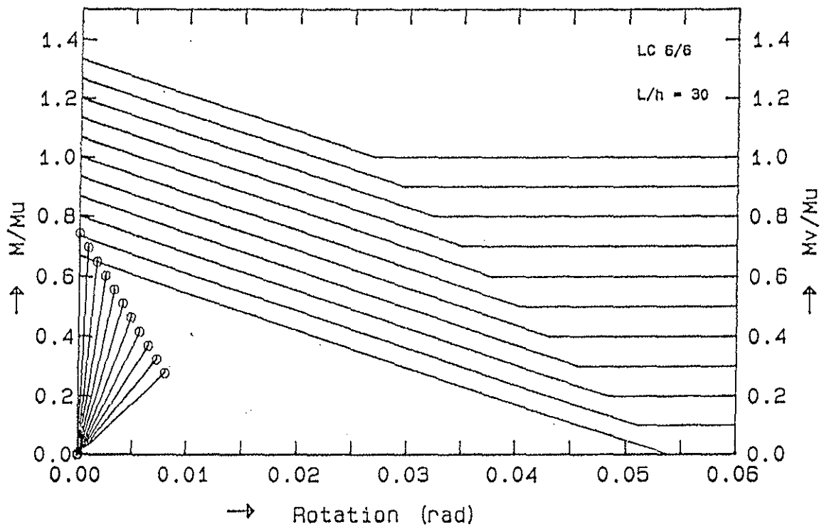
fig.5:: Normalized moment - rotation graph with \beta increments of 0.1 Timber grade LC 6/6 (Eurocode5): L/h = 25 and 30
