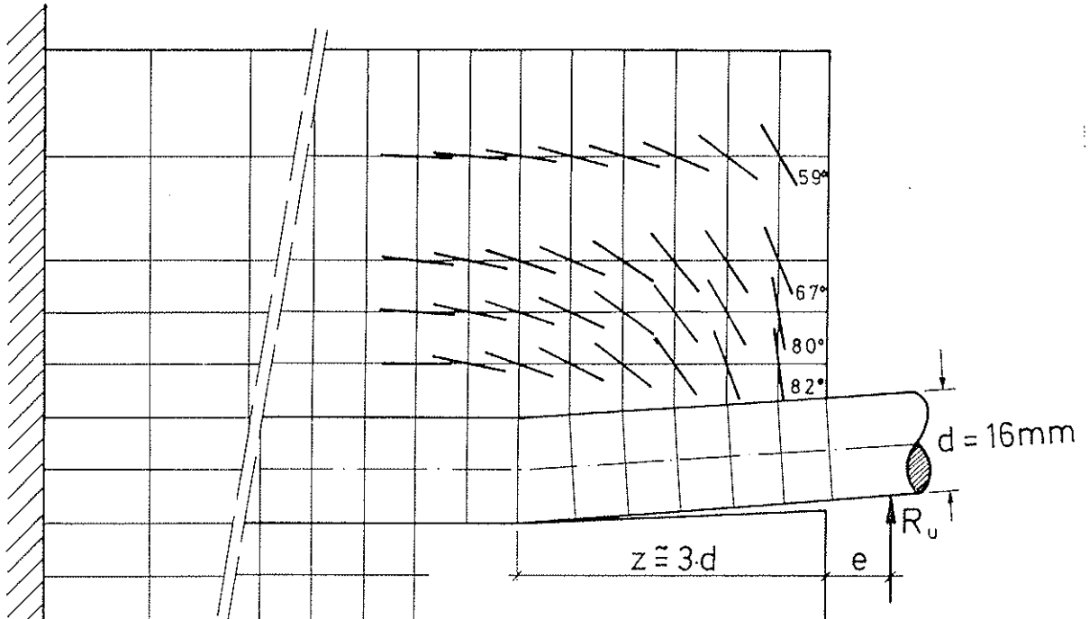
Fig.7: Stress distribution in the end-grain area of timber (FE-calculation); steel bolt diameter d = 16 \text{ mm}
