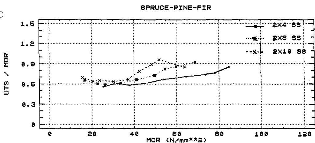
Figure 5. Tension/Bending Property Ratios for Case A, B, C Test Configurations - S-P-F, Select Structural Grade.
