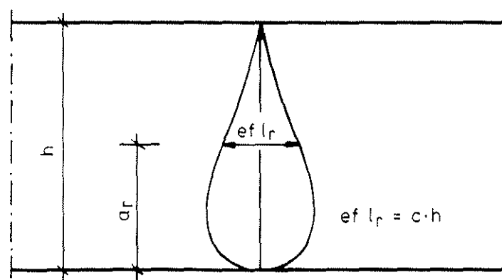
Fig. 7: Assumption for ef l_r in case of one fastener per row, only
