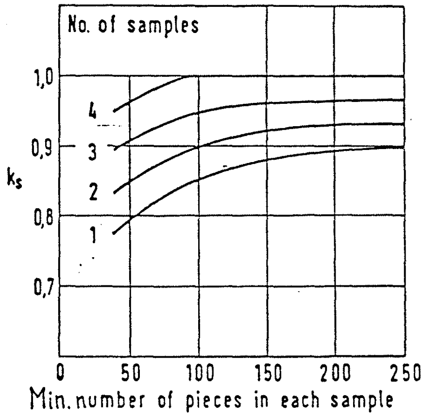
Figure 10.-- Relationship between the factor k_s and the number of samples and number of pieces in each sample in Eurocode 5 (Glos and Fewell, 1989).
