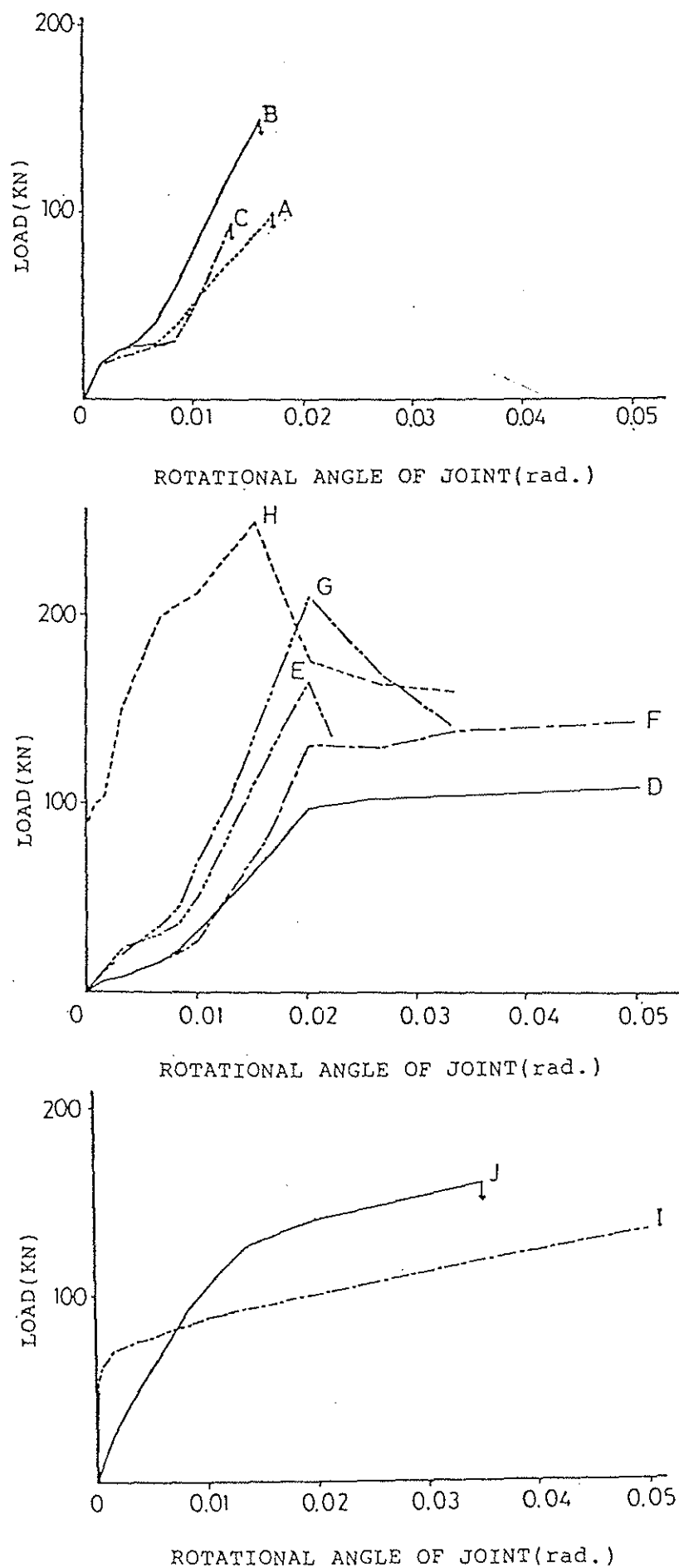
Fig.7 RELATION BETWEEN LOAD AND ROTATIONAL ANGLE OF JOINT
