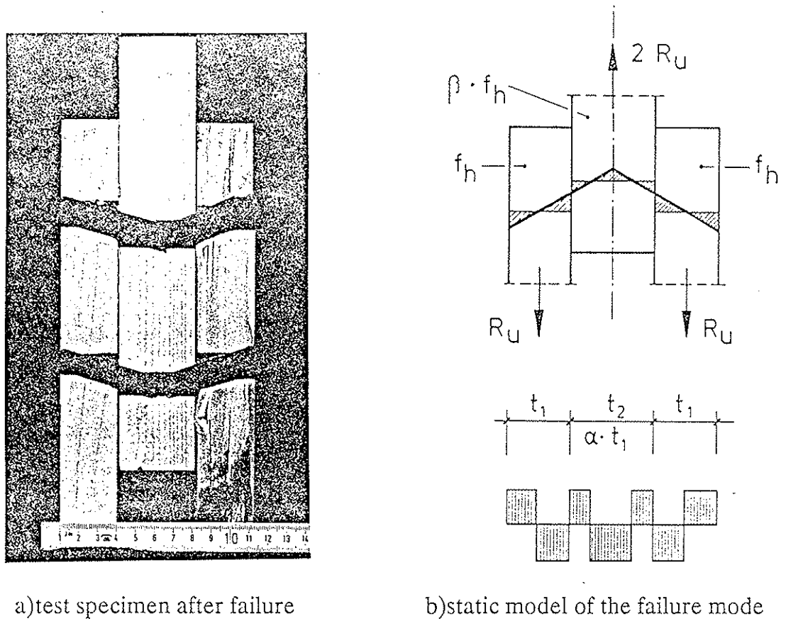
Fig. 3: Failure mode 3a (only one bending failure of the dowels)
