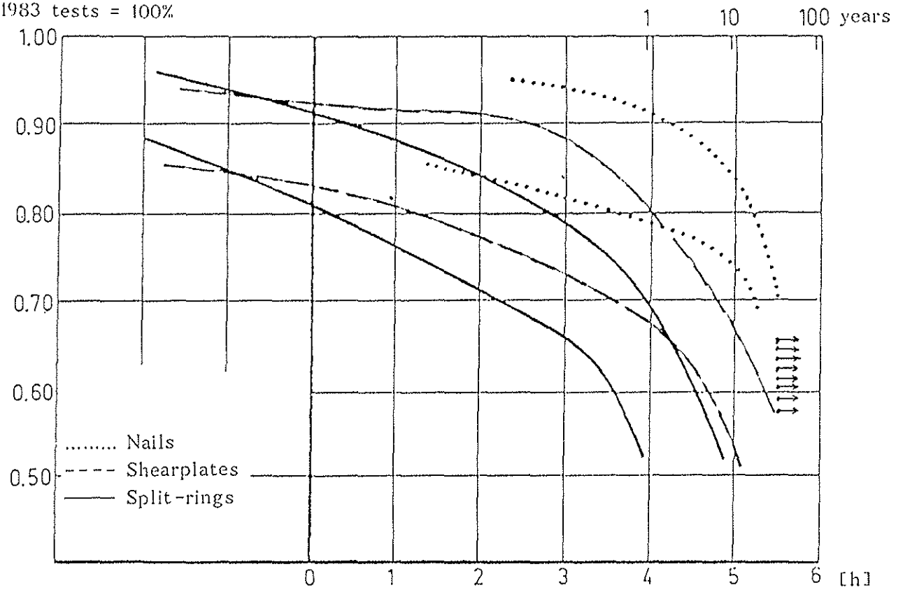
Fig.1: Upper and lower boundary of failed joints
