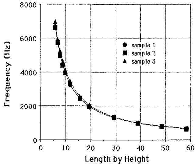
Figure 5. Effect of length by height of specimen on measuring fundamental vibration frequency
