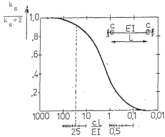
fig.2 : The bending moment at the joint in relation to the joint stiffness as given by form.(4).
