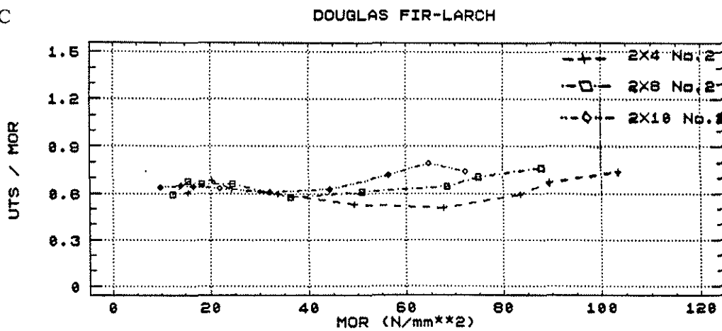
Figure 10. Tension/Bending Property Ratios for Case A, B, C Test Configurations - D-Fir-L, No. 2 Grade.
