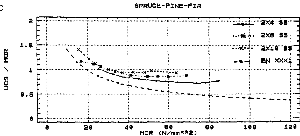
Figure 7. Compression/Bending Property Ratios for Case A, B, C Test Configurations - S-P-F, Select Structural Grade.
