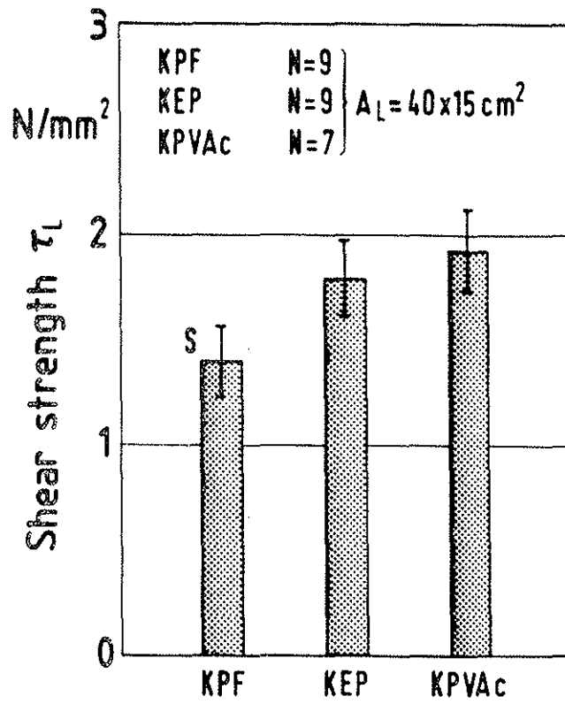
Figure 11: Effect of glue type on shear strength \tau_L ( L_L = 40 \text{ cm} , B_L = 15 \text{ cm} , \alpha = 0^\circ , l_{e1} = 5 \text{ cm} ) s = standard deviation
