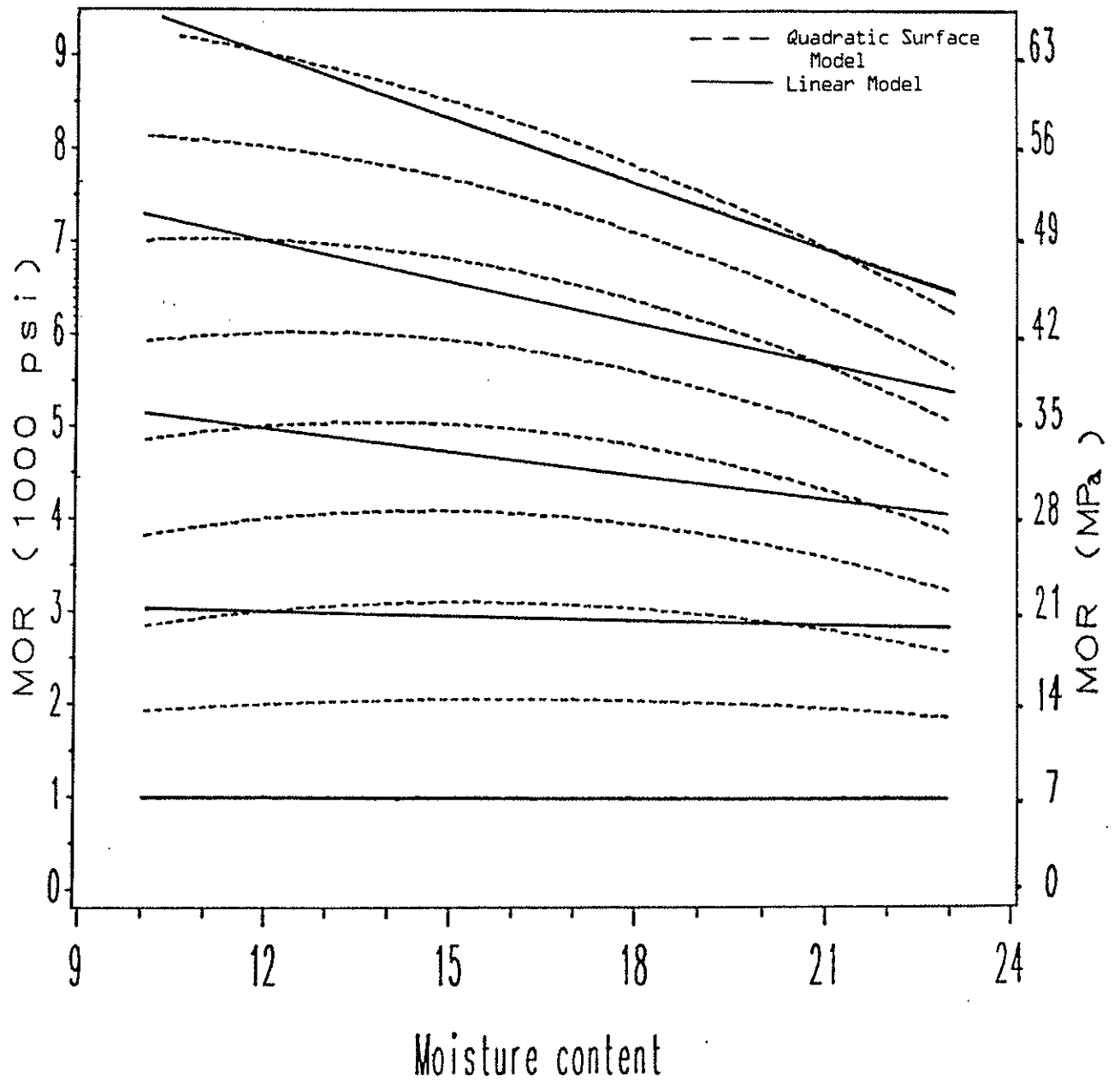
Figure 12.--Comparison of quadratic surface (QSM) (Green and Evans, 1989a) and linear models for predicting effect of moisture content on modulus of rupture.
