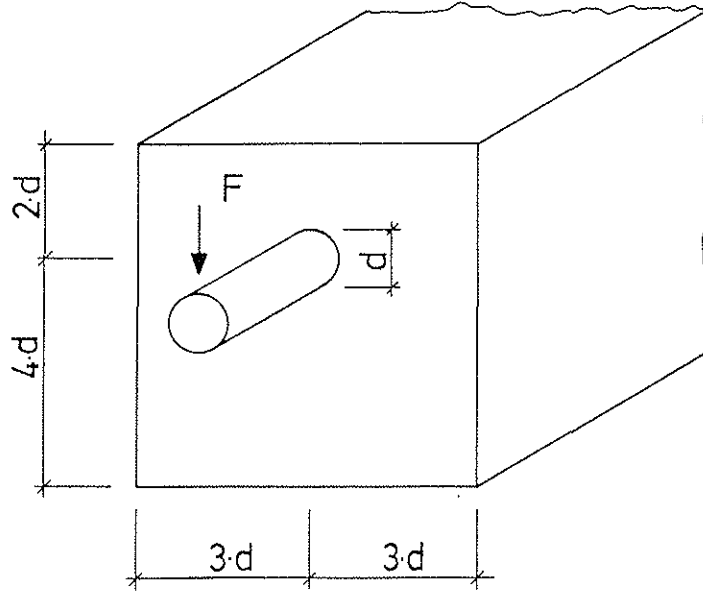
Fig.3: Minimum edge distances to avoid perpendicular-to-grain tension failures
