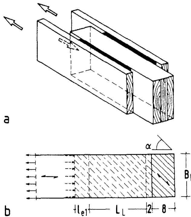
Figure 2: Specimen for basic joint tests a) Threedimensional view b) Side view
