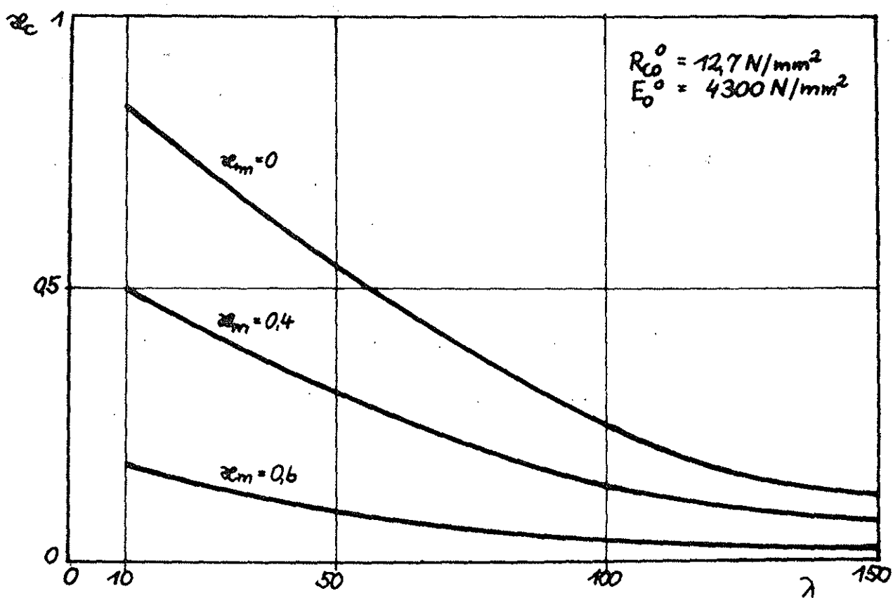
Figure 3: Dependence of \chi_c on \lambda for different \alpha_m ( K_M = 0 )
