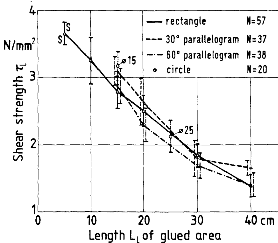
Figure 8: Effect of shape of glued area on shear strength \tau_L for different lengths of glued area ( l_{e1} = 5 cm, \alpha = 0^\circ ) s = standard deviation
