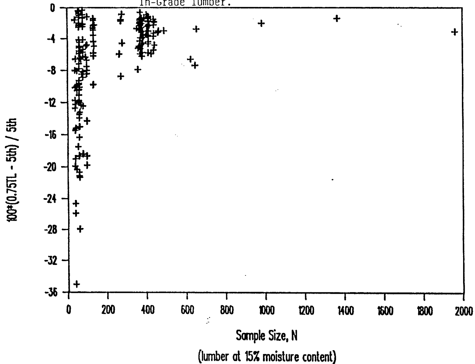
Figure 11.--Relationship between nonparametric tolerance limit and 5th percentiles for bending and tensile strength of In-Grade lumber.
