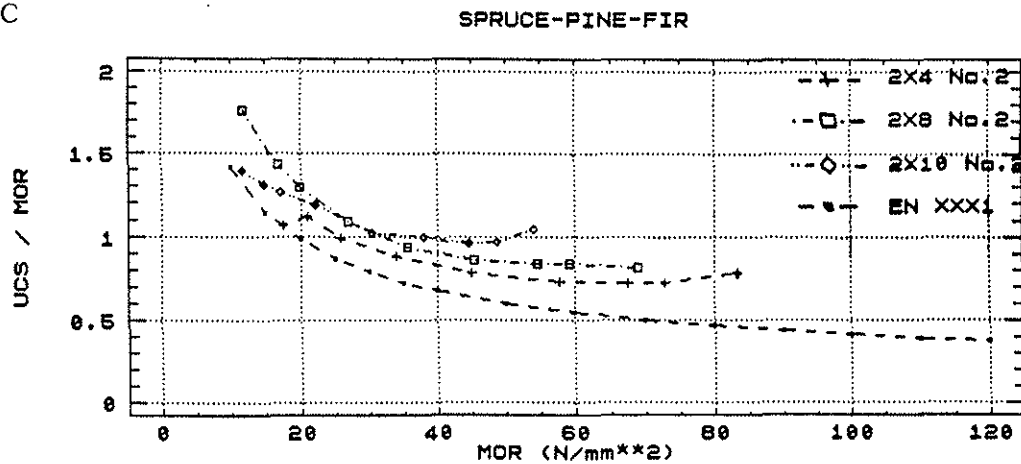
Figure 8. Compression/Bending Property Ratios for Case A, B, C Test Configurations - S-P-F, No. 2 Grade.
