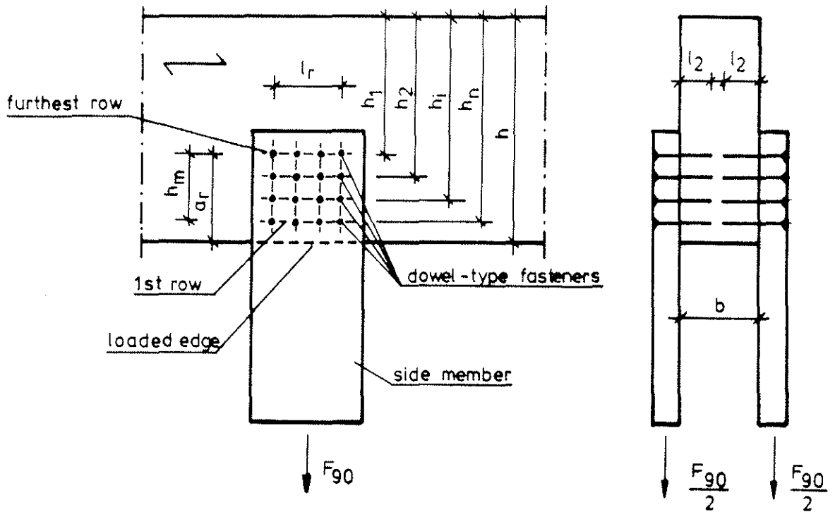
Fig. 4: Joint with F_{90} acting perpendicular to grain ( notations ).
