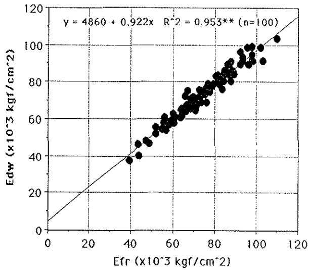
Figure 1. Relationship between E_{fr} and E_{dw} on sugi squares
