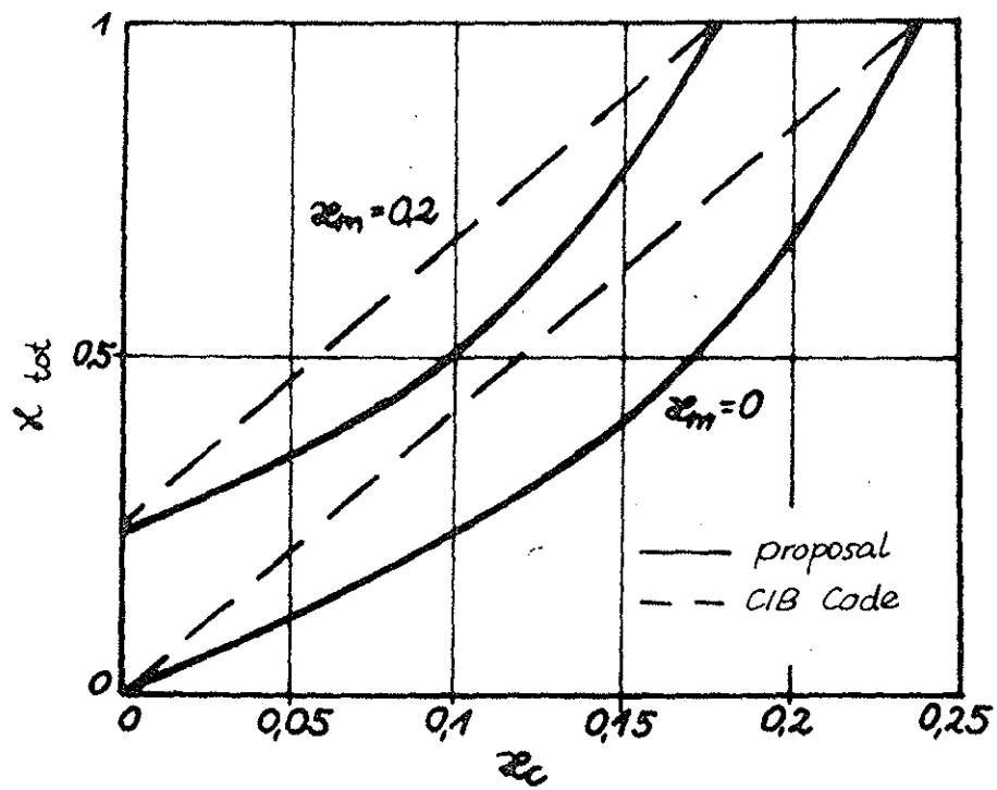
Figure 4: Comparison in terms of the components of X_c and X_m in X_{tot} for \lambda = 100
