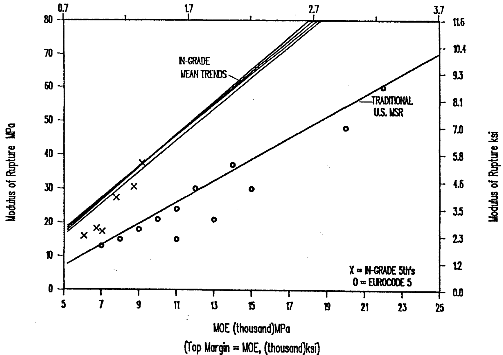
Figure 3.--Relationship between modulus of elasticity and modulus of rupture at 12% moisture content.
