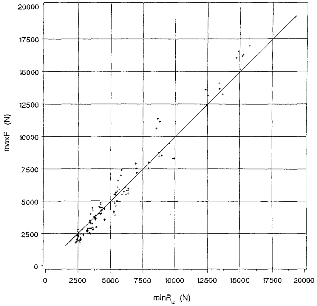
Fig. 6: Comparison of test results with calculated values
