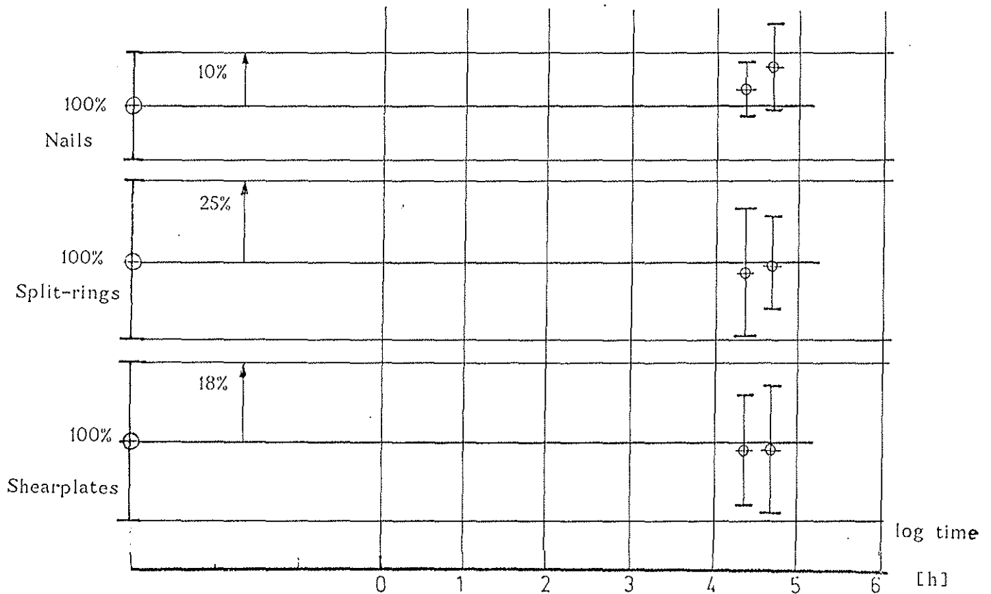
Fig.2: Comparison of the Standard Short Duration strength of joints with various load history. The strength of the joints without any load duration history is set to 100% while the 95% probability of these results is also indicated, see Table 1.
