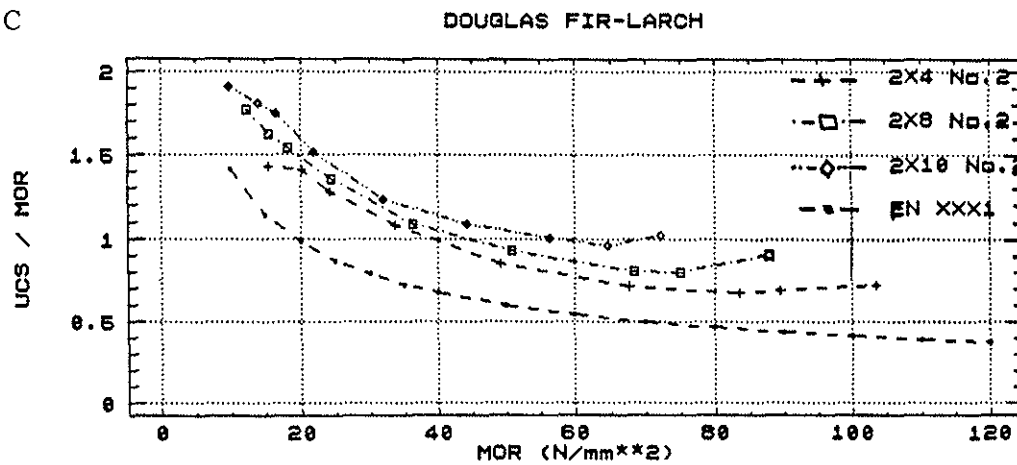
Figure 12. Compression/Bending Property Ratios for Case A, B, C Test Configurations - D Fir-L, No. 2 Grade.
