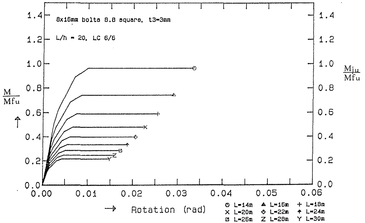
fig.9: Moment rotation curves of a steel reinforced joint with a square pattern 8 bolts of 16mm diameter, steel plate thickness t=3\text{mm} for increasing spans.
