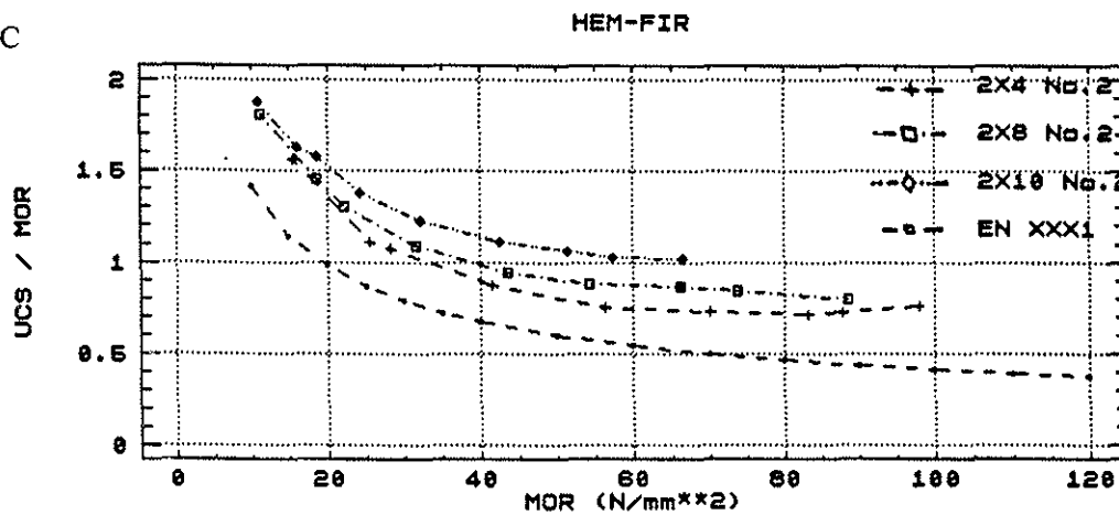
Figure 16. Compression/Bending Property Ratios for Case A, B, C Test Configurations - Hem-Fir, No. 2 Grade.
