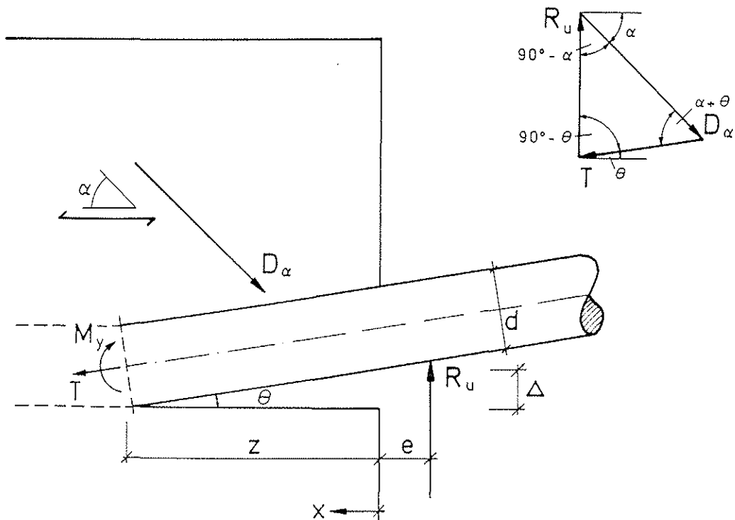
Fig.4: Resulting forces at ultimate limit state
