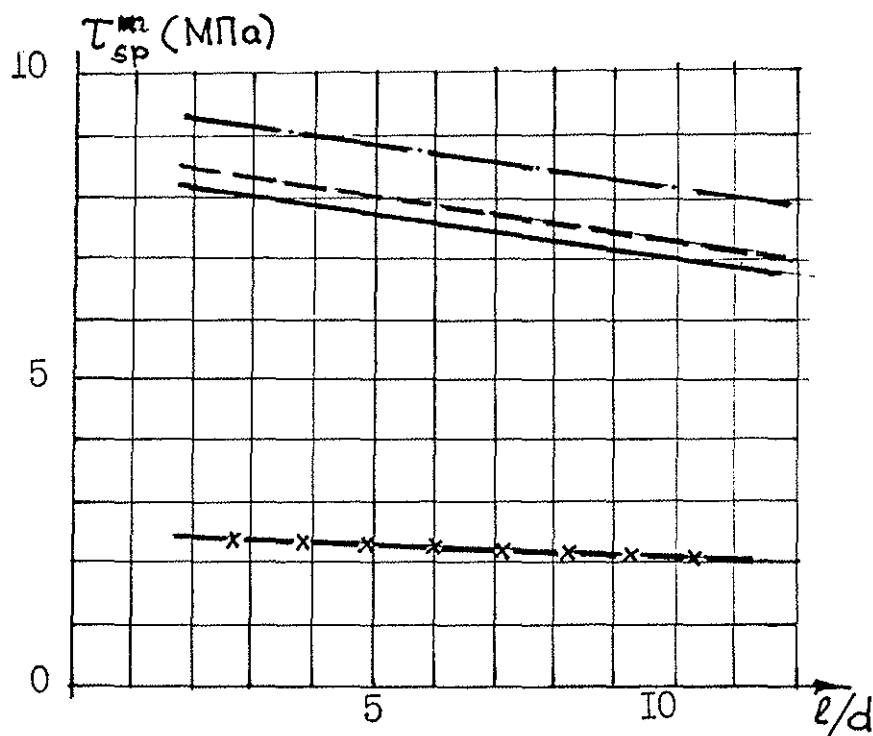
Fig. 2. Relationship graph for average spalling stress \tau_{sp}^m of 1/d .
