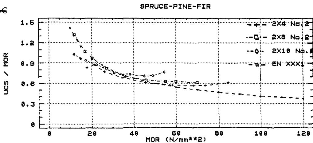
Figure 4. Compression/Bending Property Ratios for D Fir-L, Hem-Fir and S-P-F, No. 2 Grade.
