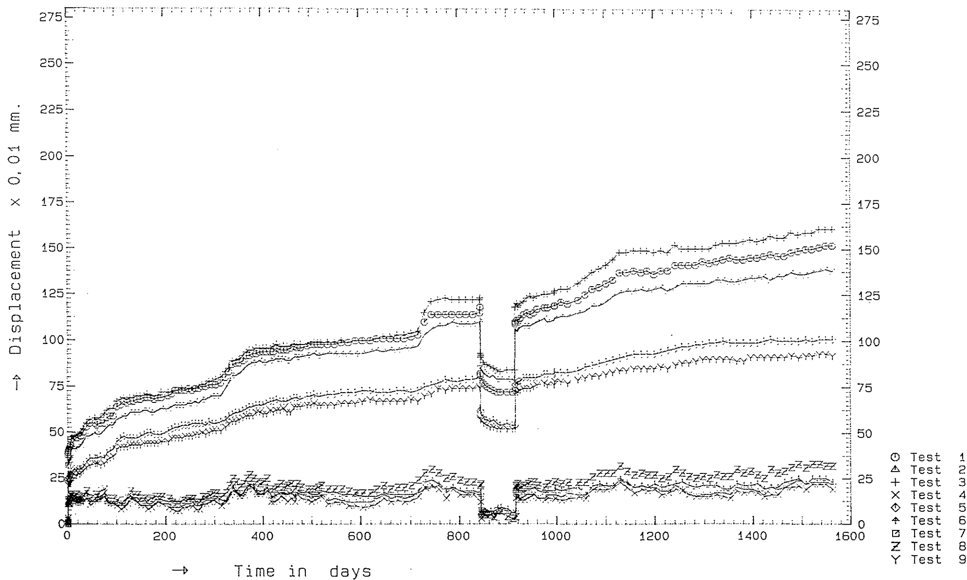
fig.4: Creep results of joints with splittings and steelplate reinforced joints. The data of the reinforced joints is found at the bottem of the graph. During the first 2 years the load level was 40% afterwards 50%.
