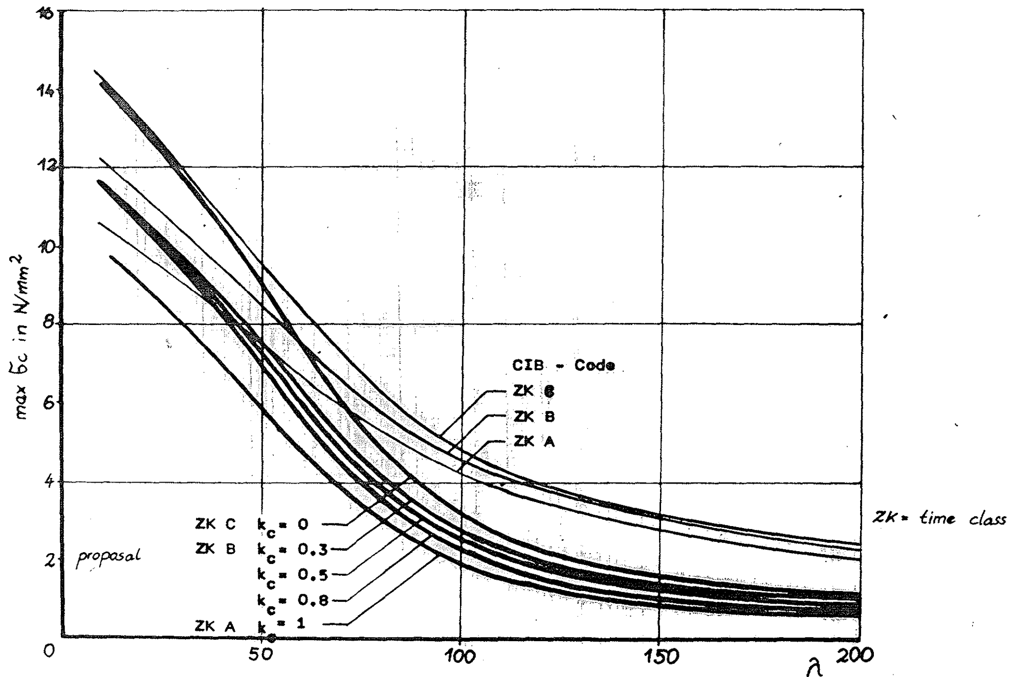
Figure 5: Dependence of \max G_c on \lambda acc. to the proposal and acc. to the CIB Code
