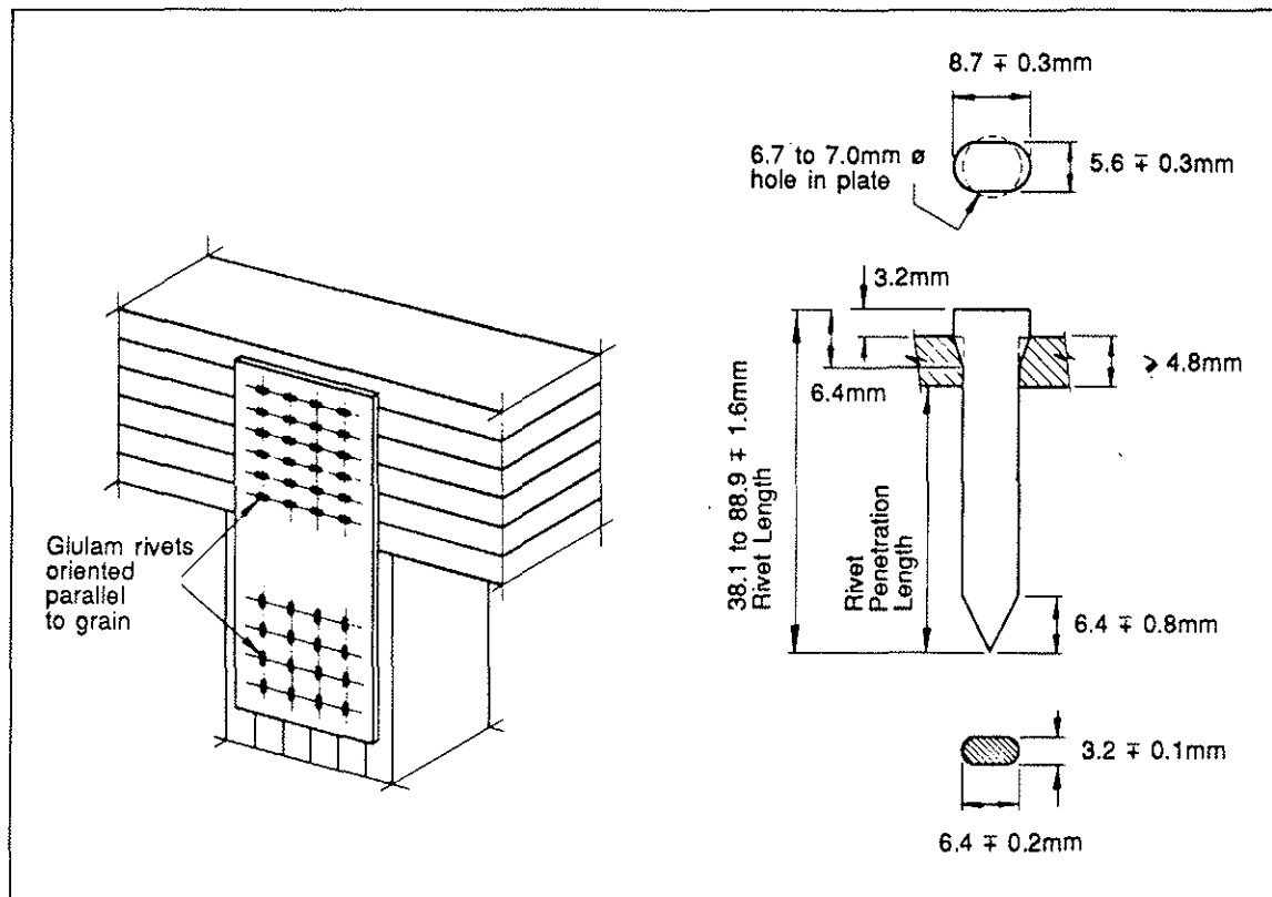
Figure 1 Typical Glulam Rivet Connection
