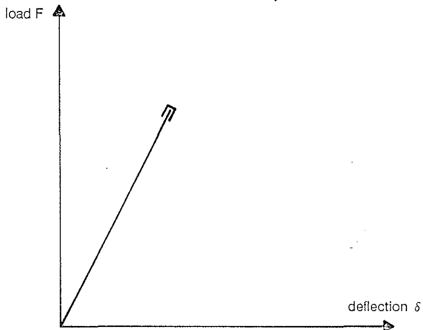
Fig. 2: Typical load - deformation relationship of the fastener material used
