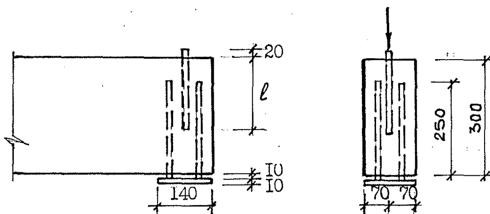
Fig. 1. Specimens of joints on steel bars glued-in across wood grain.
