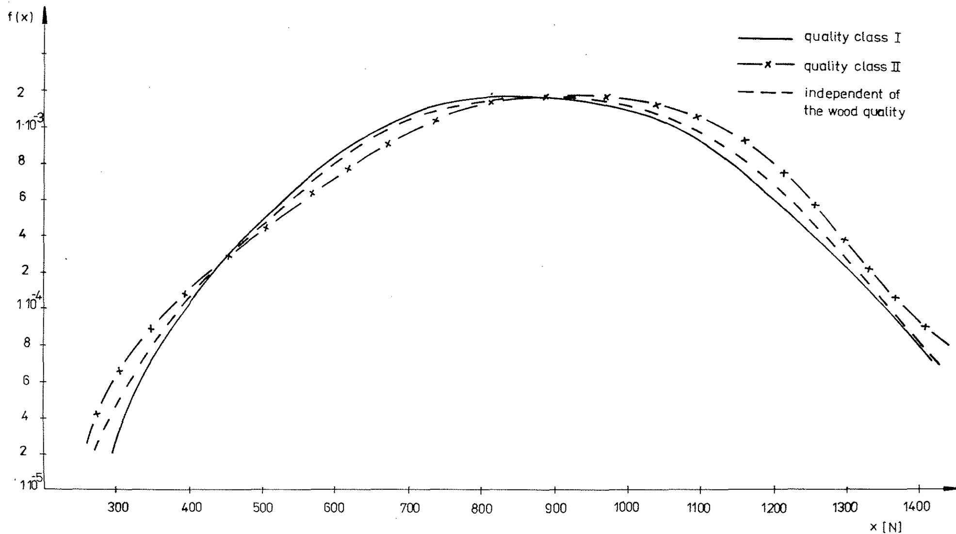
Figure 1. Distribution densities of the Weibull distribution for the ultimate loads F_{\max} /N/
