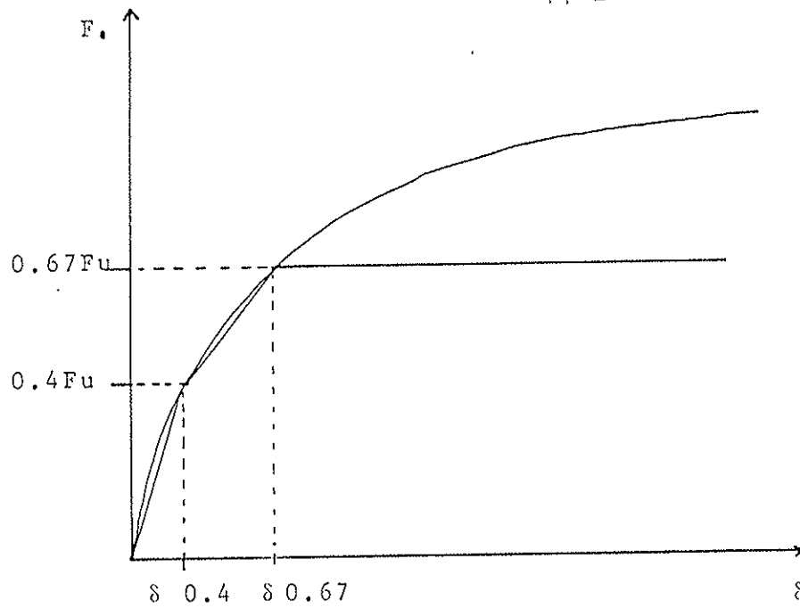
fig.6: Linear schematisation of the load slip curve of steel reinforced joints.
