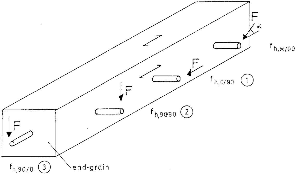
Fig.1: Different types of embedding strengths due to loaded steel bolts in timber
