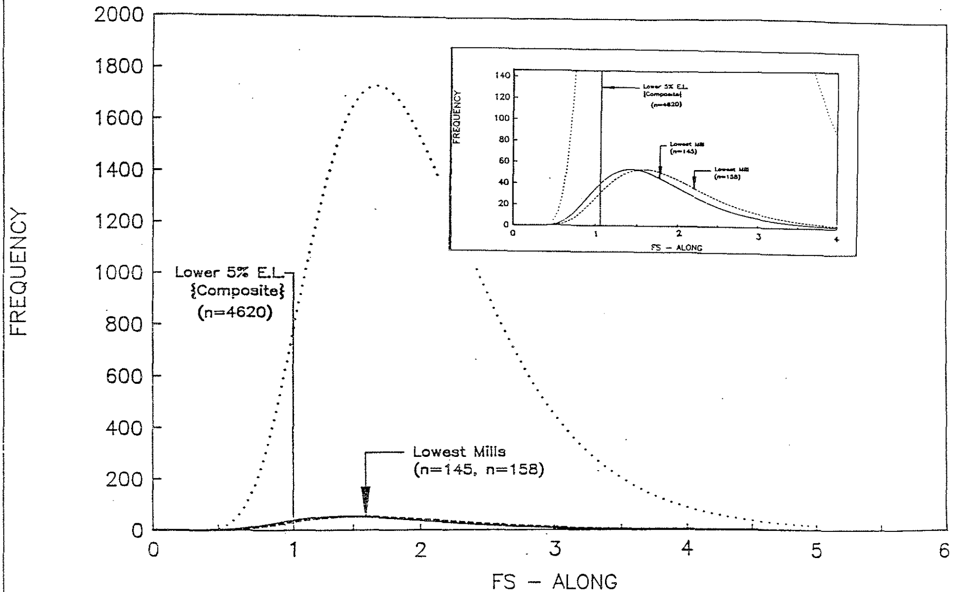
Figure 3. Comparison of subgroup samples with composite sample exclusion limits.
