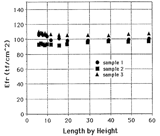
Figure 6. Effect of length by height of specimen on Efr for sugi 50 mm X 50 mm squares
