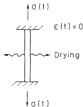
Fig. 1. Drying wood element under full restraint.
