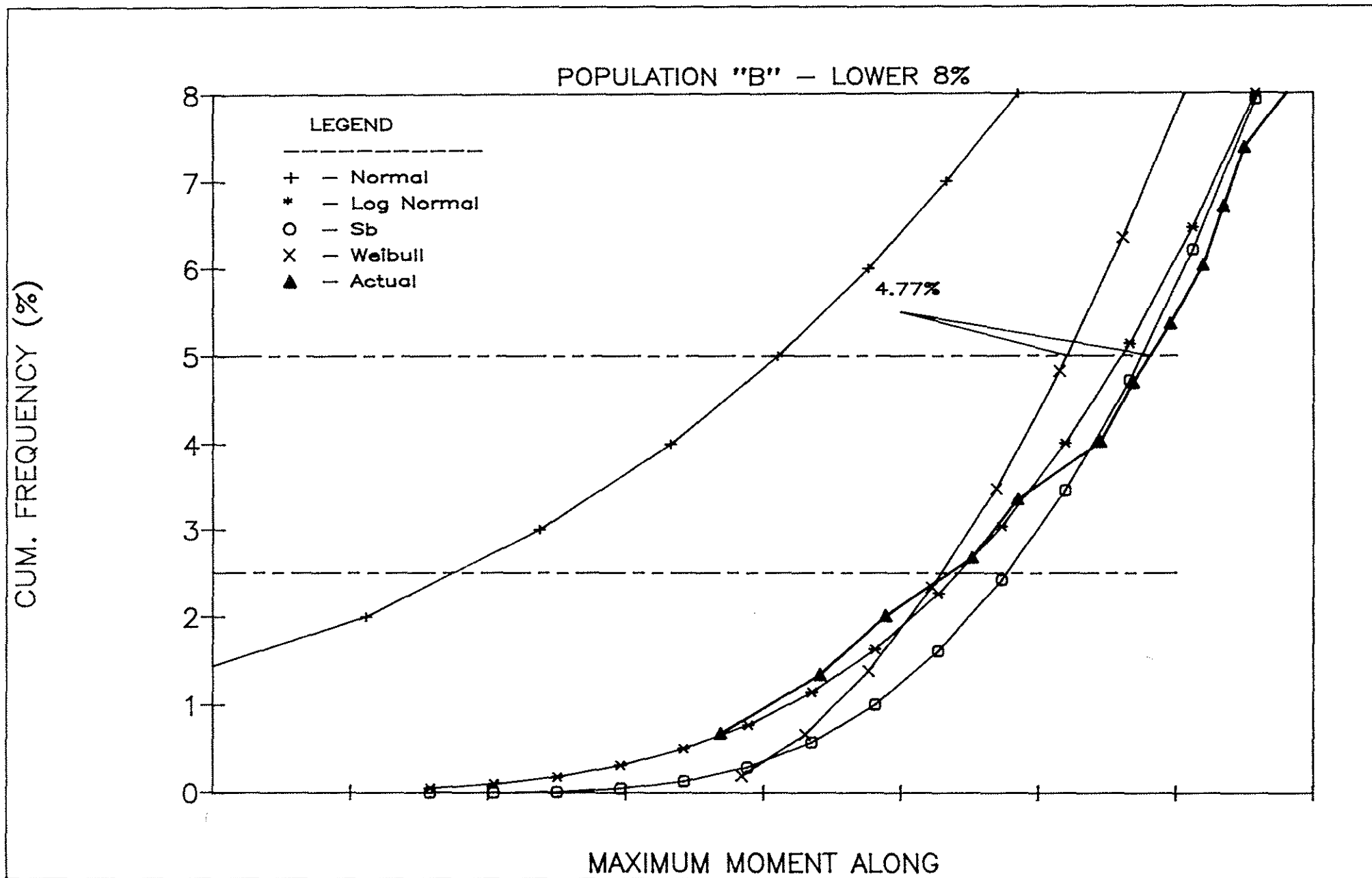
FIGURE 5. COMPARISON OF PROBABILITY DENSITY FUNCTIONS VERSUS ACTUAL TEST DATA FOR THE LOWER 8% OF STRENGTH ON TEST POPULATION "B".
