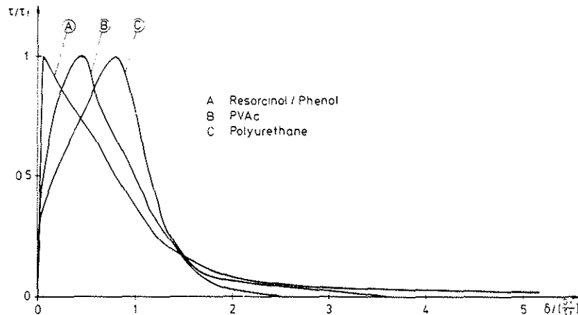
Figure 7. Normalized \tau - \delta curves for PVAc, polyurethane and resorcinol/phenol adhesives. R = .0625 mm/min, C = 4 days.
