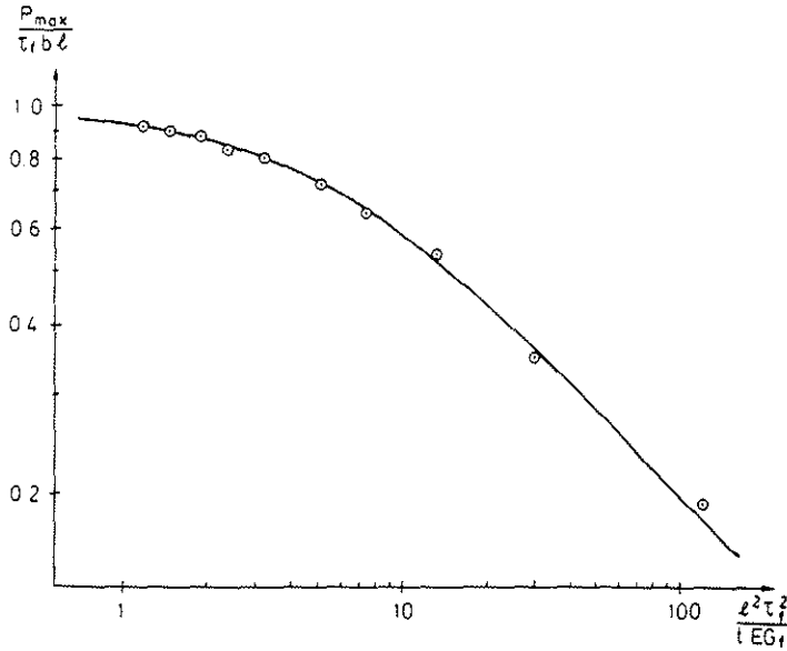
Fig 6. Strength of lap joints. Test results (Redux adhesive - light metal joints) from (Marian, 1954) compared with theoretical curve valid for \tau_f = 40 MPa and E G_f / \tau_f^2 = 22 mm.
