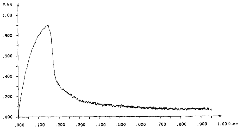
Figure 2. Example of recorded load versus displacement in the clip-gauges.
