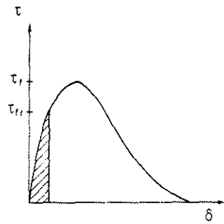
Fig 7. Simplified effective fracture energy when \tau_f > \tau_{fr} .
