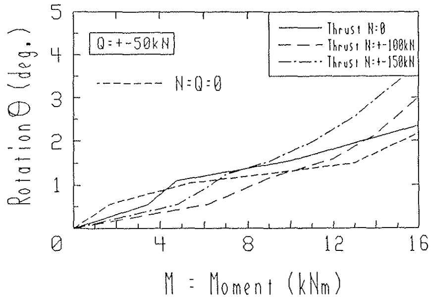
Fig. 6 Influence of N and Q on Rotation-Moment relationship (6 bolt connection)
