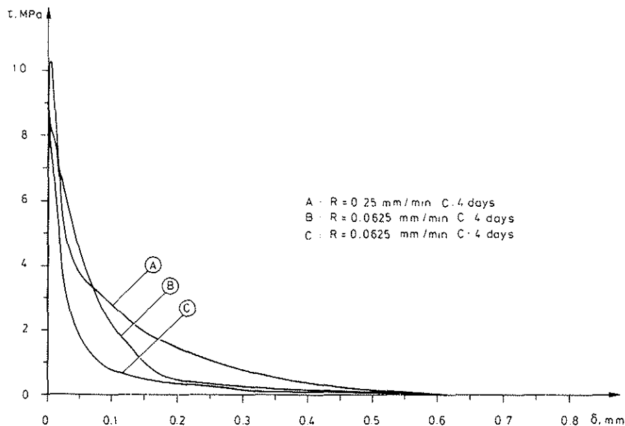
Figure 6. \tau - \delta curves for resorcinol/phenol, tested at different rate of deformation (R) and after different curing time (C).
