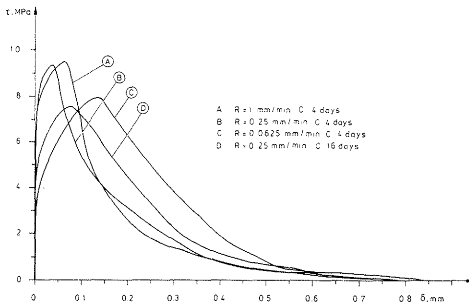
Figure 4. \tau - \delta curves for PVAc, tested at different rate of deformation (R) and after different curing time (C).
