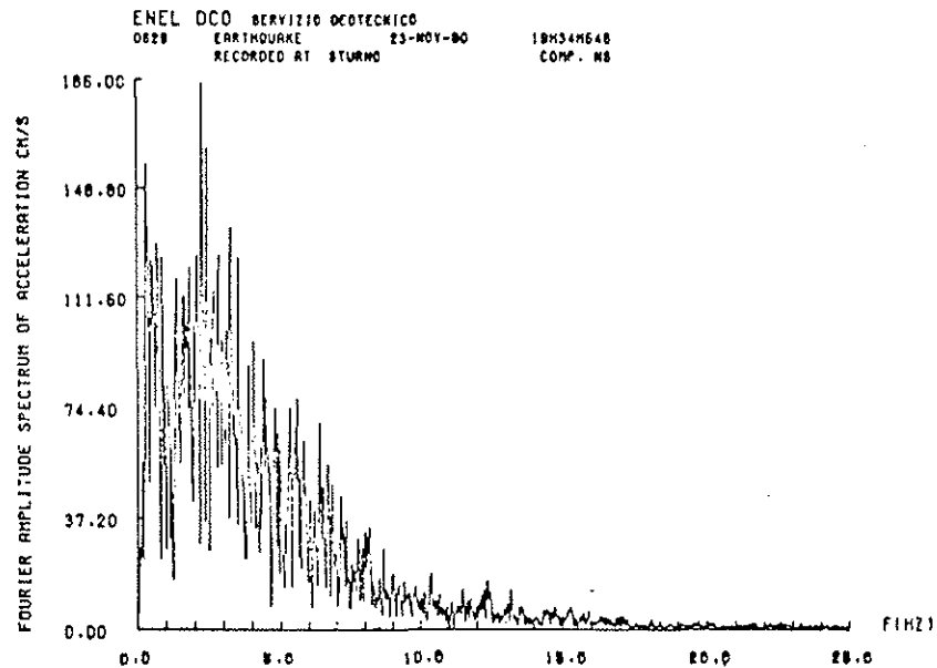
Fig. 1 - Campania-Lucania Earthquake: Sturmo N-S Accelerogram a); Acceleration Response Spectra b); and Fourier Spectrum c).
