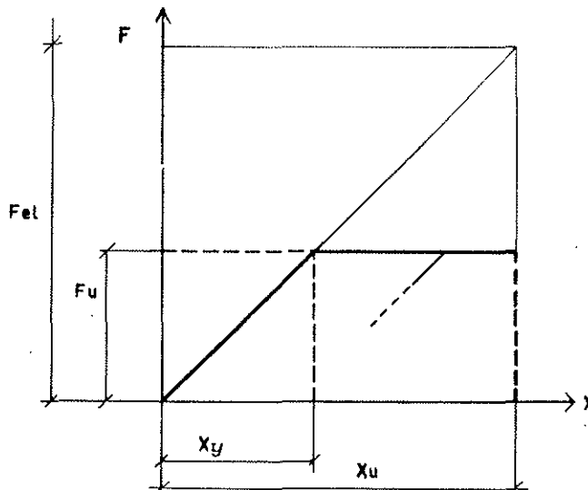
Fig. 3 - Conventional Load-Displacement Diagrams
