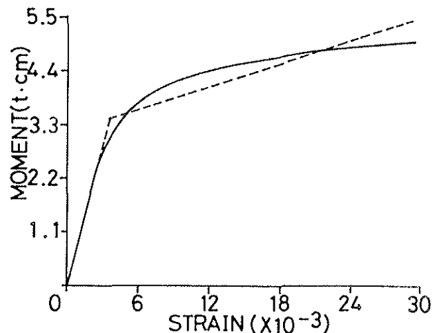
Fig.7 Relation between the moment and the strain in bending test of a bolt
