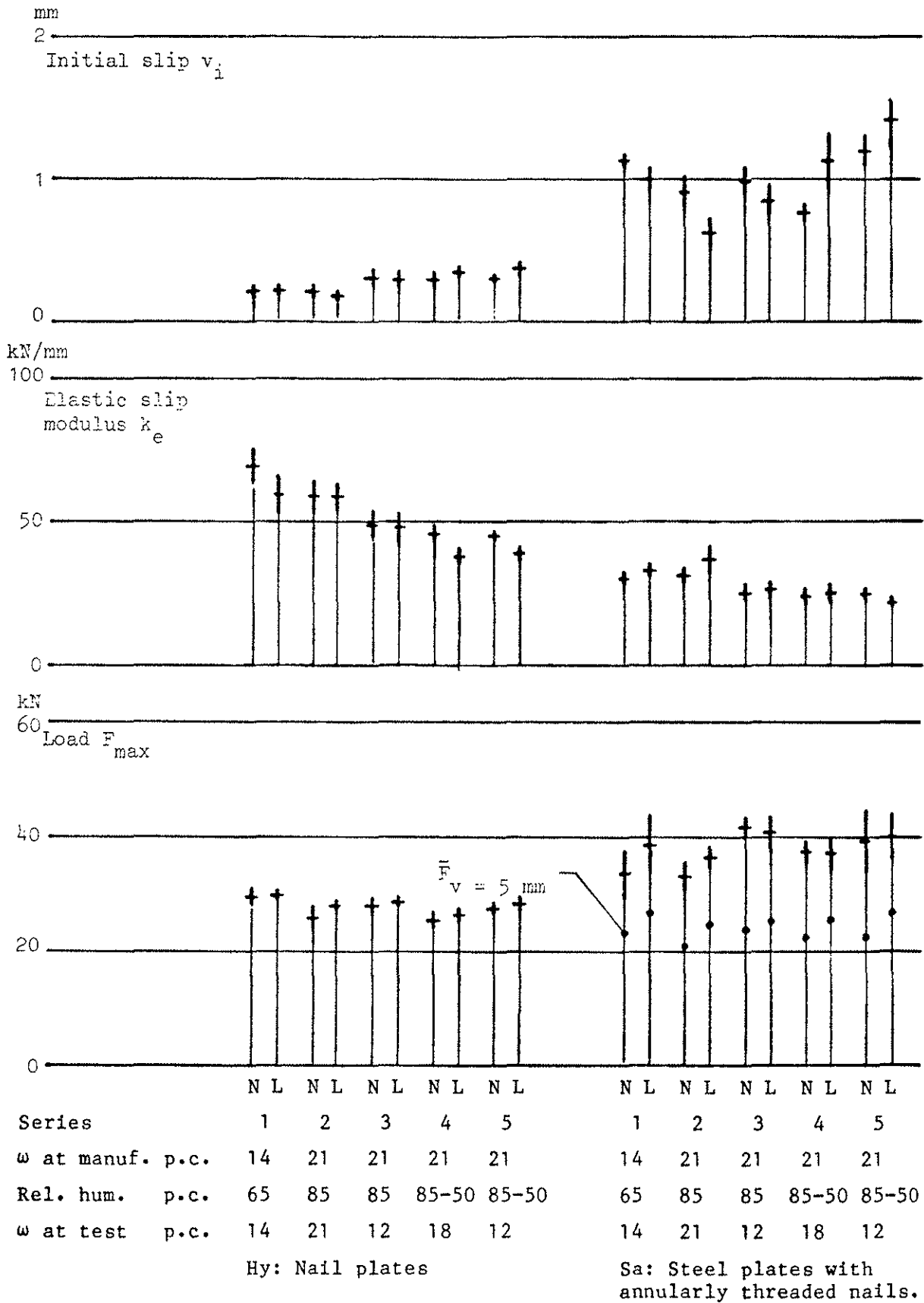
Figure 11 Stiffness and strength from short-term testing of (N) non-preloaded and (L) long-term loaded joints with nail plates and steel plates. Average values and 95 p.c. confidence intervals from 6 specimens.
