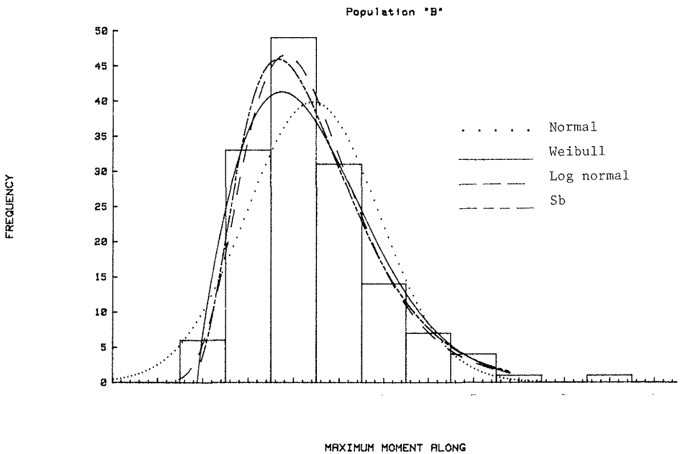
FIGURE 4. PROBABILITY DENSITY FUNCTIONS FOR STRENGTH (MAXIMUM MOMENT) ON TEST POPULATIONS "A" AND "B".
