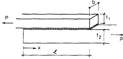
Fig 1. Geometry of single-lap joint. t_1 E_1 / (t_2 E_2) = \alpha \leq 1.0 .
