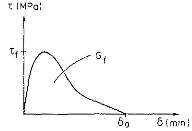
Fig 2. Constitutive relation of bond line.
