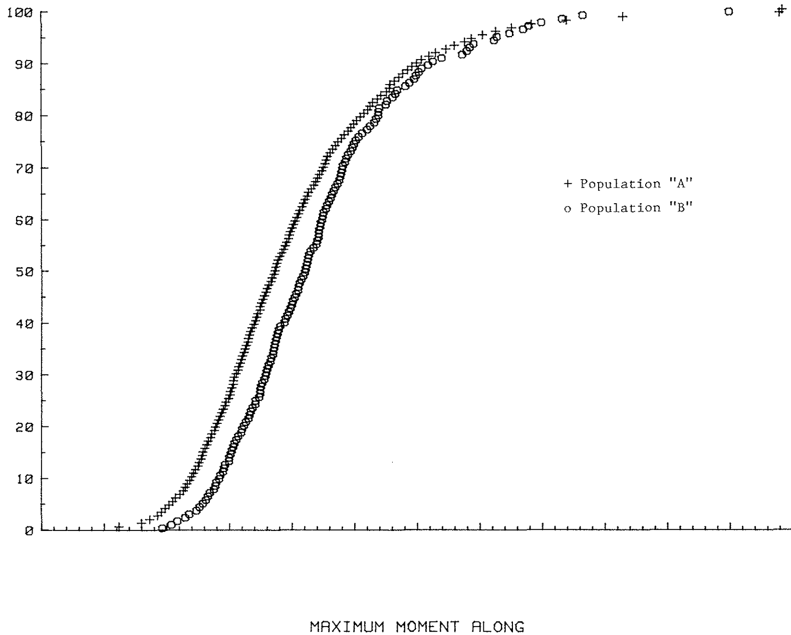
FIGURE 2. CUMULATIVE DISTRIBUTION FOR STRENGTH (MAXIMUM MOMENT) ON TEST POPULATIONS "A" AND "B".
