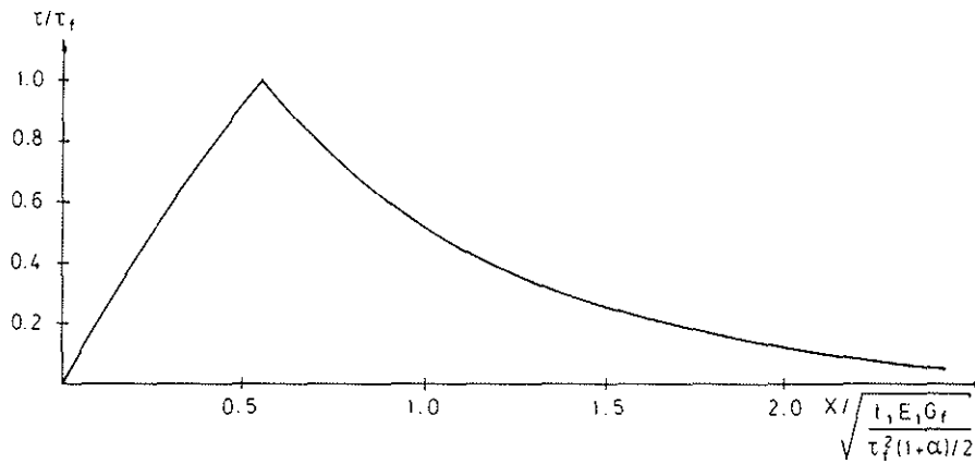
Fig 3. Stress distribution in a fracture region moving along the bond line during fracture of a brittle joint. Const. prop. according to Fig 4b).
