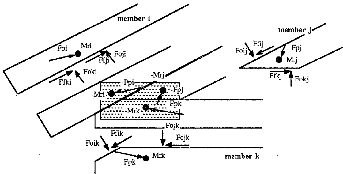
Fig. 1, A nail plate heel joint and its actions (forces and moments)
