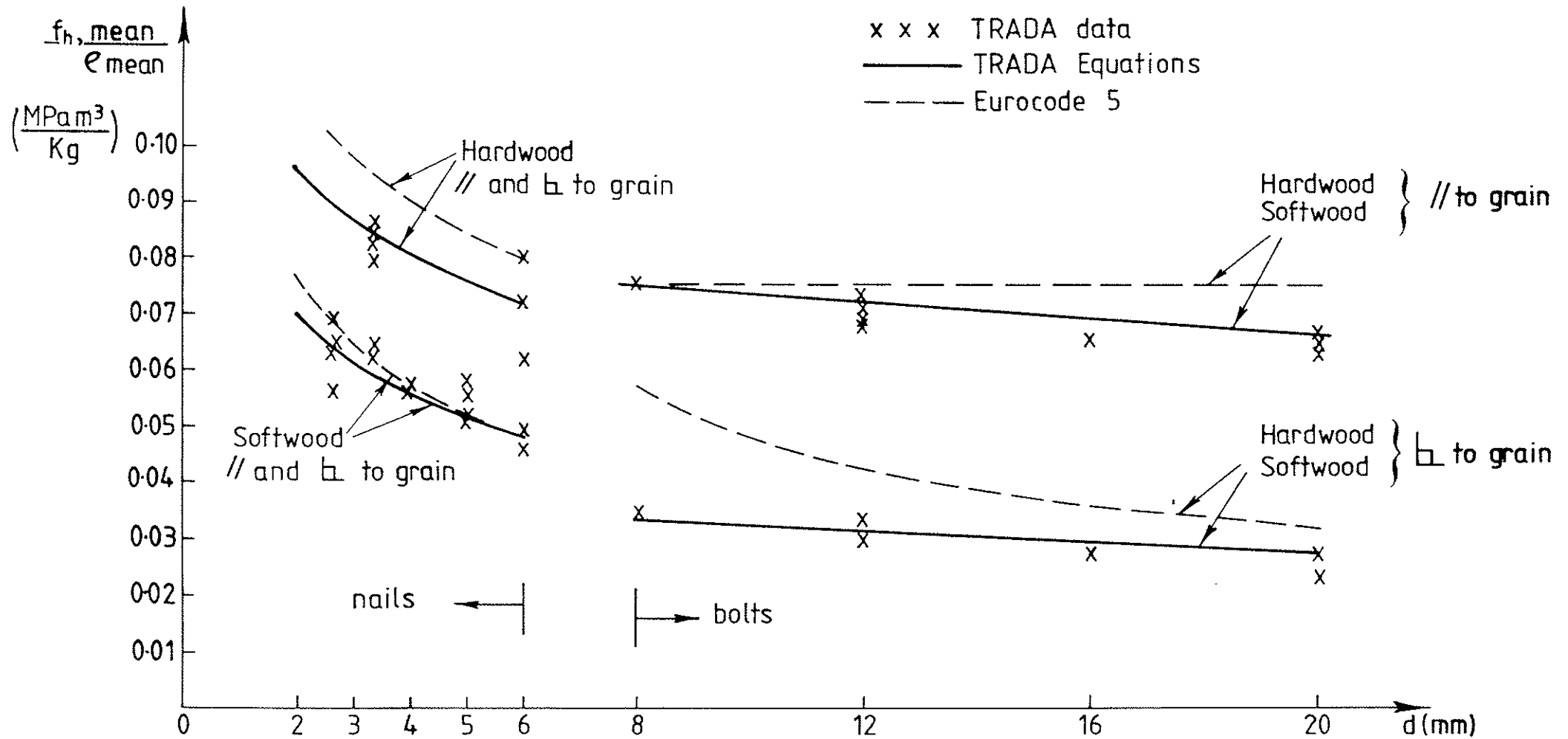
Figure 1 f_{h, \text{mean}}/e_{\text{mean}} as a function of diameter d for nails or bolts in solid timber
