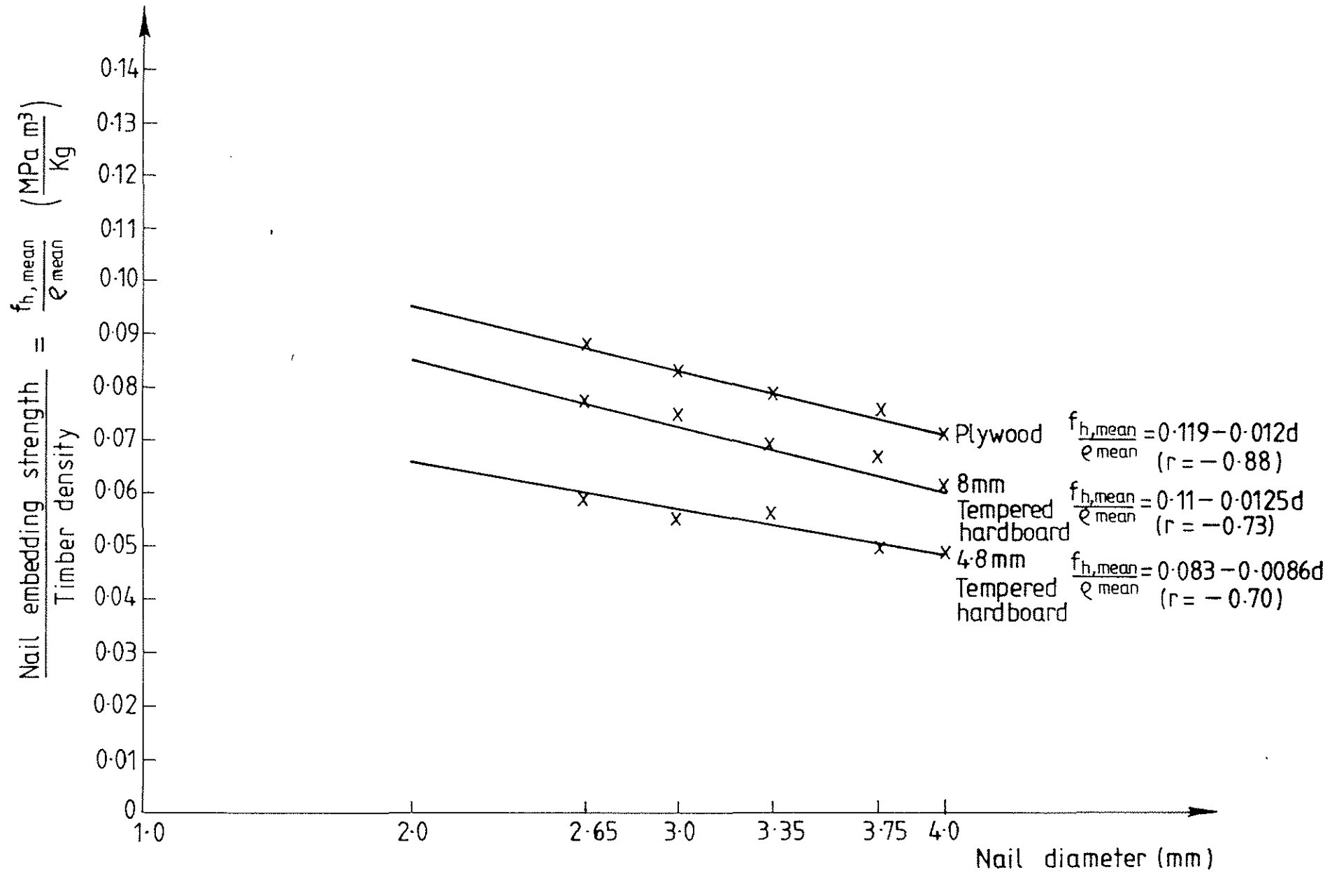
Figure 9 f_{h, \text{mean}} / e_{\text{mean}} as a function of diameter d for nails in sheet materials
