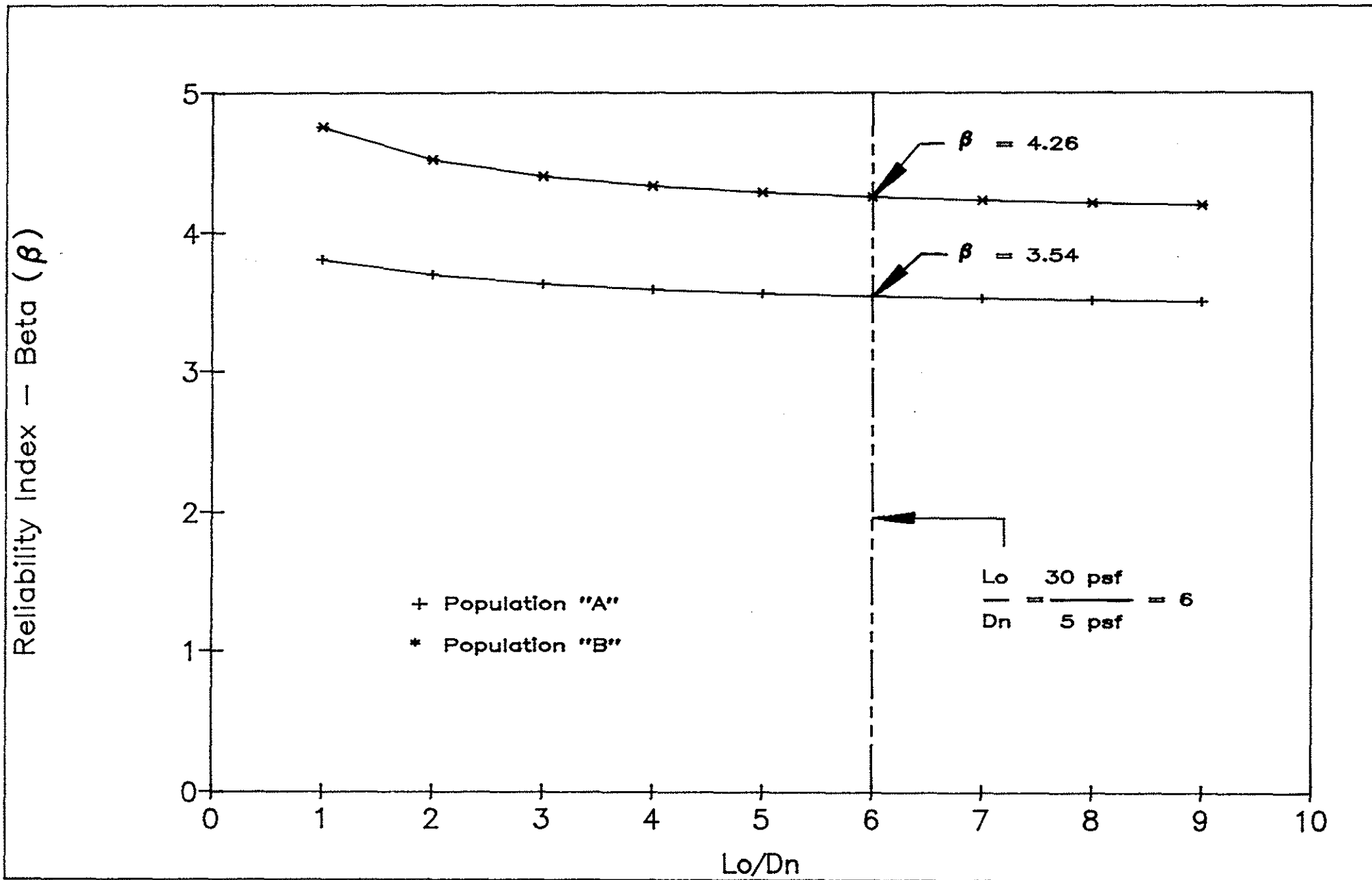
FIGURE 6. COMPARISON OF BETAS BETWEEN TEST POPULATIONS "A" AND "B".
