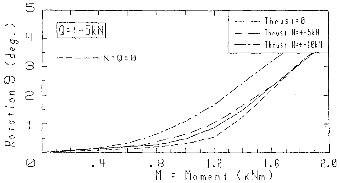
Fig. 5 Influence in N and Q on Rotation-Moment relationship (15 nail connection)
