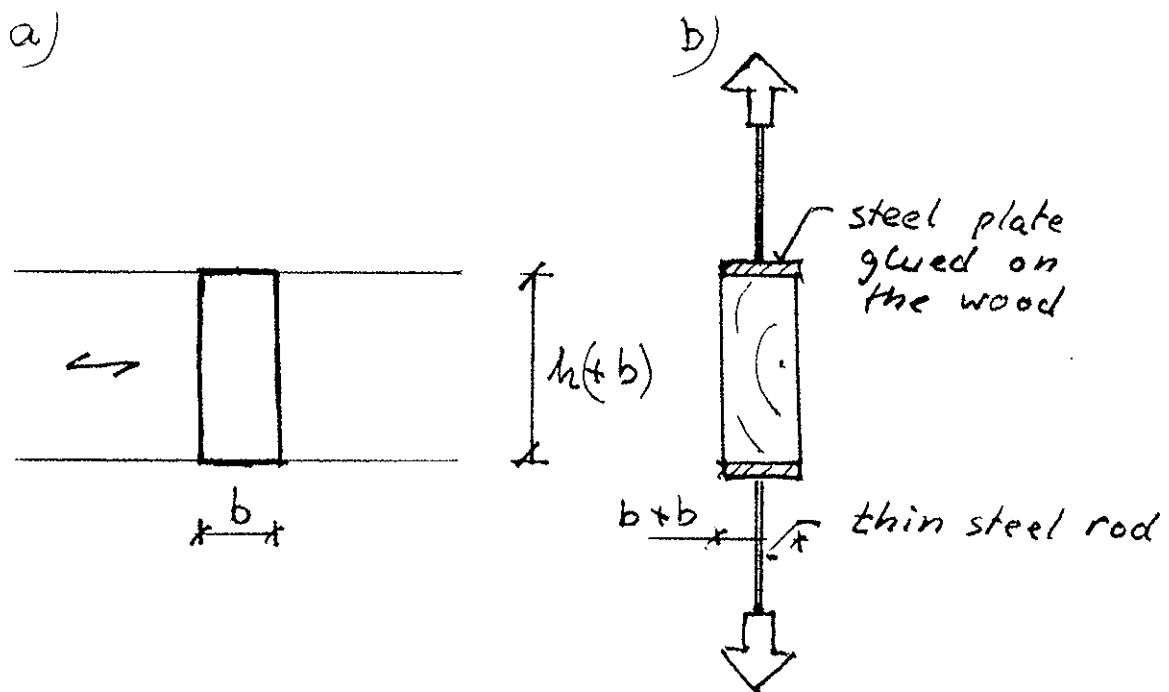
Figure 1. a) Specimen with square cross-section b \times b is cut from a beam with depth h and width b b) Steel plates are glued to the wood, and the load transferred through thin steel rods.
