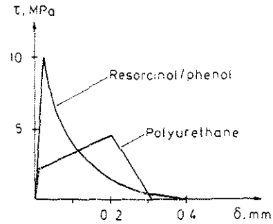
Fig 8. Schematic \tau - \delta curves for two adhesive bond lines.
