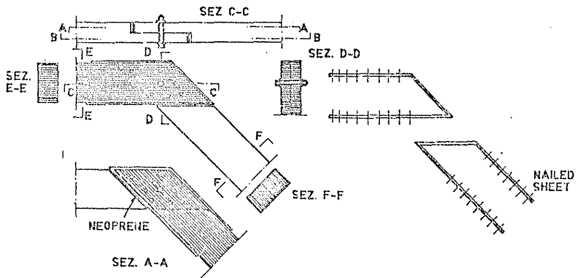
FIG. 8) EXAMPLE OF BOLTED-NAILED JOINT WITH DISSIPATIVE CAPACITY
