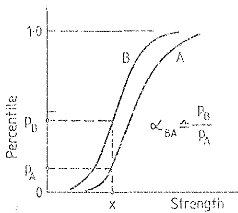
(a) Factor \alpha_{BA}
