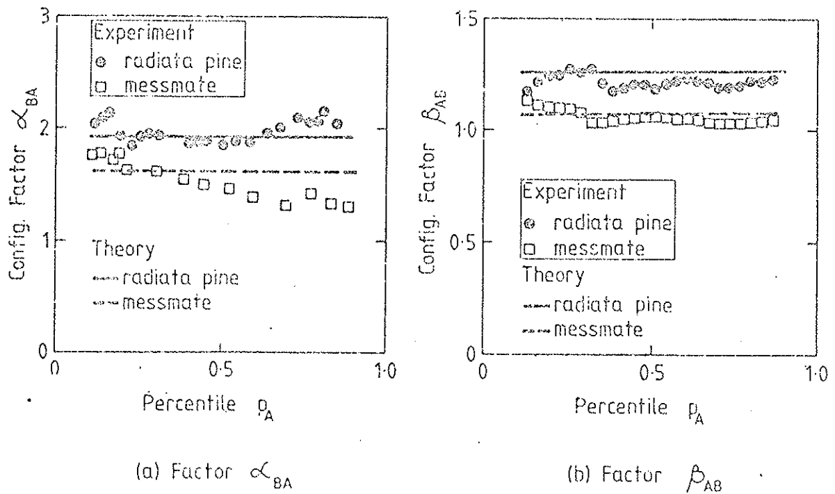
Figure 4. Configuration factors for effect of loaded length Configuration A: loaded length = L Configuration B: loaded length = 2L
