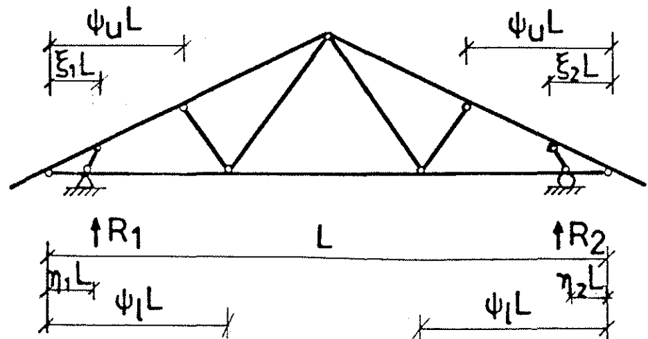
Figure 3. Notations introduced for geometry and support reactions.
