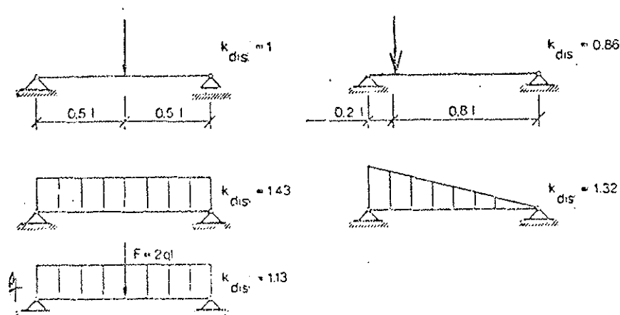
Figure 5.1.7 b. Examples on k_{dist,v}
