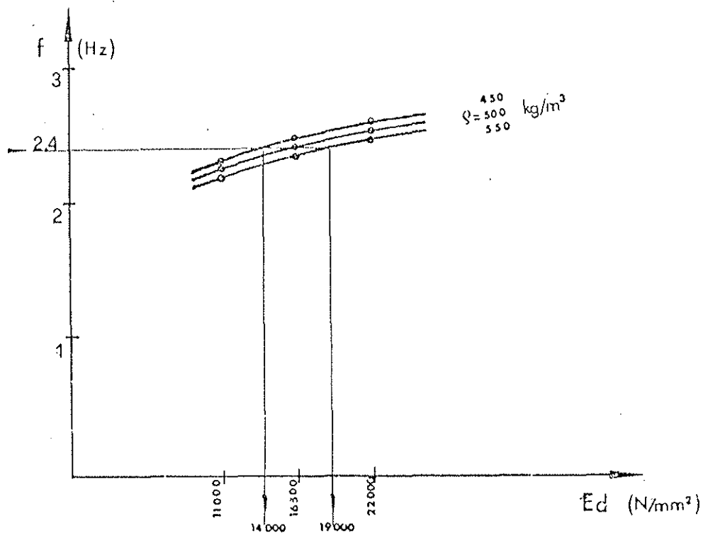
Fig. 7 - The frequencies of the modal shapes like the experimental shape, versus the dynamic elastic modulus ( E_d ) and the density mass of timber ( \rho ).
