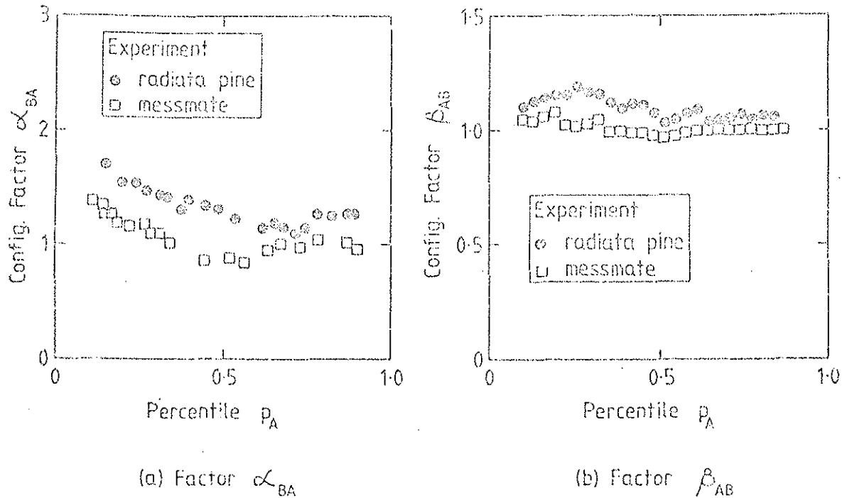
Figure 5. Configuration factors for the effect of edge bias Configuration A: grading defect on tension edge Configuration B: grading defect on random edge
