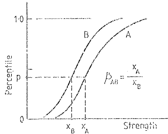
(b) Factor \beta_{AB}
