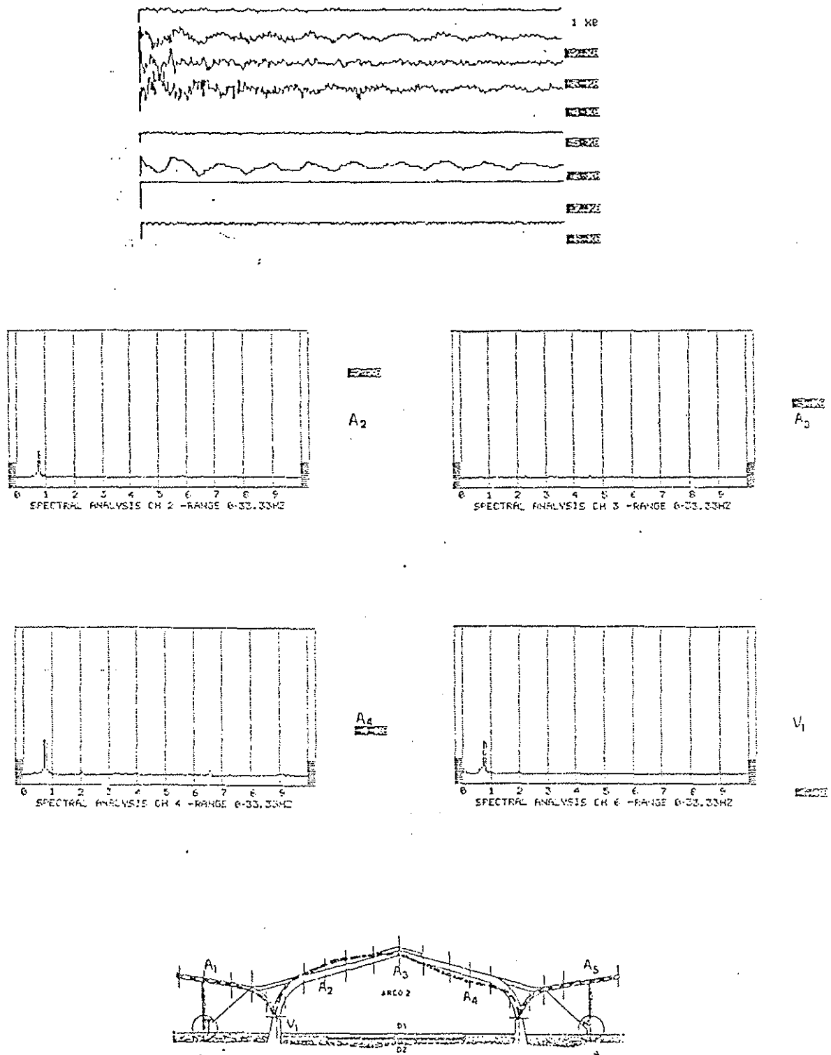
Fig. 3 - Vertical tests: impulse of a quarter of the span. The frequencies detected in several measuring points have the same value: the excited "mode" of vibration has a frequency of about 2,4 Hz; the modal shape is similar to the 3rd theoretical mode.
