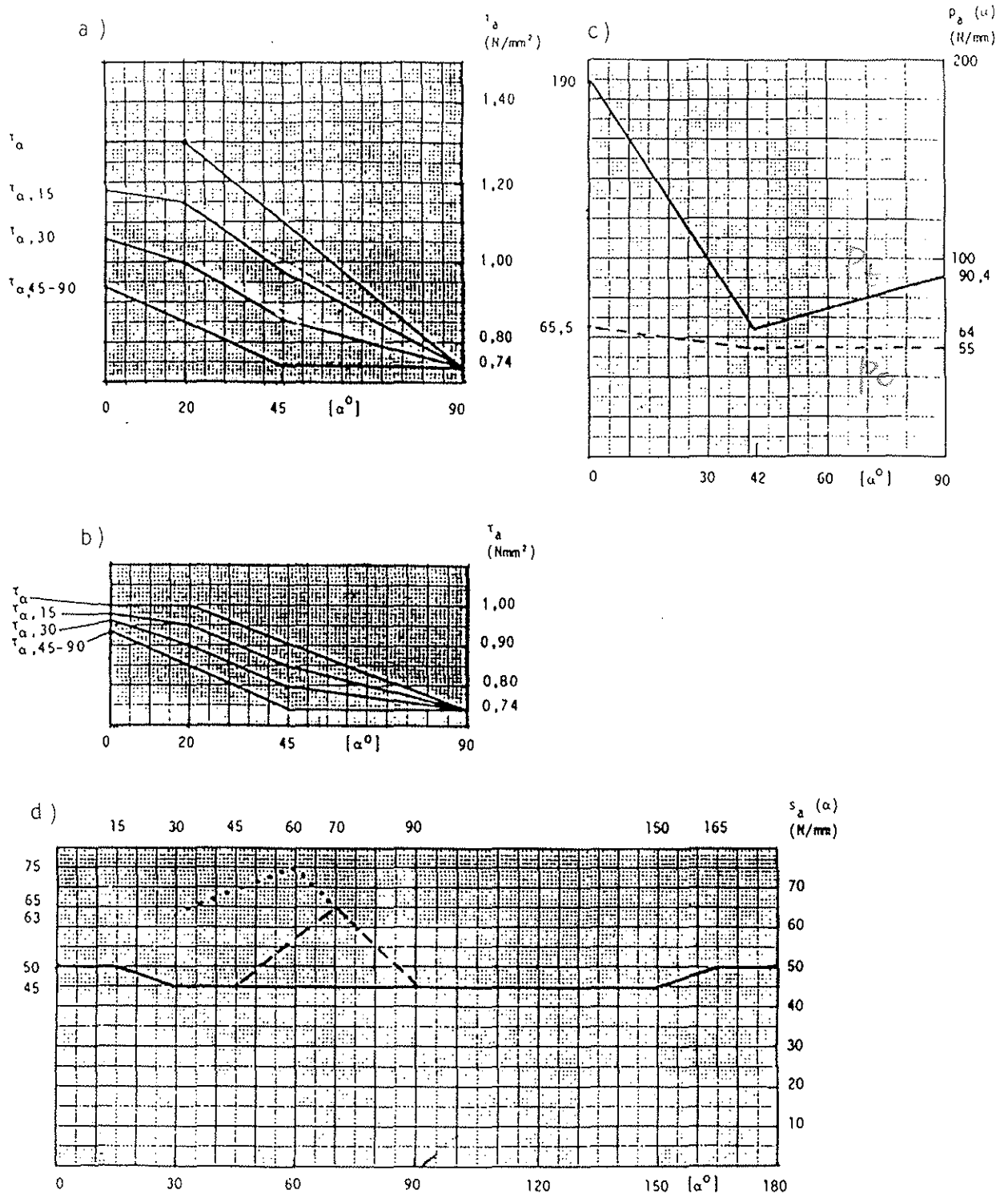
Figure 2. Examples of the allowed strength values of nailplate joints
