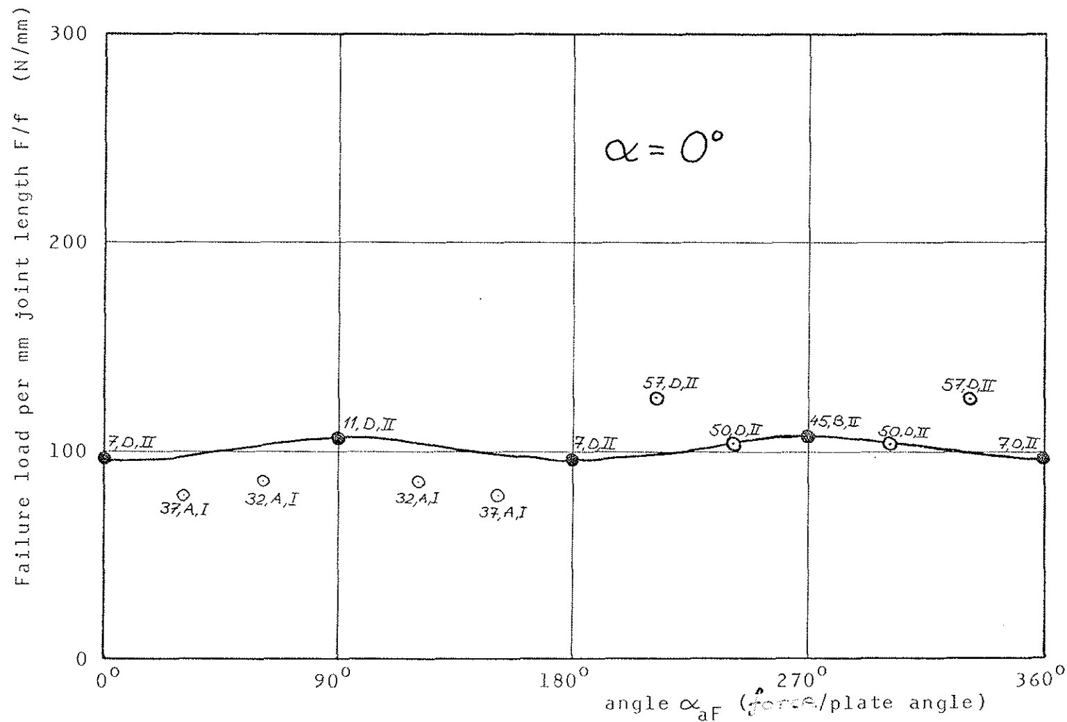
Figure 9. Test results for \alpha = 0^\circ and various angles of \alpha_{aF} . Results below design curve were due to anchorage failure.
