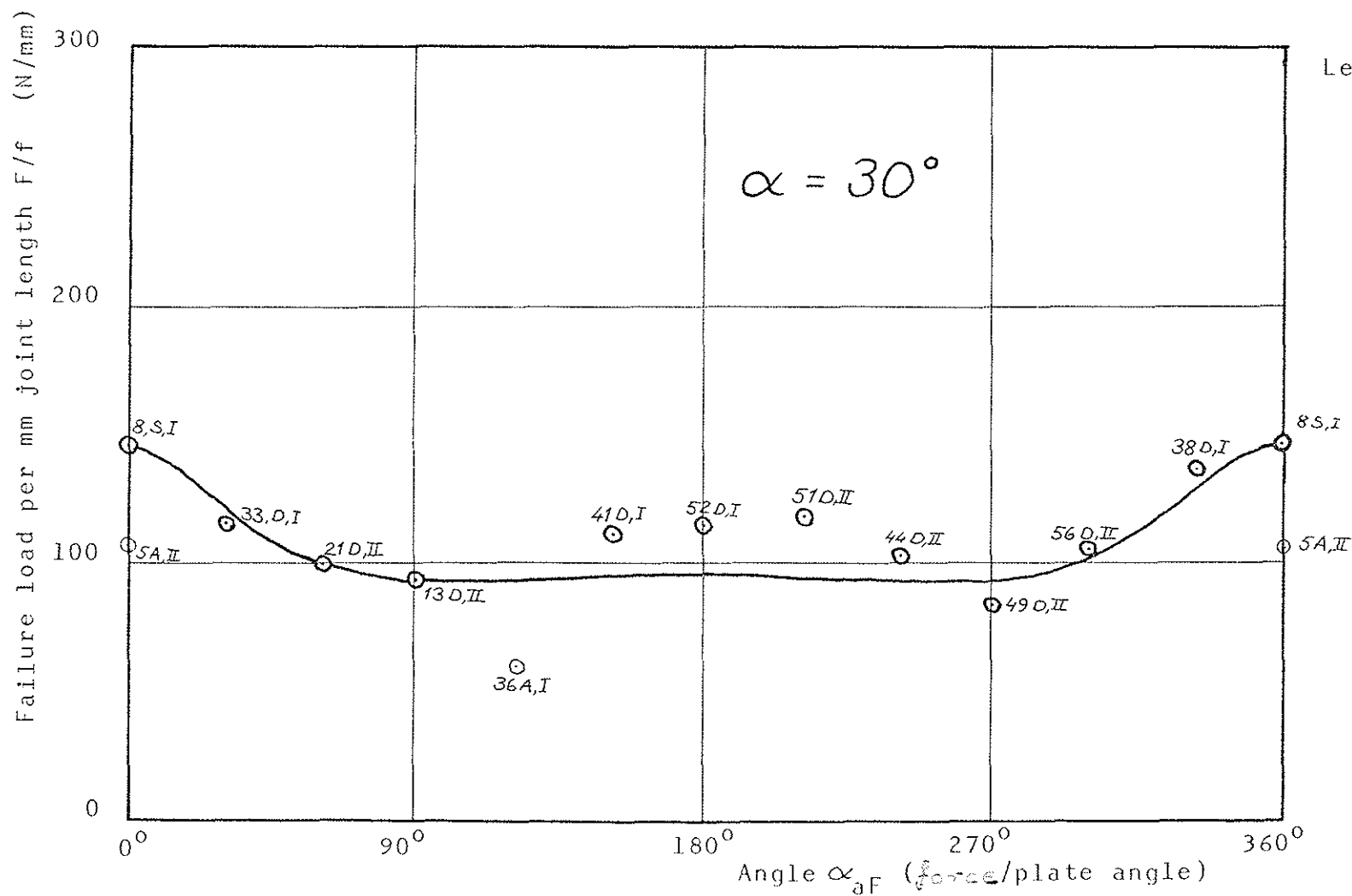
Figure 10. Test results for \alpha=30^\circ and various angles of \alpha_F .
