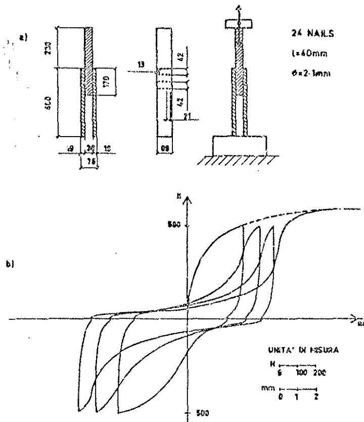
FIG. 7) TEST ON NAILED JOINTS UNDER CYCLIC LOAD: a) DIAGRAM OF TEST SET-UP; b) TYPICAL EXPERIMENTAL PLOT; AFTER DI IORIO, 1984.
