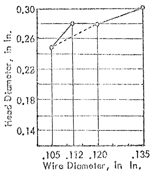
Fig. 3.- Relationship between head diameter and wire diameter of standard pallet-assembly nails.
