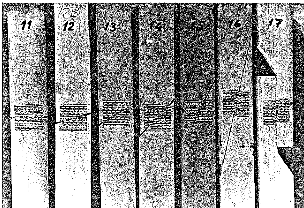
Figure 8. Failure modes from testing of plate strength in b-direction. For all tests failure loads are almost equal and failure involves the same mechanism of yielding hinges.
