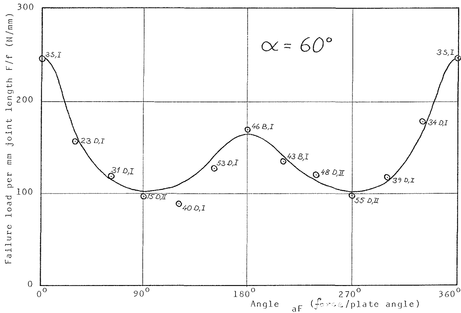
Figure 11. Test results for \alpha = 60^\circ and various angles of \alpha_F .
