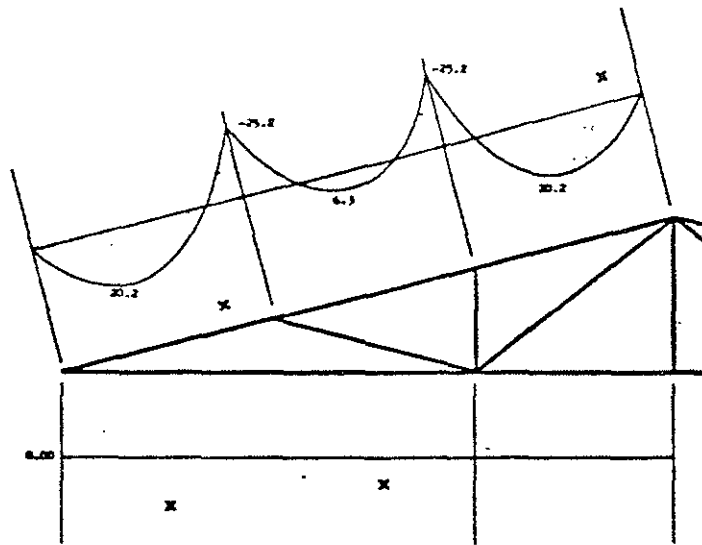
Fig. 4. Pinned connections, continuous beam analysis, eccentricities excluded.
