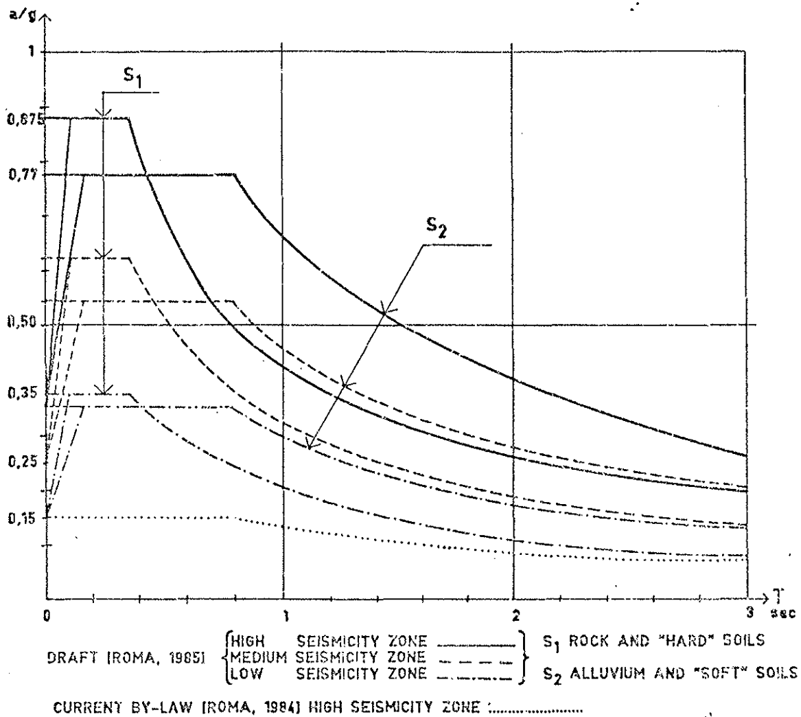
FIG. 5) ACCELERATION DESIGN SPECTRA OF ITALIAN SEISMIC RULES
