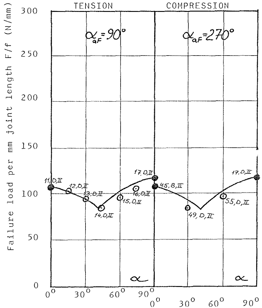
Figure 5b) Results from test of plate-strength in b-direction.
