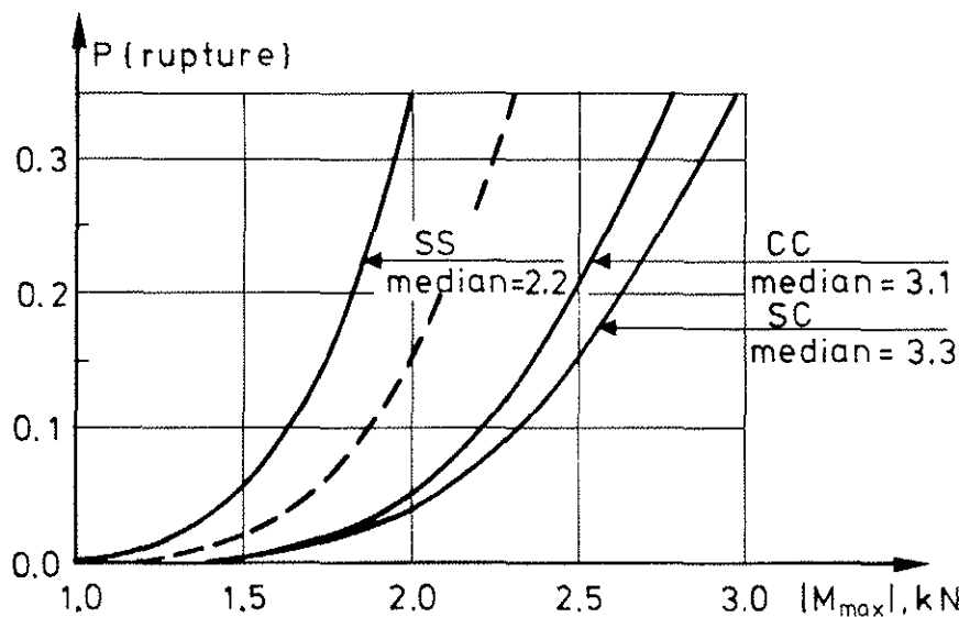
Figure 2.2 Cumulative distribution functions for timber beams with different supports. The dotted line represents F_d .
