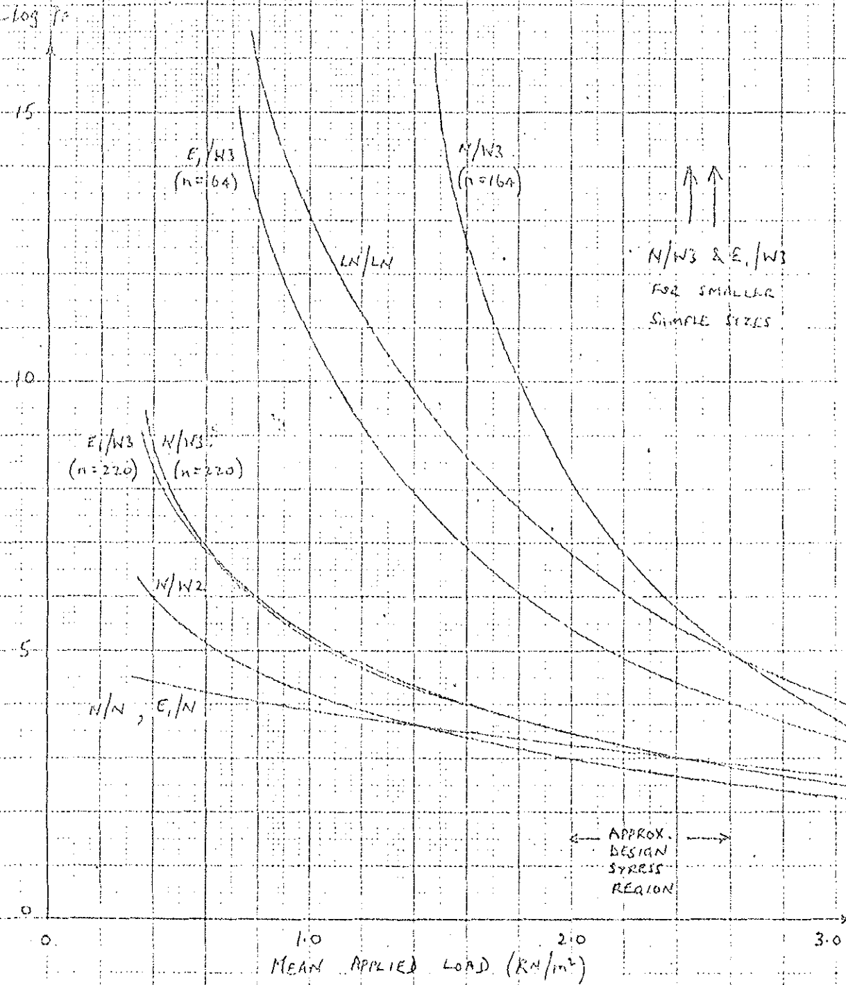
FIG 14 COMPARISON OF LONG-TERM FAILURE PROBABILITIES SHOWING HOW E_i/W3 AND N/W3 ARE AFFECTED BY SAMPLE SIZE
