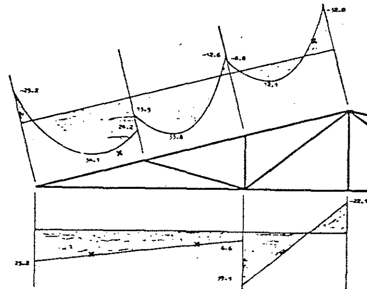
Fig. 7. Stiff connections, frame analysis, eccentricities included appr.
