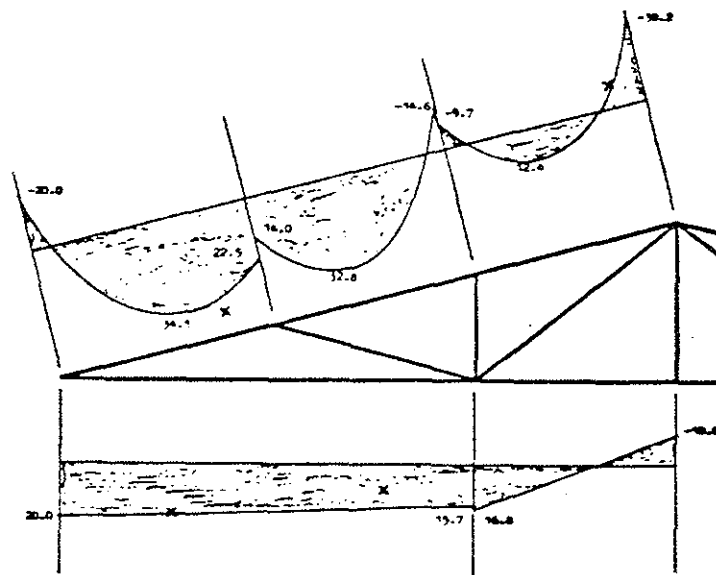
Fig. 6. Stiff connections, frame analysis, eccentricities excluded.
