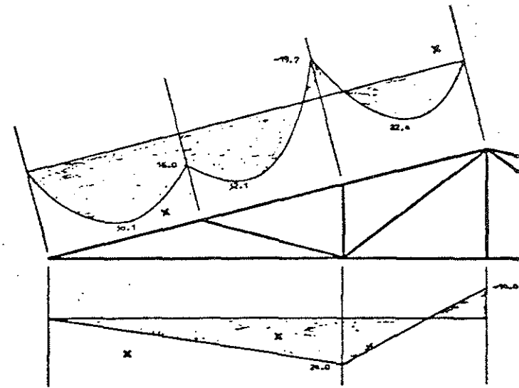
Fig. 5. Pinned connections, frame analysis, eccentricities excluded.
