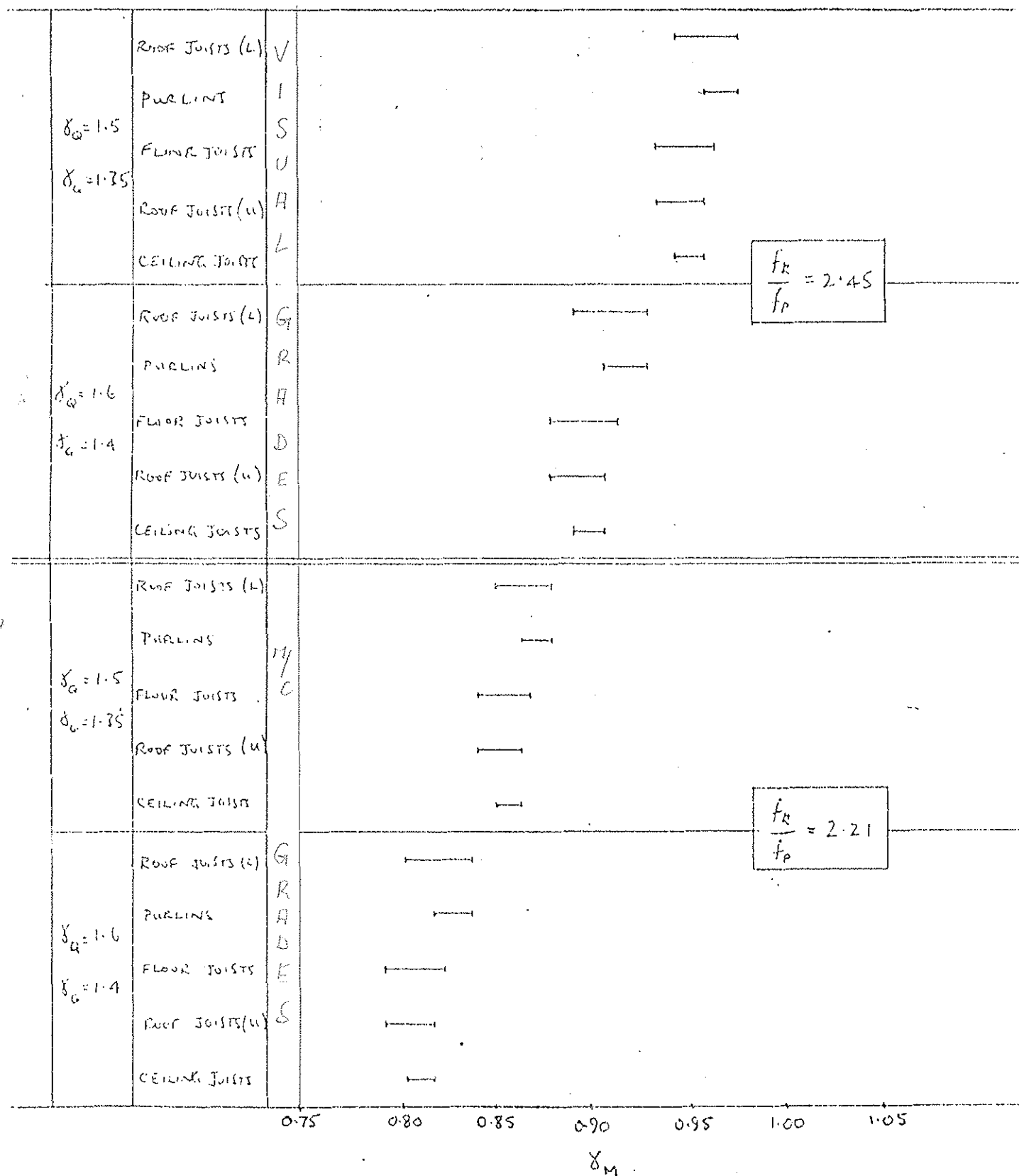
FIG 5 VALUES OF \delta_M FOR BENDING
