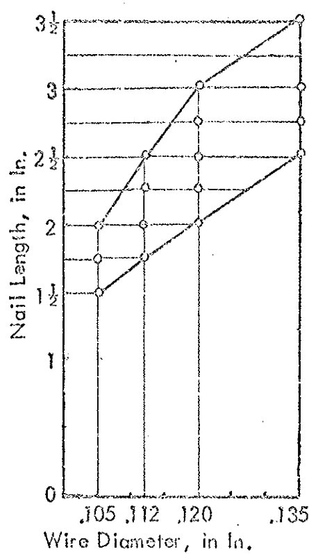
Fig. 1.- Standard pallet-assembly nails, helically threaded, stiff-stock or hardened steel.
