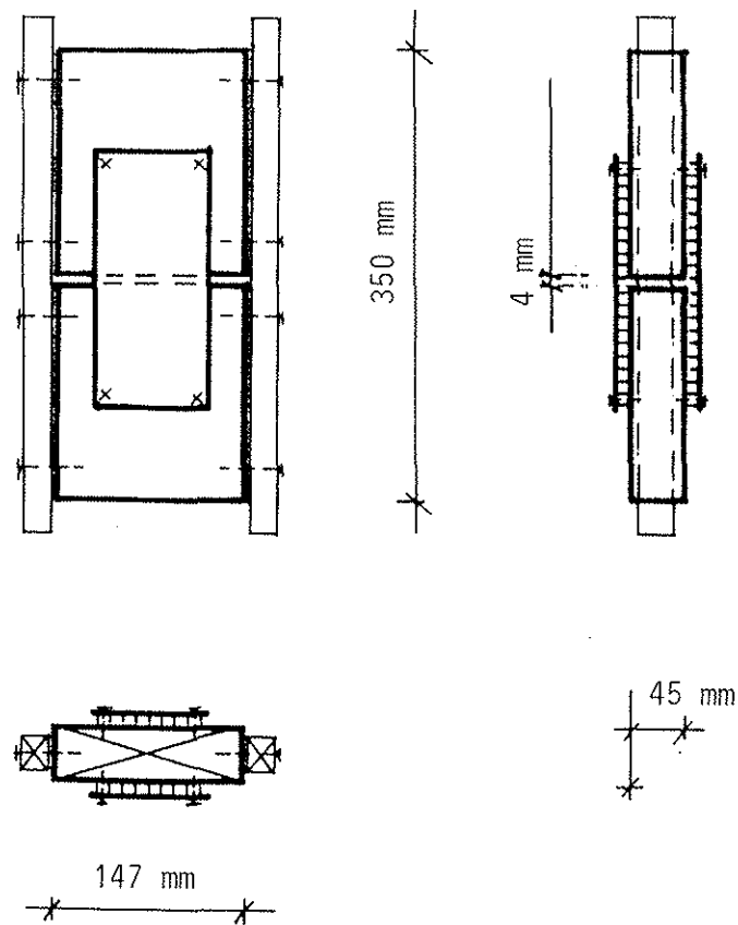
Figure 3. Compression test specimen with strips of wood for facilitating assembling.
