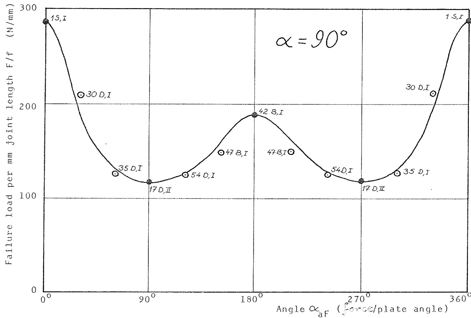
Figure 12. Test results for \alpha = 90^\circ and various angles of \alpha_{aF} .
