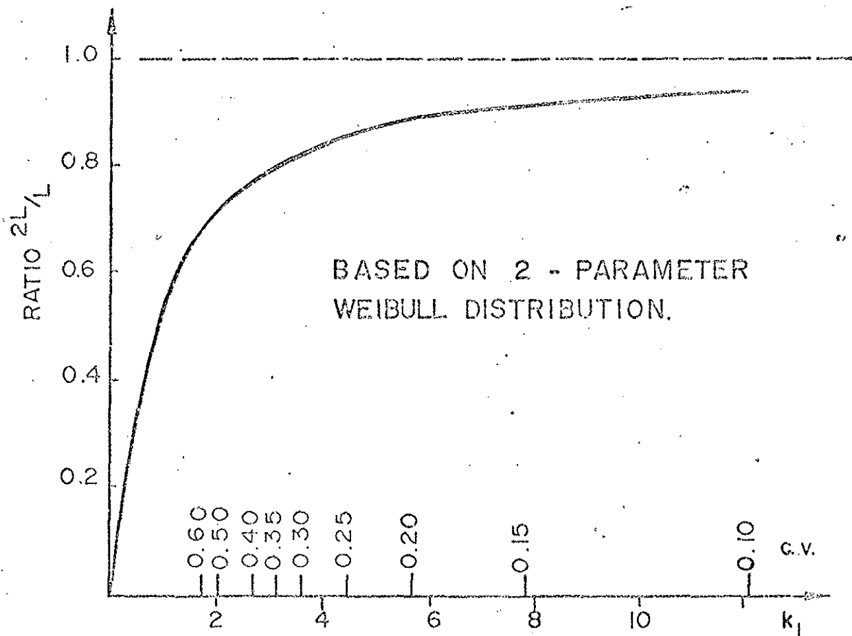
FIG 2. STRENGTH AFTER DOUBLING LENGTH AS FUNCTION OF k_l
