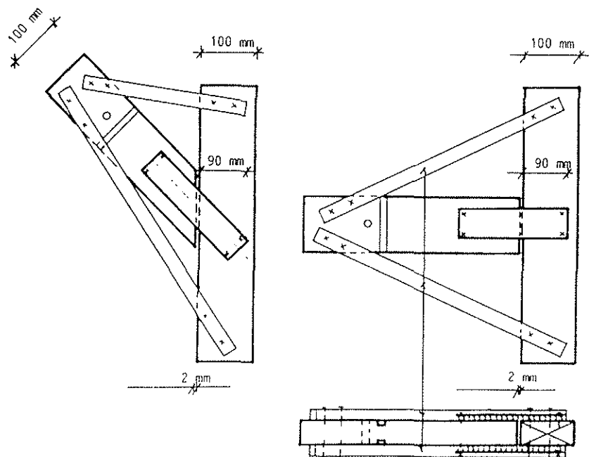
Figure 2. T-joint sepecimens with strips of wood for facilitating assembling a) \tau_{0.90} and \tau_{90.90} b) \tau_{0.45}
