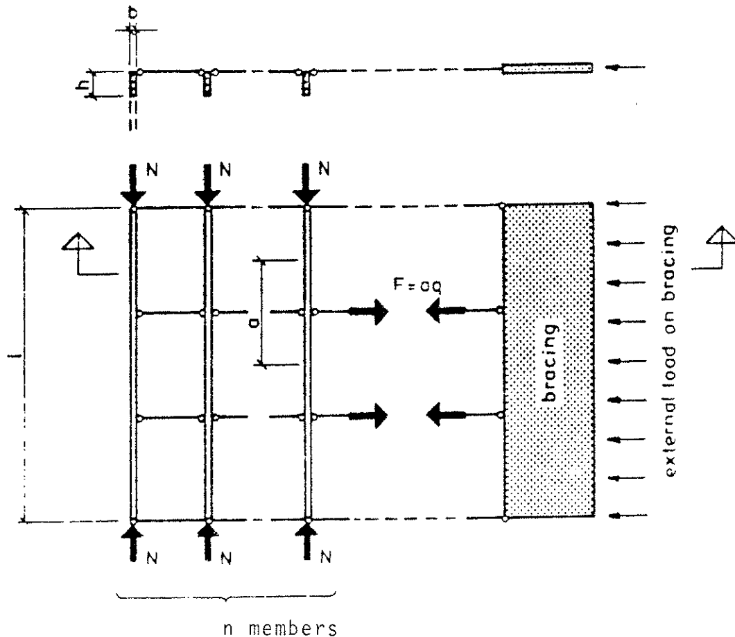
Fig. 1: Bracing System
