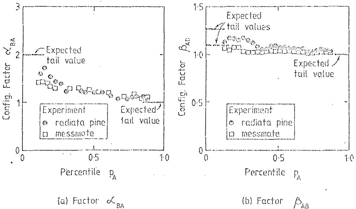
Figure 6. Configuration factors for the effect of stick length Configuration A: stick length is full stick Configuration B: stick length is half stick
