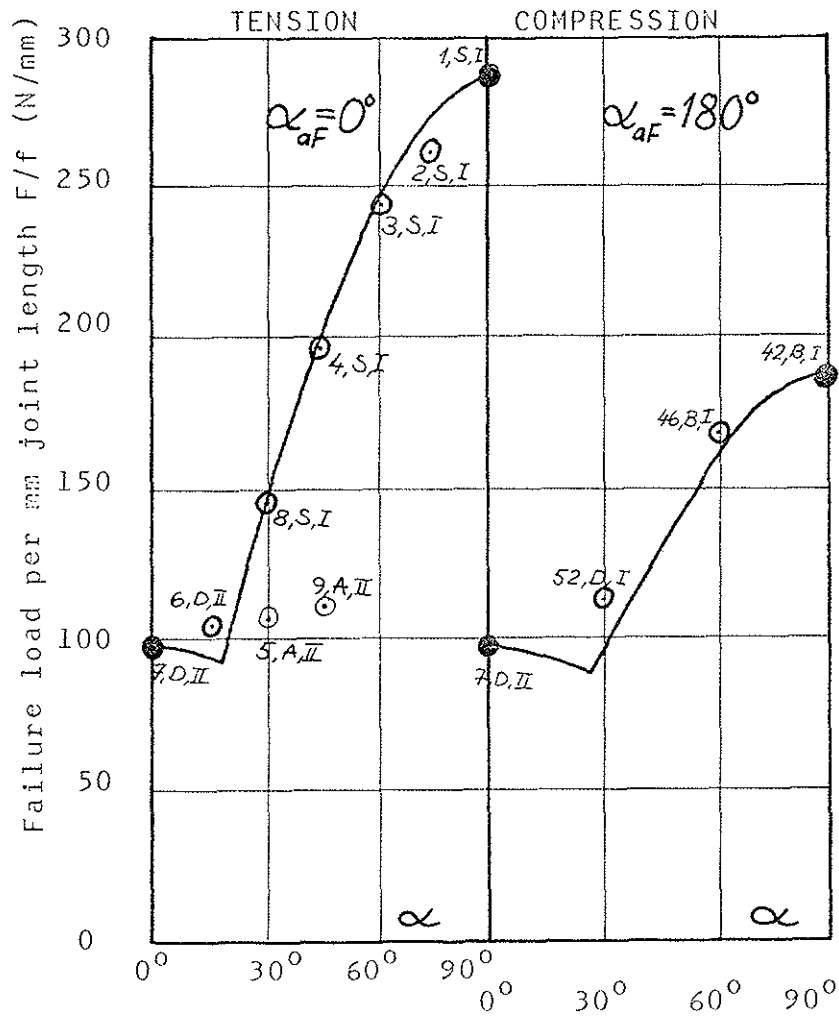
Figure 5a) Results from test of plate-strength in a-direction.
