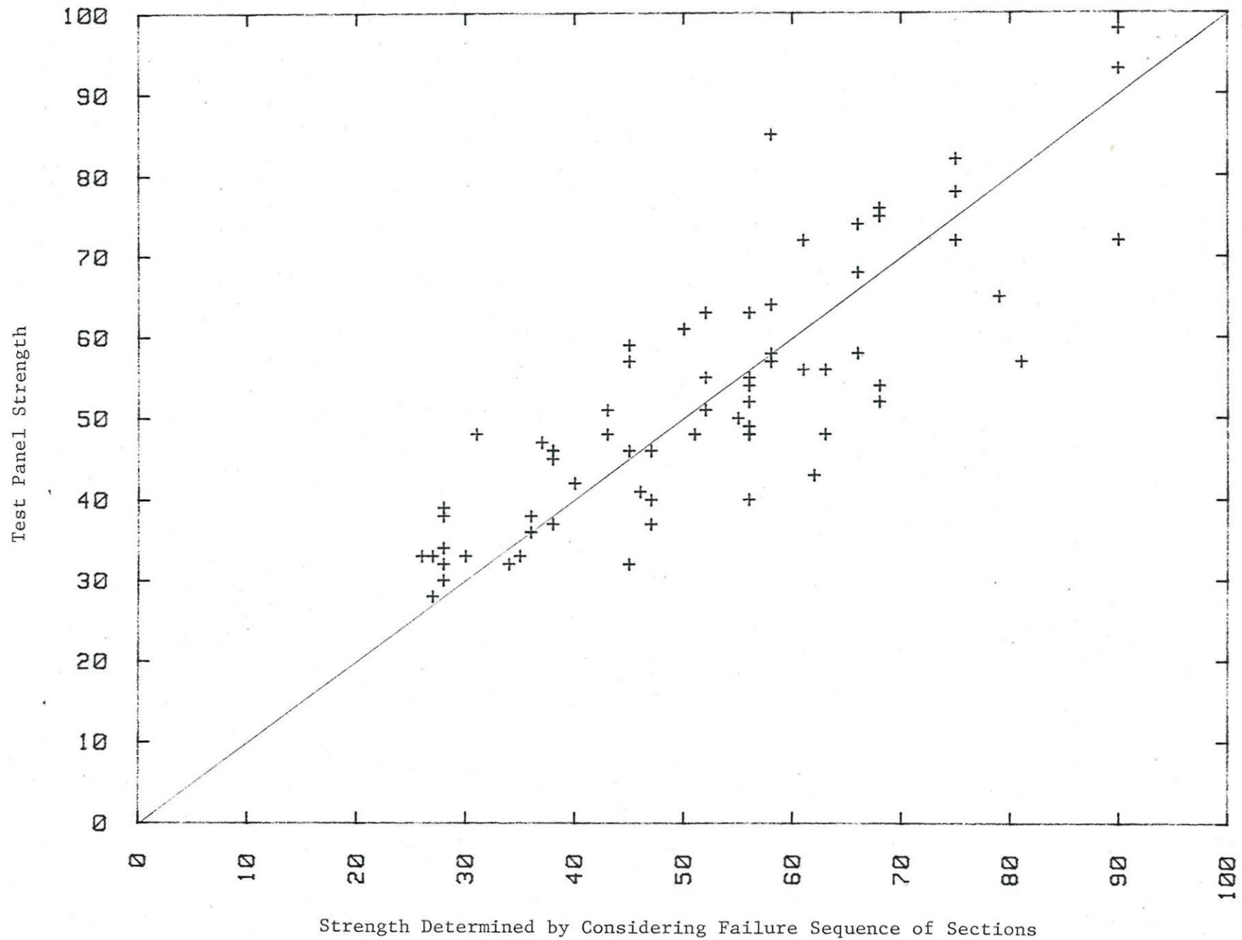
Figure 7. Relationship of estimated to observed strength ratio when estimated ratio considers failure sequence.
