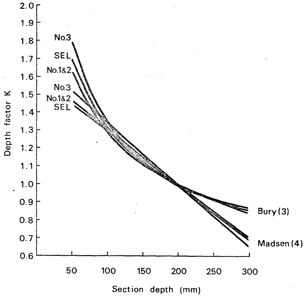
Fig.2. Comparison of grade equations.
