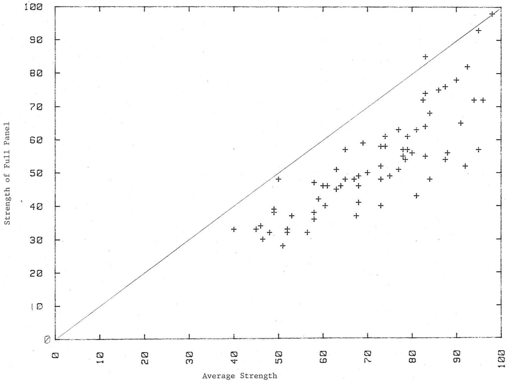
Figure 3. Relationship of average strength of strips to test strength of full panel.
