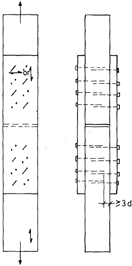
Fig. 5. Sheet material to wood single shear specimen.
