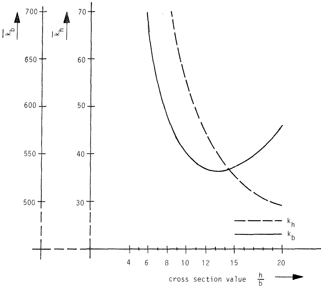
Fig. 5 Coeff. \bar{k}_h and \bar{k}_b in relationship of the cross section quotient h/b ( \beta_V=500 , \beta_F=1000 , G/ =40 )
