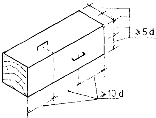
Fig 6 Withdrawal specimen
