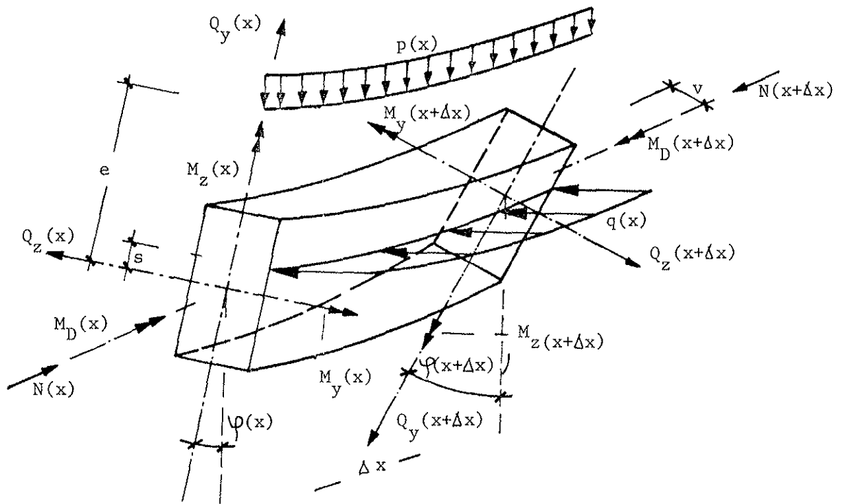
Fig. 2 Sectional forces of a beam element, vertically loaded and laterally supported.
