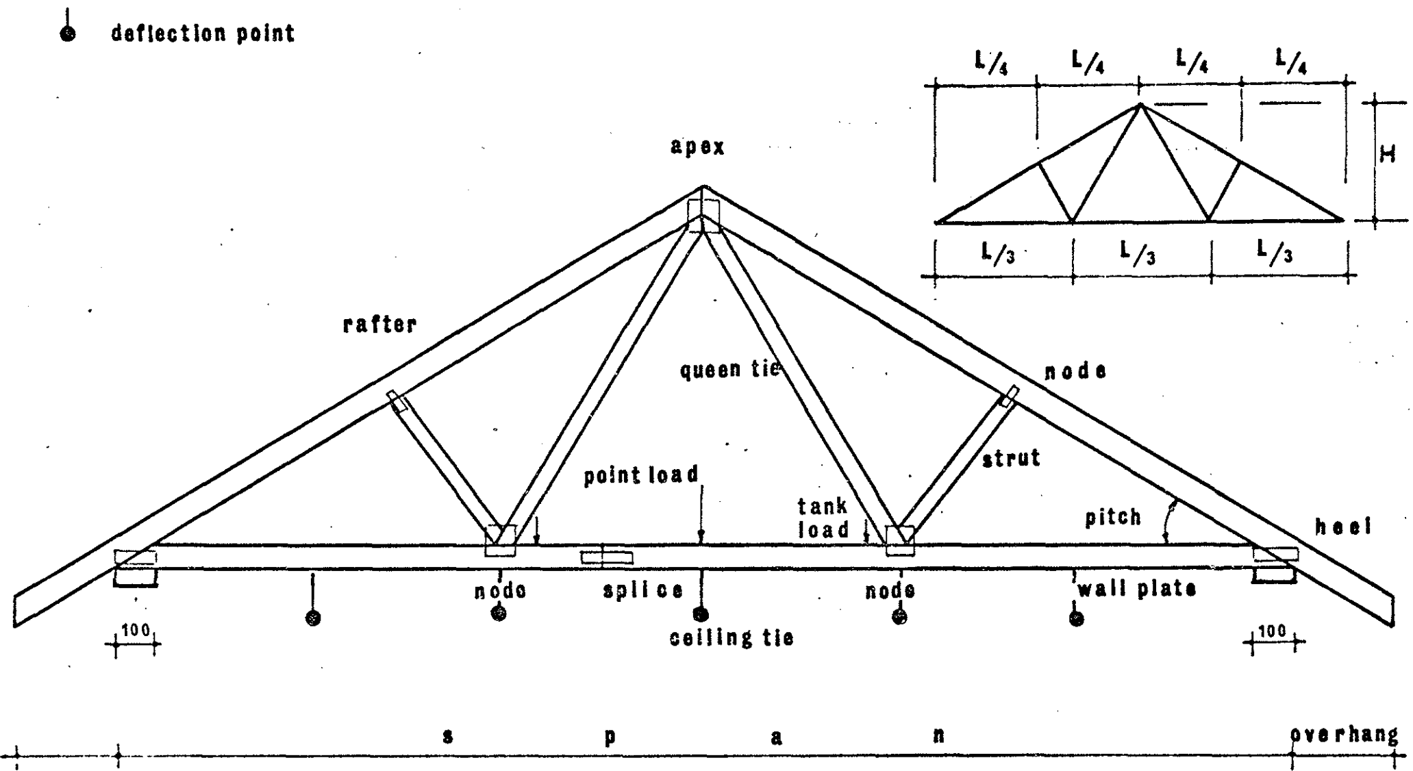
Fig: 1.1 Details of Fink Trussed Rafter
