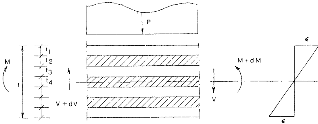
Fig. 1 Strain Distribution due to Bending
