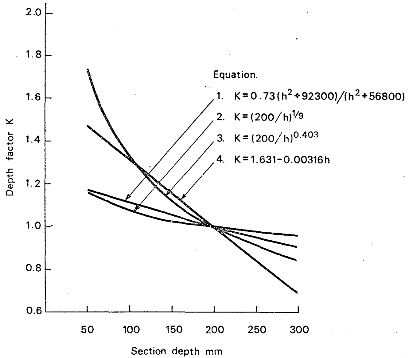
Fig.1. Effect of depth on bending stress.
