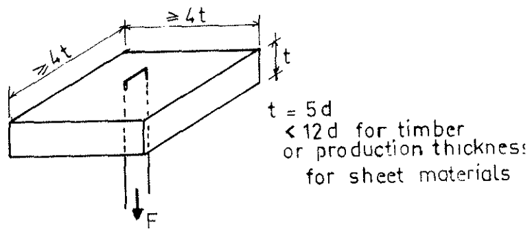
Fig 7 Pull-through specimen
