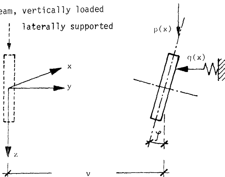
Fig. 1 Laterally supported system
