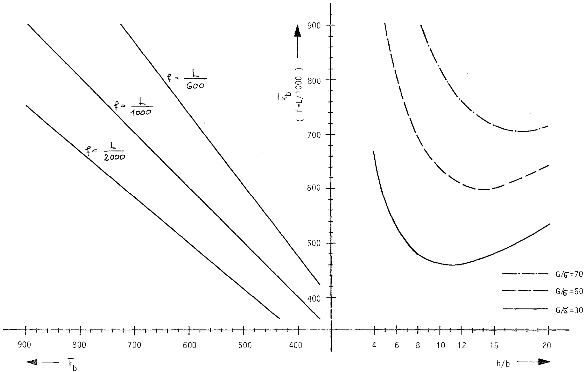
Fig. 6 Coeff. \bar{k}_b as a function of the ratios h/b , G/\sigma and the bracing deformation f ( initial deflection \bar{v}=L/500 )
