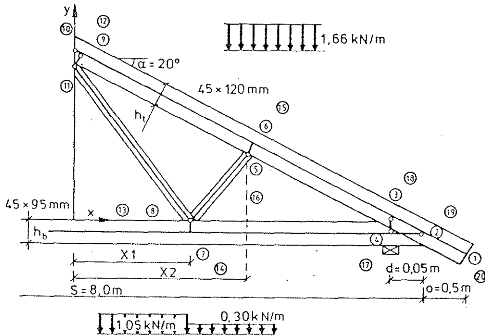
Frame Model with distributed loads.
