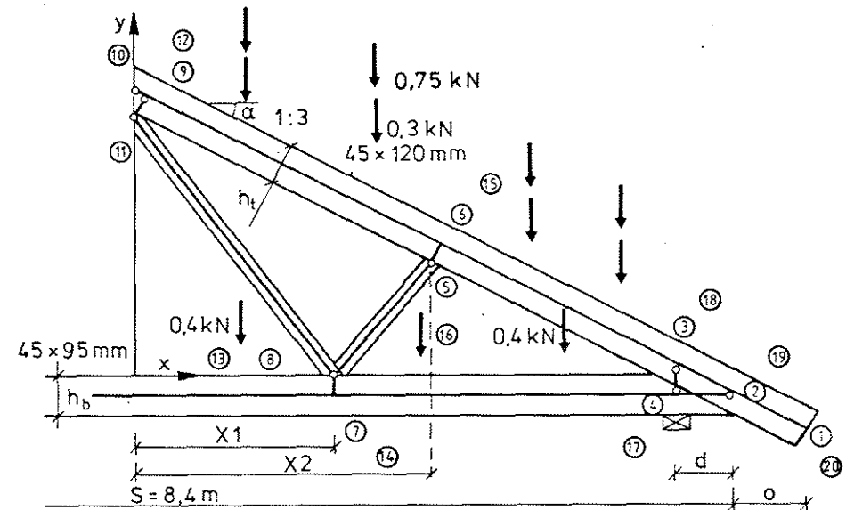
Frame model of wood trussed rafter.
