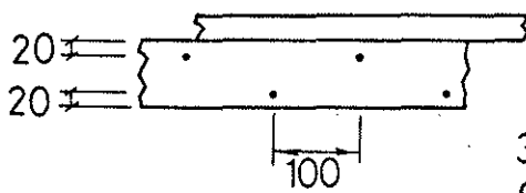
Plan - bracing in ceiling plane
