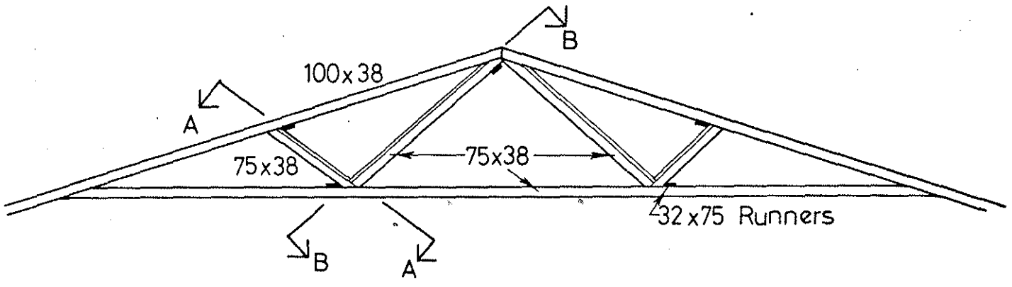
Fink truss
