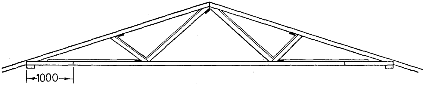
Elevation - Fink truss
