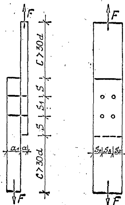
Fig. 2 Sample for determining load carrying ability of asymmetrical joints.
