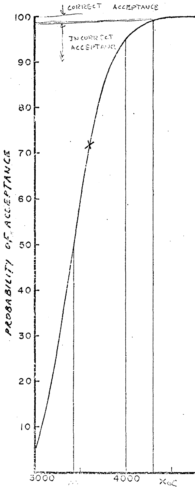
Fig. 1.1 \bar{x} - k_2 s (tolerance limit)
