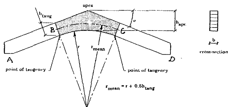
Fig. 5.2.4a Double tapered curved beam
