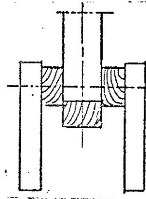
Fig. 6: Rear view of oblique joint
