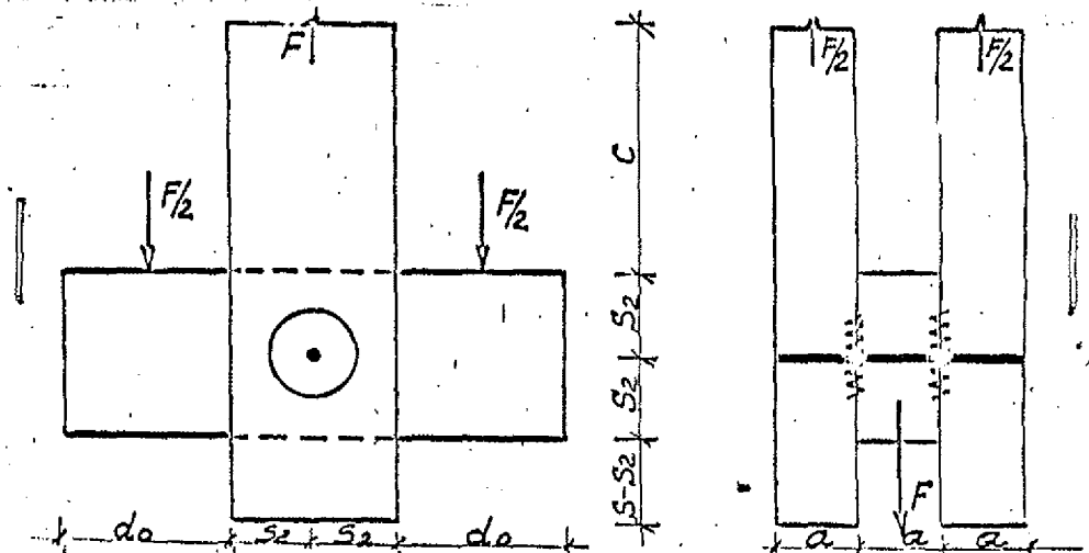
Fig.3 Sample for determination of load carrying ability of rings in direction perpendicular to grain.
