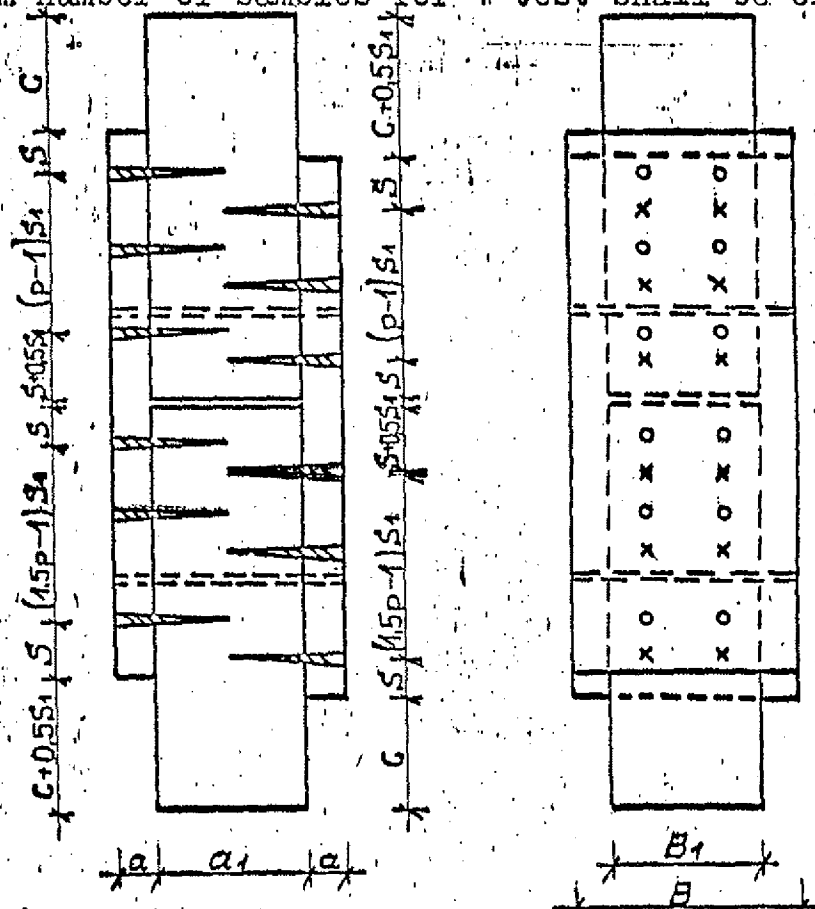
Fig.3 Sample for determination of the effect of connectors number.
