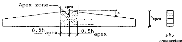
Fig. 5.2.2 b Double tapered beam
