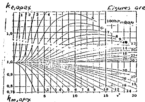
Figure 5.2.4b k_{m, \text{apex}} and k_{t, \text{apex}} for E_{0, \text{mean}}/E_{90, \text{mean}} = 30
