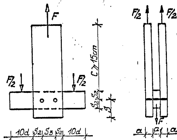
Fig. 4 Sample for determining load carrying ability of bolts and screws in direction perpendicular to grain for d < 10 mm
