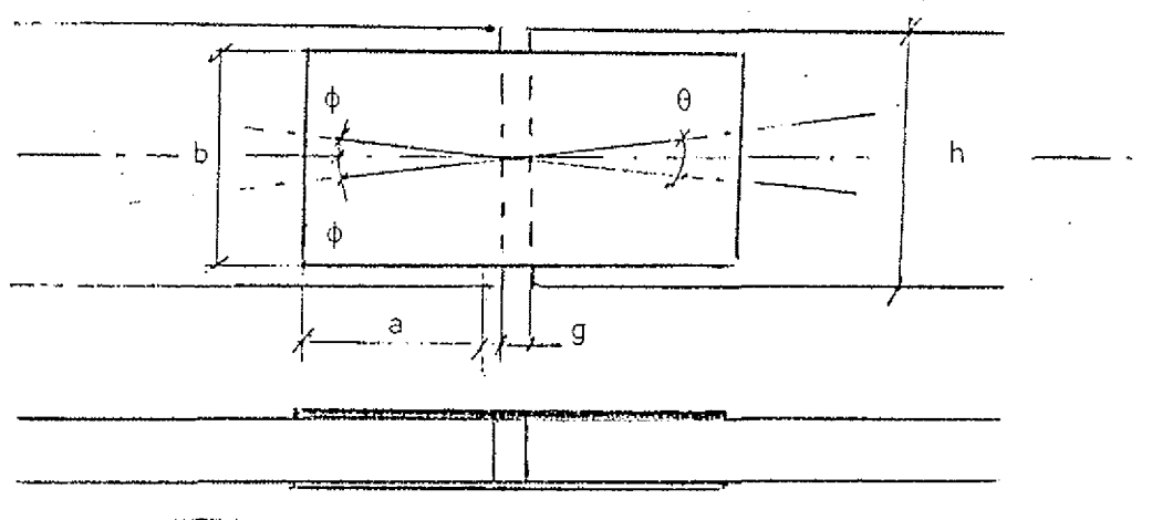
Figure 2:7 Symmetrical splicing with nail plates
