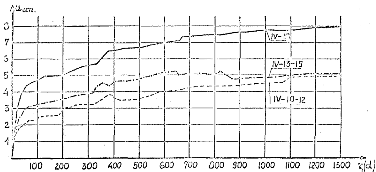
Fig. 7 Time - deflection curve (mean values).
