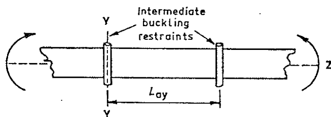
(a) SIDE ELEVATION OF BEAM
