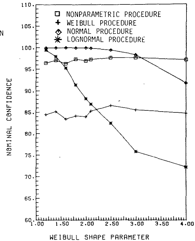
Figure 3. Comparison of procedures when the Weibull distribution is the underlying parent population ( n=70 ). The expected confidence is 95 percent.
