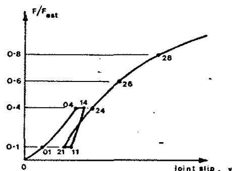
FIGURE 2 - Idealised load-deformation curve and measurements
