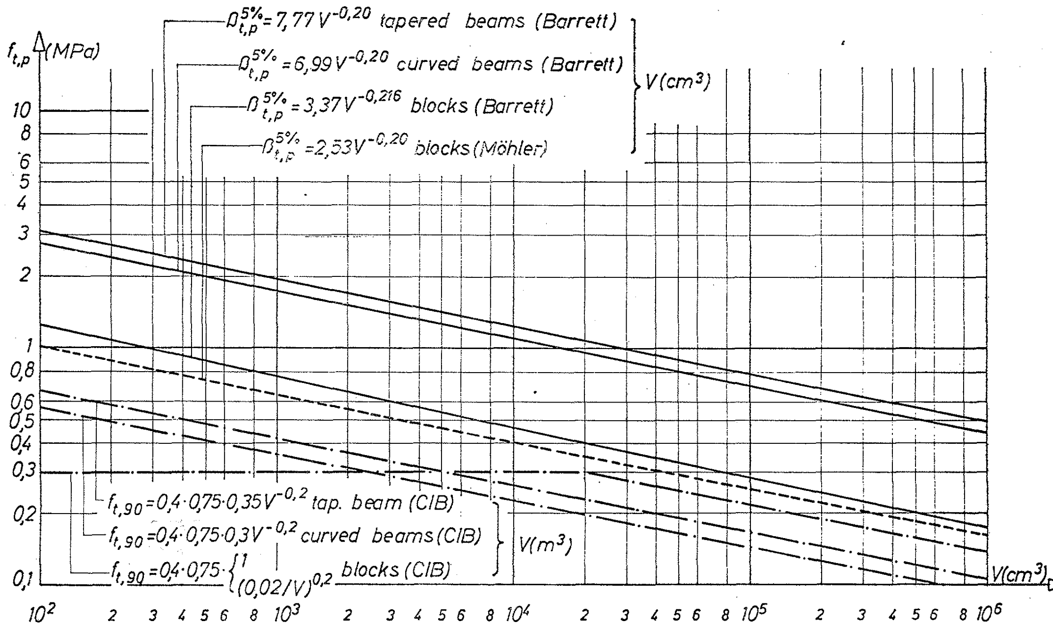
Fig.2 5% values and allowable values for tension stresses perpendicular to grain
