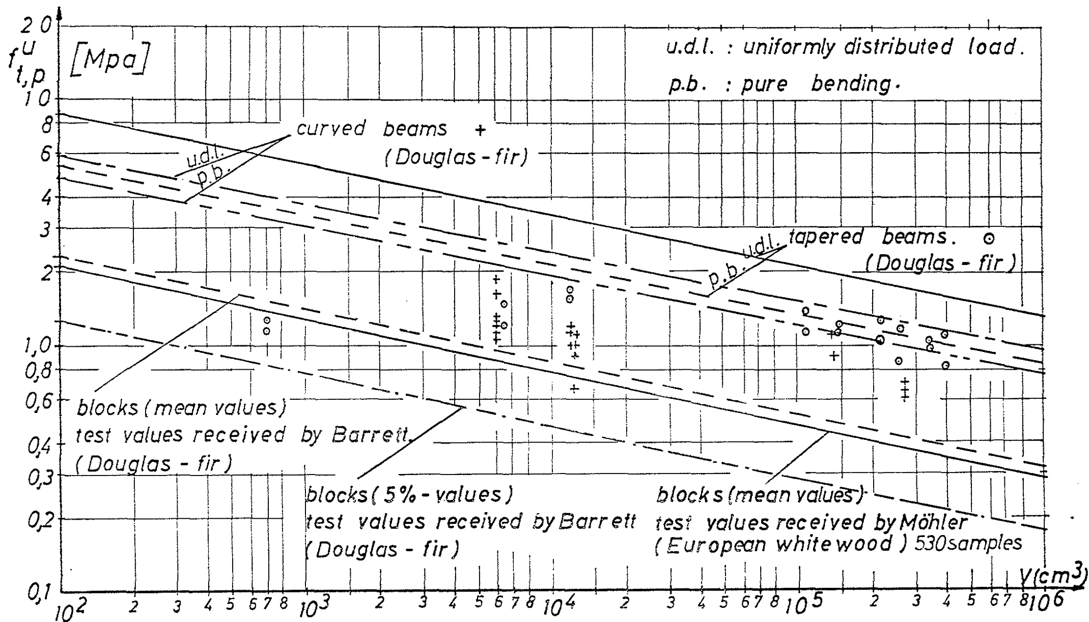
Fig.1 Relation between the tensile strength perpendicular to grain f_{t,p}^U and the volume V
