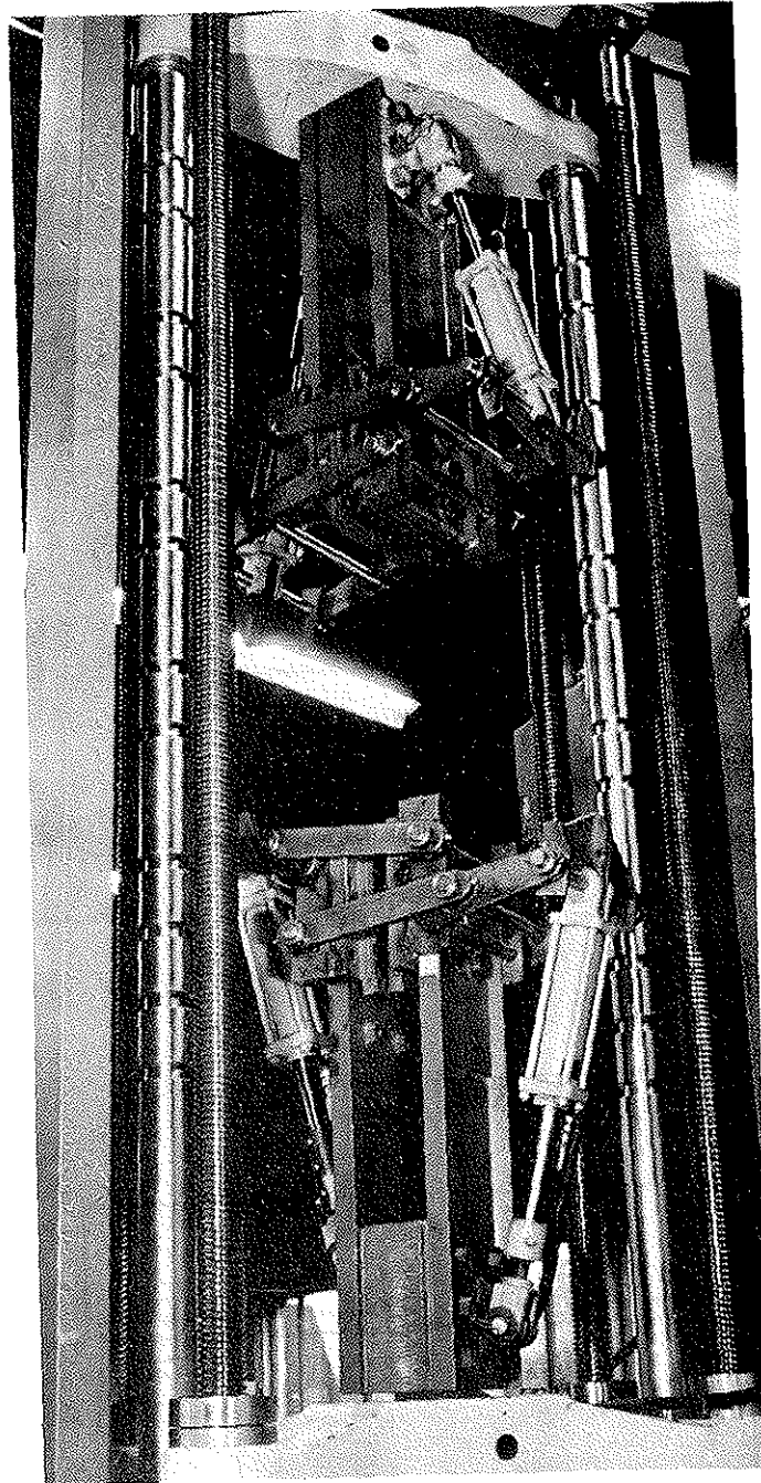
Figure 3 Grips Suitable for Tension Tests
