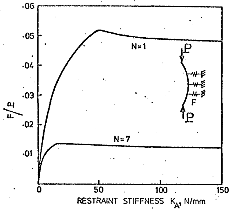
FIG. 3 MAXIMUM RESTRAINT FORCE F AT DESIGN LOAD †
