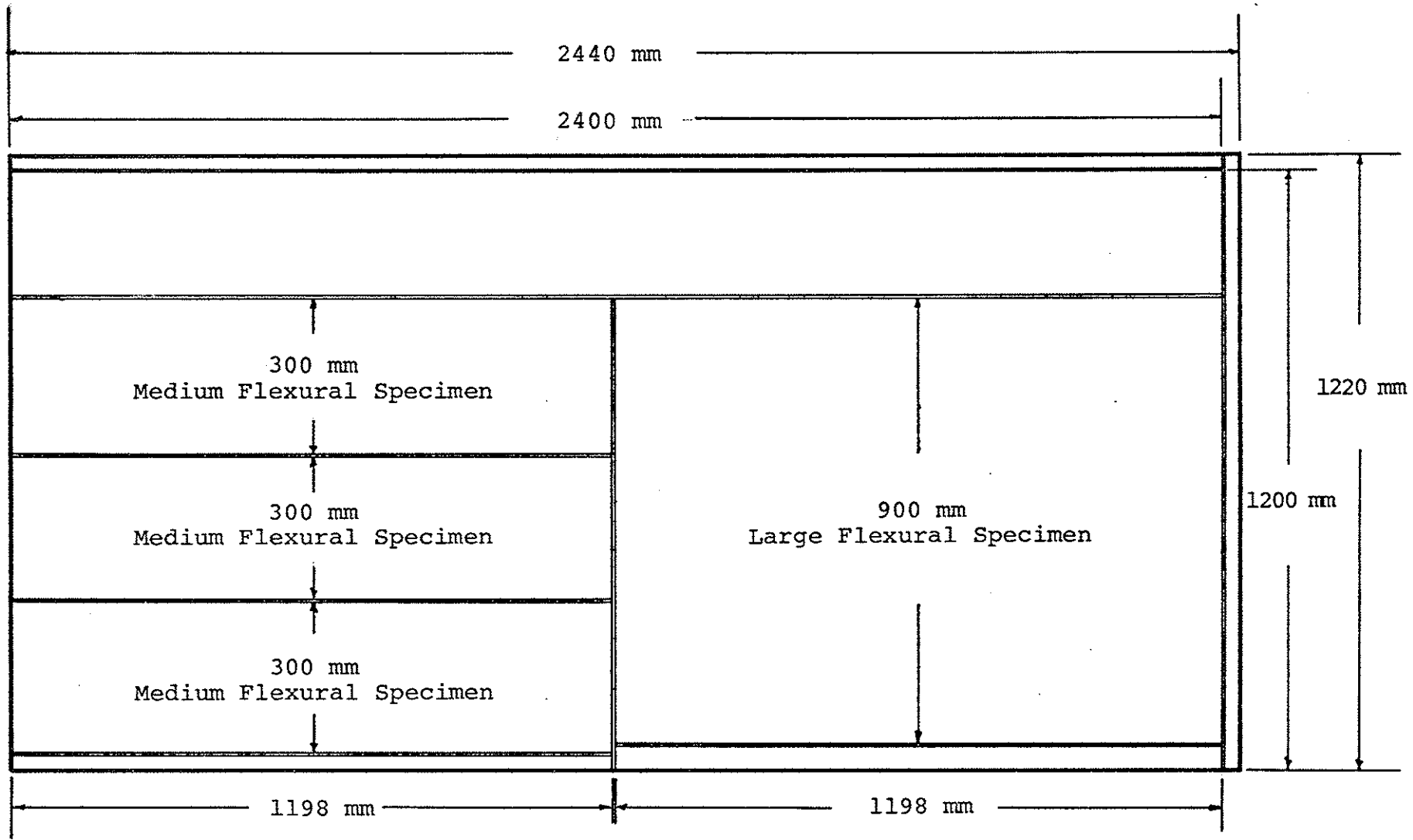
Figure 1. CUTTING PLAN
