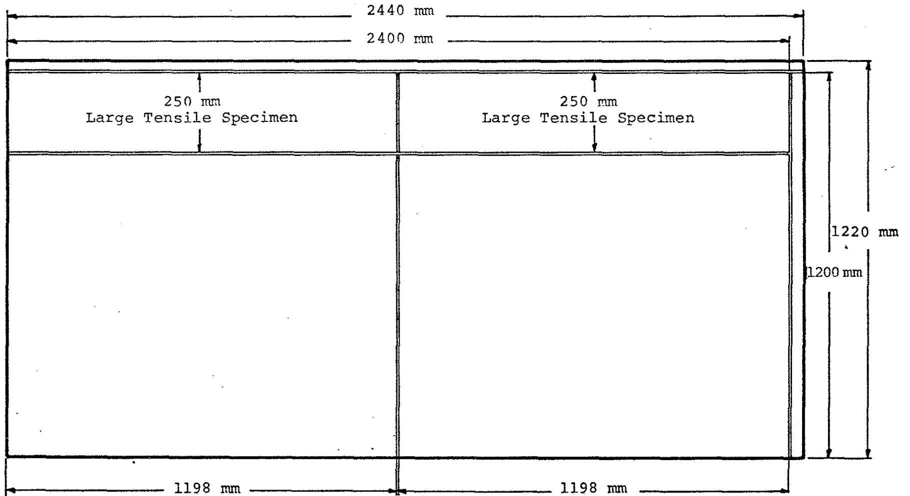
Figure 1. CUTTING PLAN
