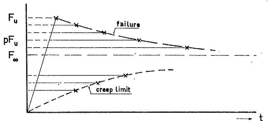
b) active loading followed by constant load at load levels p . At lower loads than F_\infty it is supposed that a creep limit exists after a certain time t .
