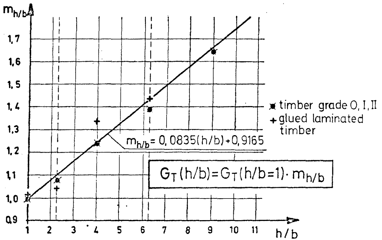
figure 6: influence of the depth to the width ratio to the torsion modulus
