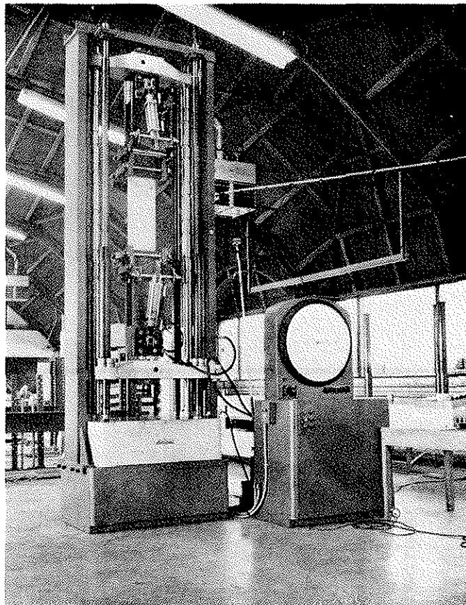
PLATE 1 TENSION TEST
