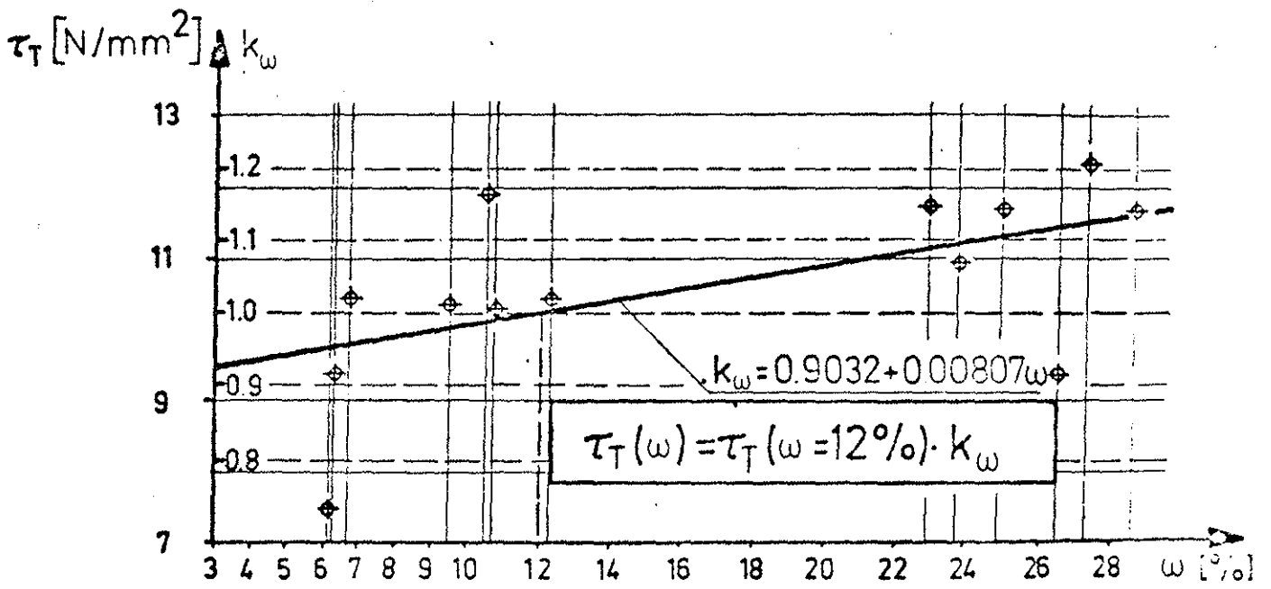
figure 2 : influence of the moisture content to the torsional strength related to \omega = 12\% (test values related to \rho_{12} = 380 \text{ kg/m}^3 )
