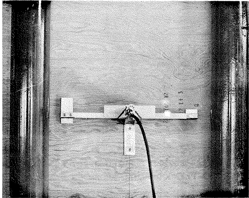
PLATE 2 DEFLECTION MEASURING DEVICE FOR PURE MOMENT FLEXURE TEST
