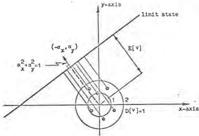
Fig. 2: Illustration of E[v] as being the distance from the origin of the reduced coordinate system to the limit state line. Each point corresponds to a random outcome of (\xi, \eta) , that is, a realization of the loaded structure.
