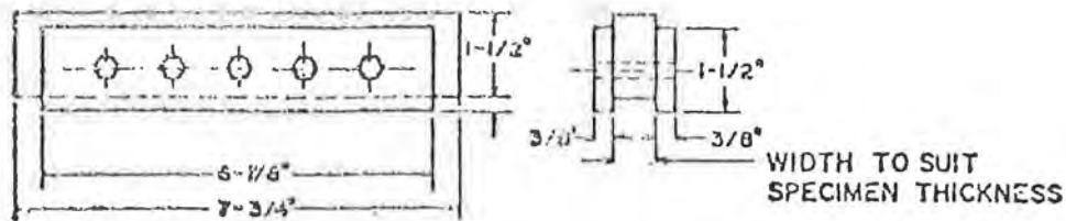
SPECIMEN LOADING BLOCKS 2 REQ'D
