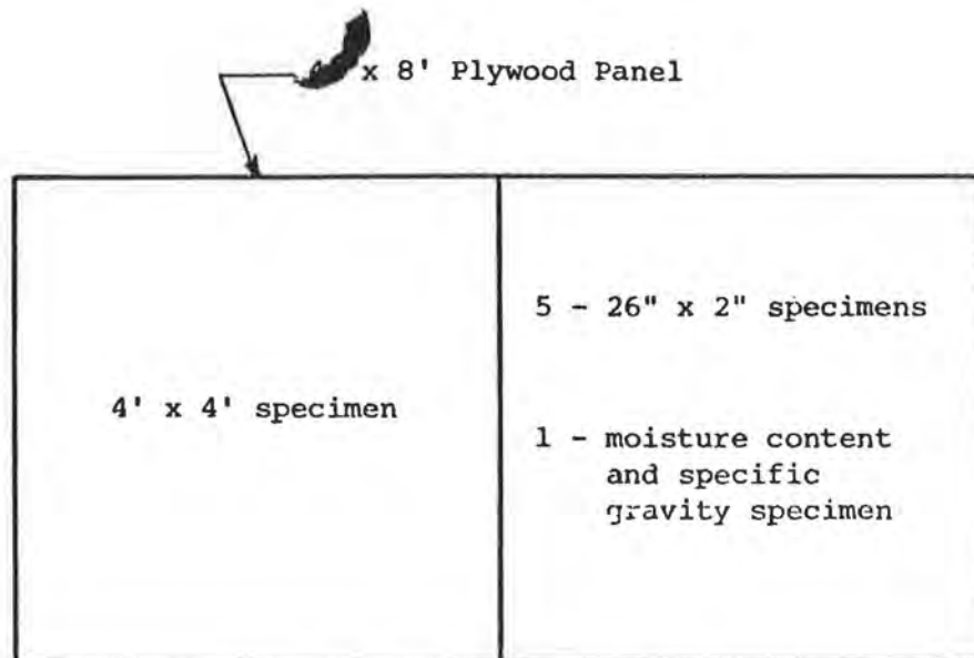
FIGURE 1. CUTTING PLAN
