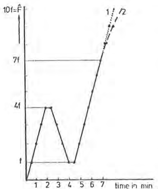
Fig. 1. Loading procedure
