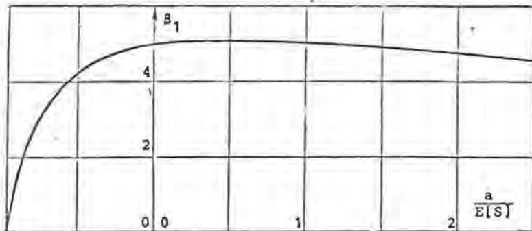
Figure 3. Illustration of translation dependence of the safety index \beta_1 . (Determined for \beta_0 = 5 , V_R = V_S = 0.2 ).
