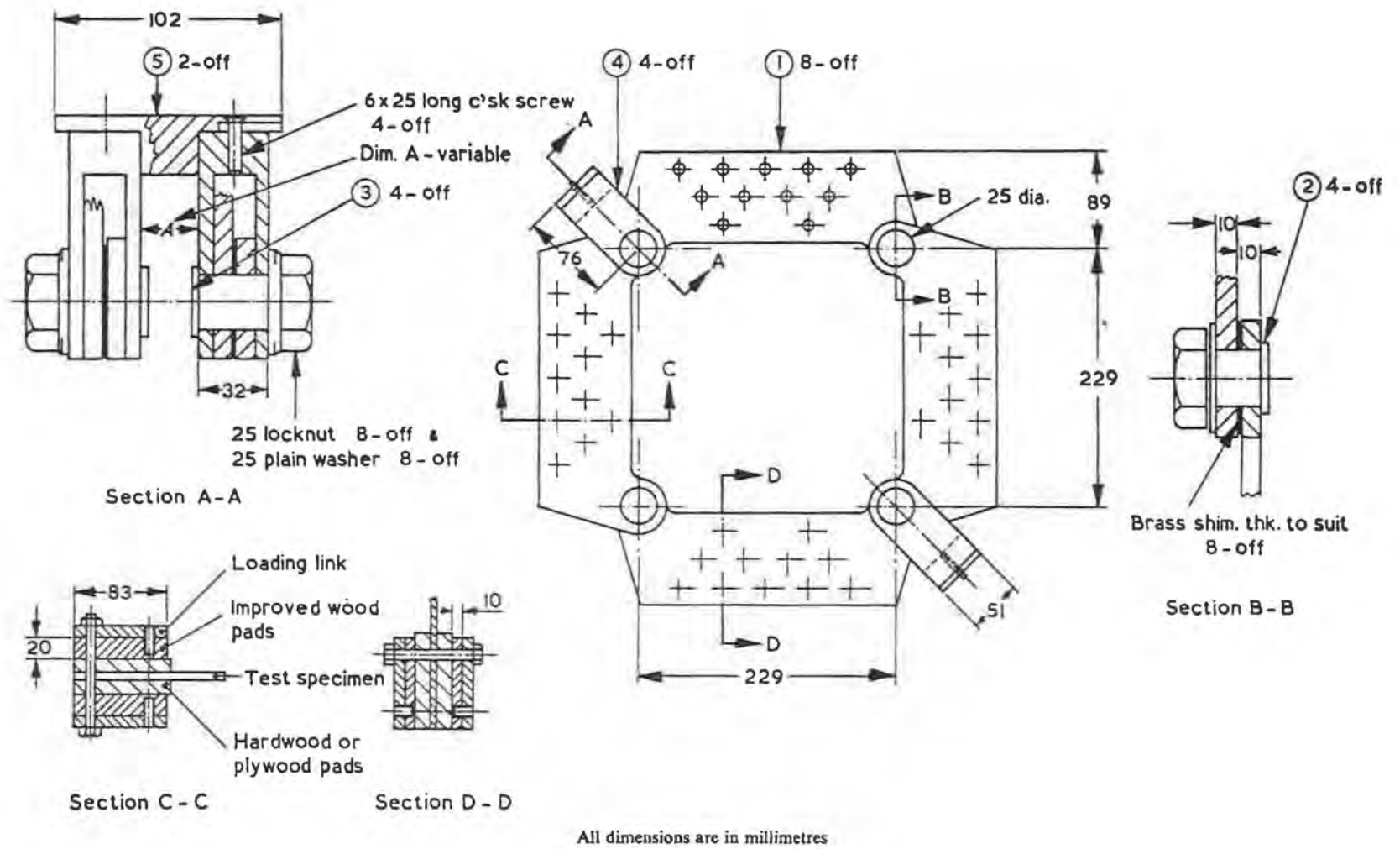
Figure 10 Panel shear apparatus
