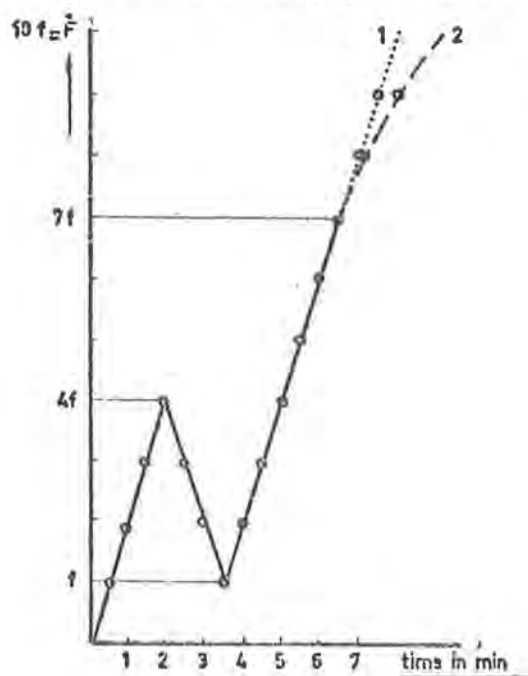
fig. 2 Loading procedure
