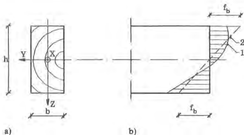
Fig. 3.01. Curve 1 of fig. b) shows the real stress distribution in principle, while curve 2 is the approximation of the theory of elasticity.
