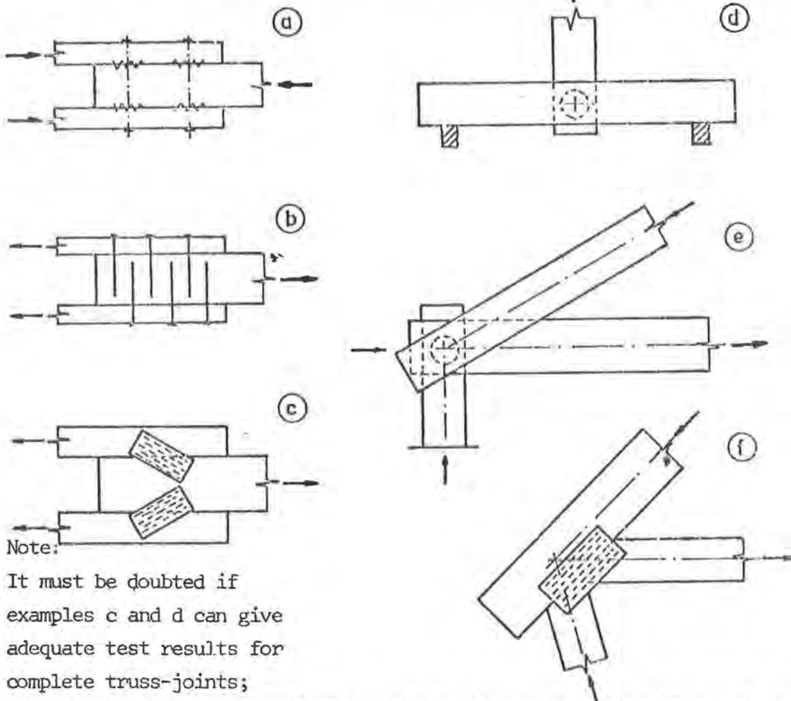
Fig. 1. Examples of test specimens.
