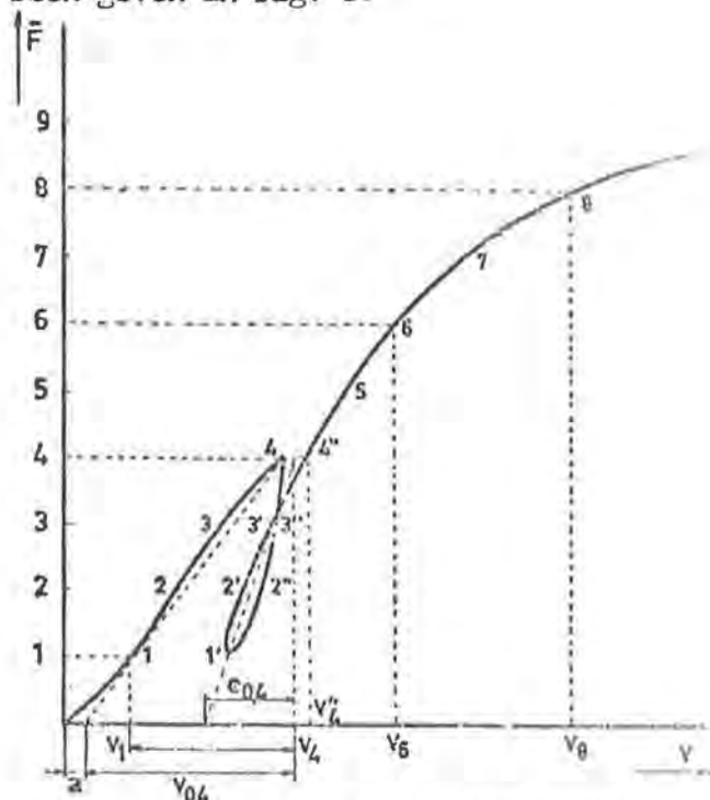
fig. 3 Idealised load-deformation curve and measurements.
