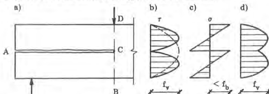
Fig. 4.01. In b) --- denotes stress distribution in an unchecked beam, and — in a checked beam.
