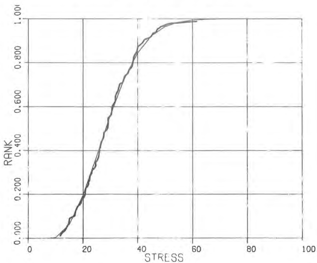
Fig 5 SAMPLE 2. Cumulative distribution and the 3-parameter Weibull cumulative function
