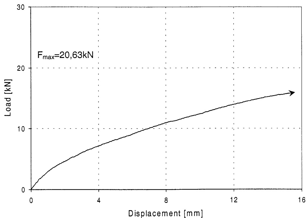
Figure 124: Load-displacement-curve of test Gil8.8-4-2
