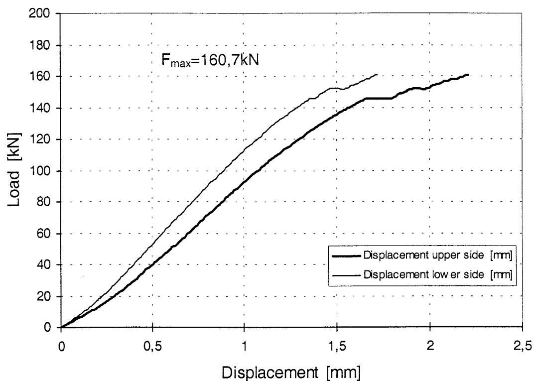
Figure 8: Load-displacement-curve of test Gi2-1
