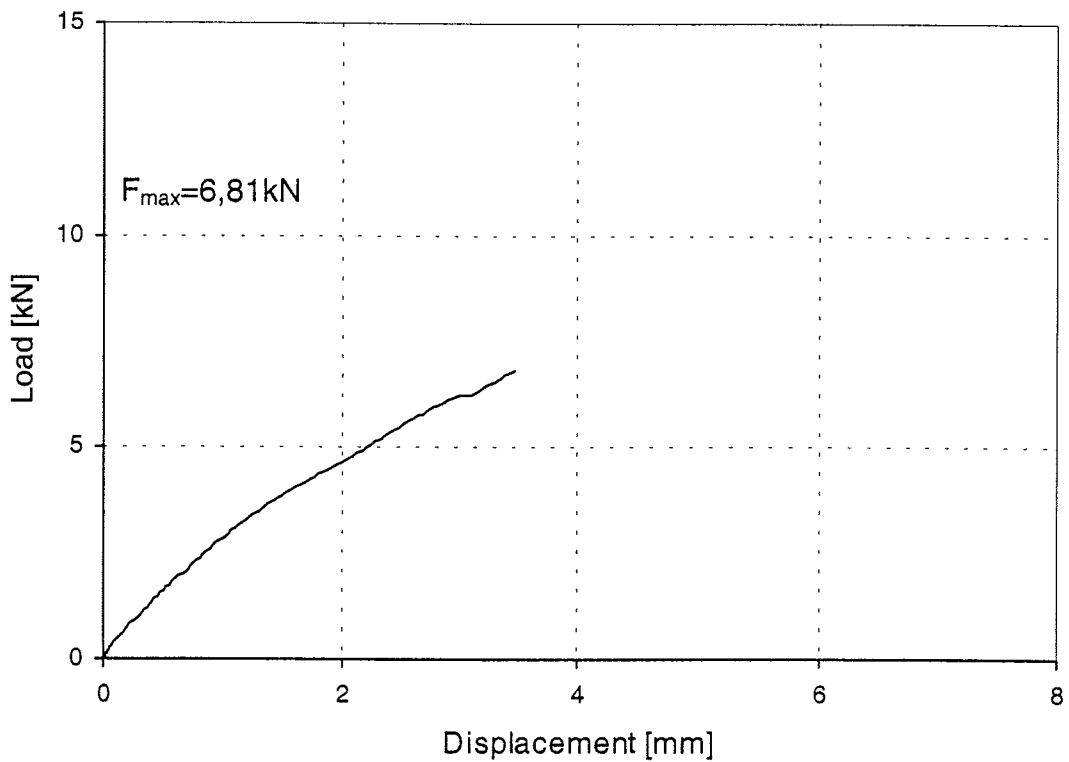
Figure 116: Load-displacement-curve of test Gil8.8-2-4
