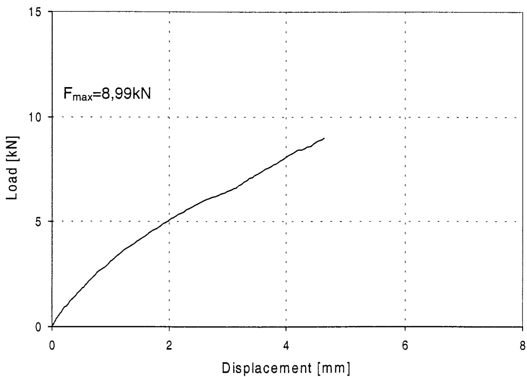
Figure 134: Load-displacement-curve of test Gil8.8-6-2
