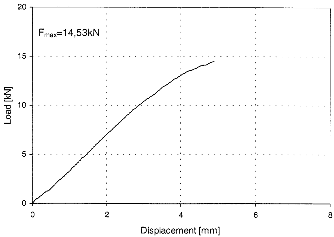
Figure 142: Load-displacement-curve of test Gilll-1-5
