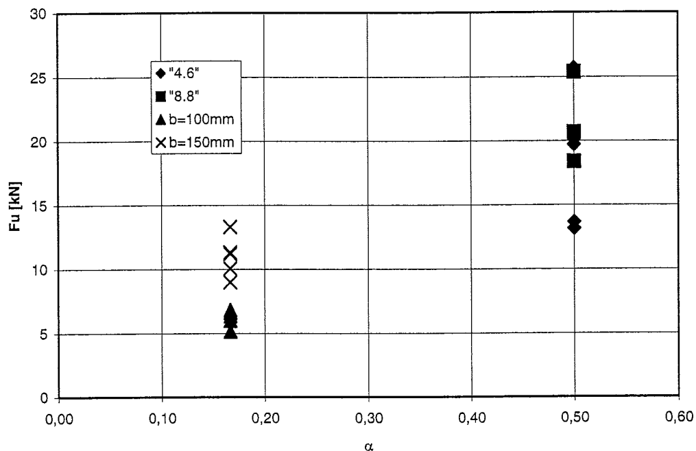
Figure 31: Comparison of different test results
