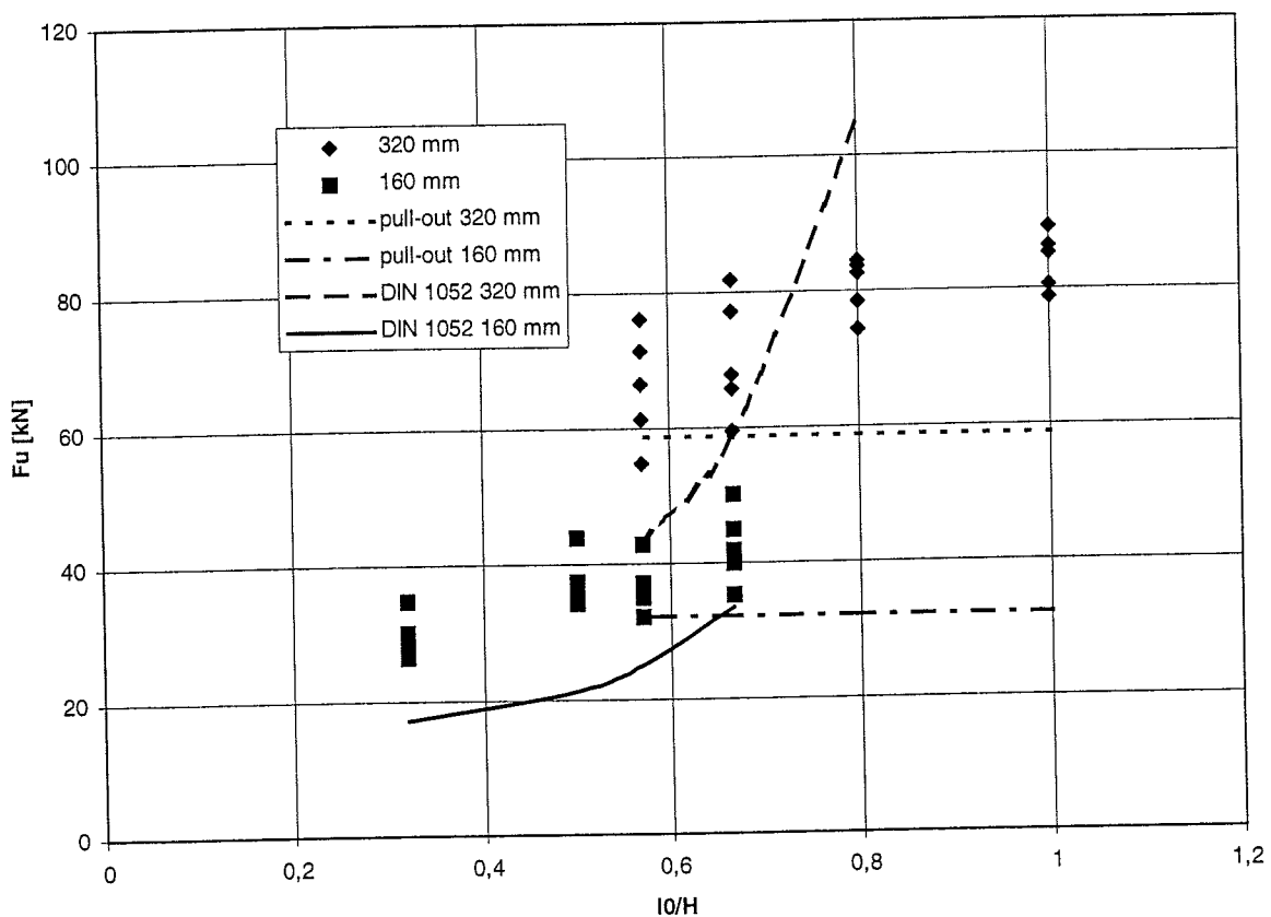
Figure 23: Test results compared to equations according to DIN 1052 [5]
