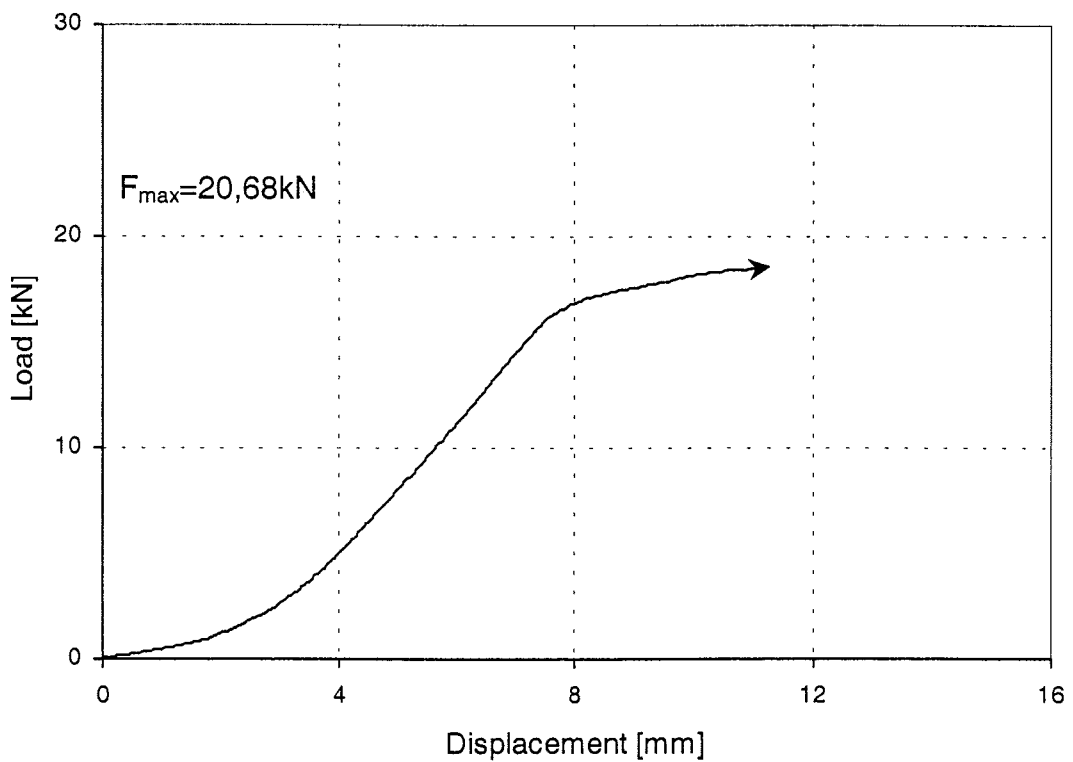
Figure 110: Load-displacement-curve of test Gil8.8-1-2
