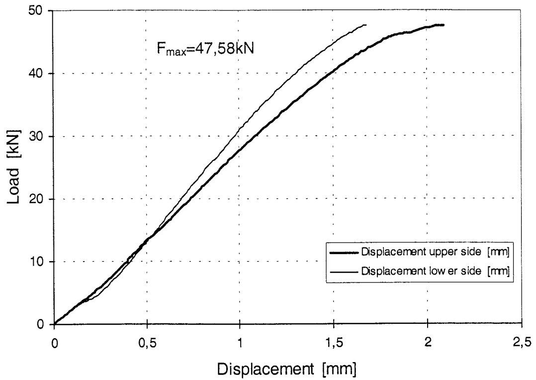
Figure 43: Load-displacement-curve of test Gi9-5
