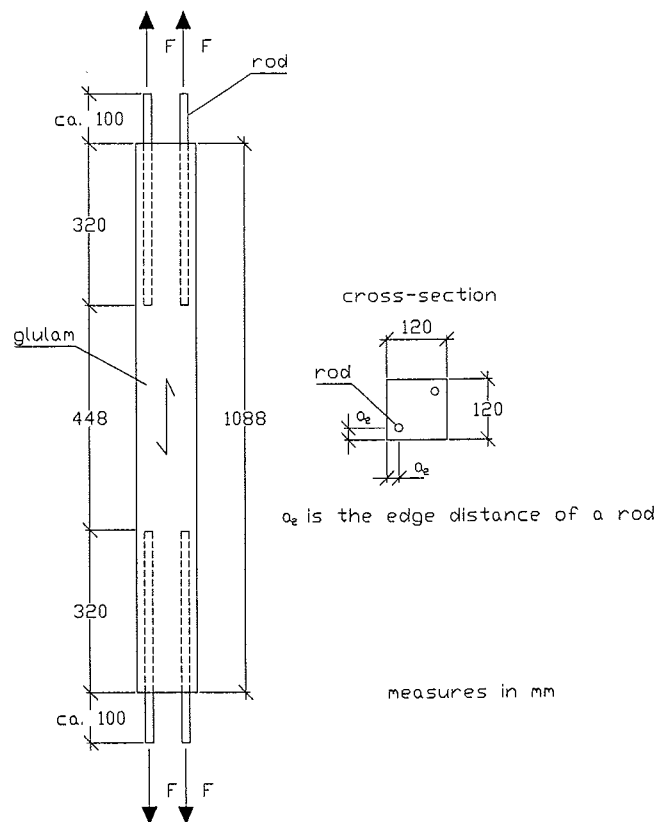
Figure 4: Dimensions, design and loading arrangement of specimens for axial loading (two rods glued-in parallel to the grain)
