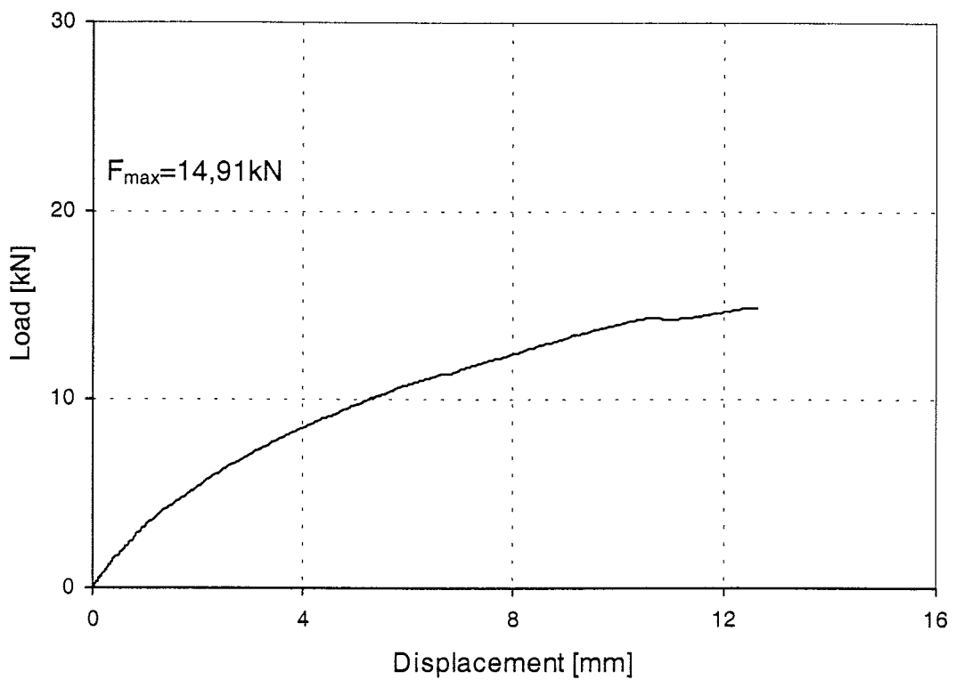
Figure 119: Load-displacement-curve of test Gil8.8-3-2
