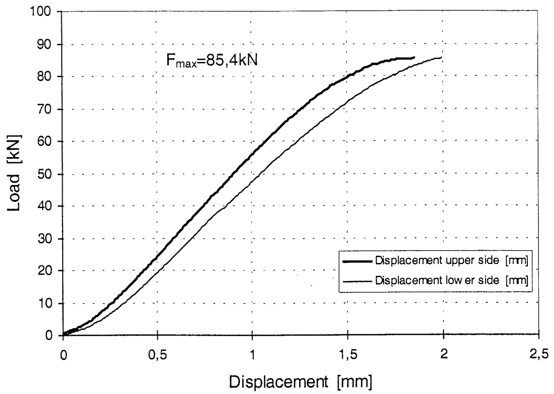
Figure 27: Load-displacement-curve of test Gi5-5
