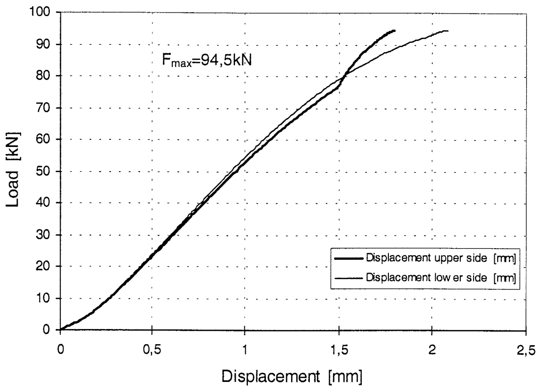
Figure 24: Load-displacement-curve of test Gi5-2
