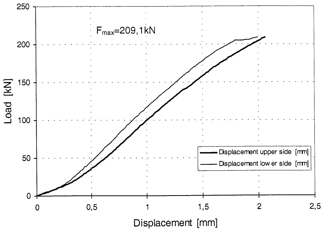
Figure 51: Load-displacement-curve of test Gi32-3
