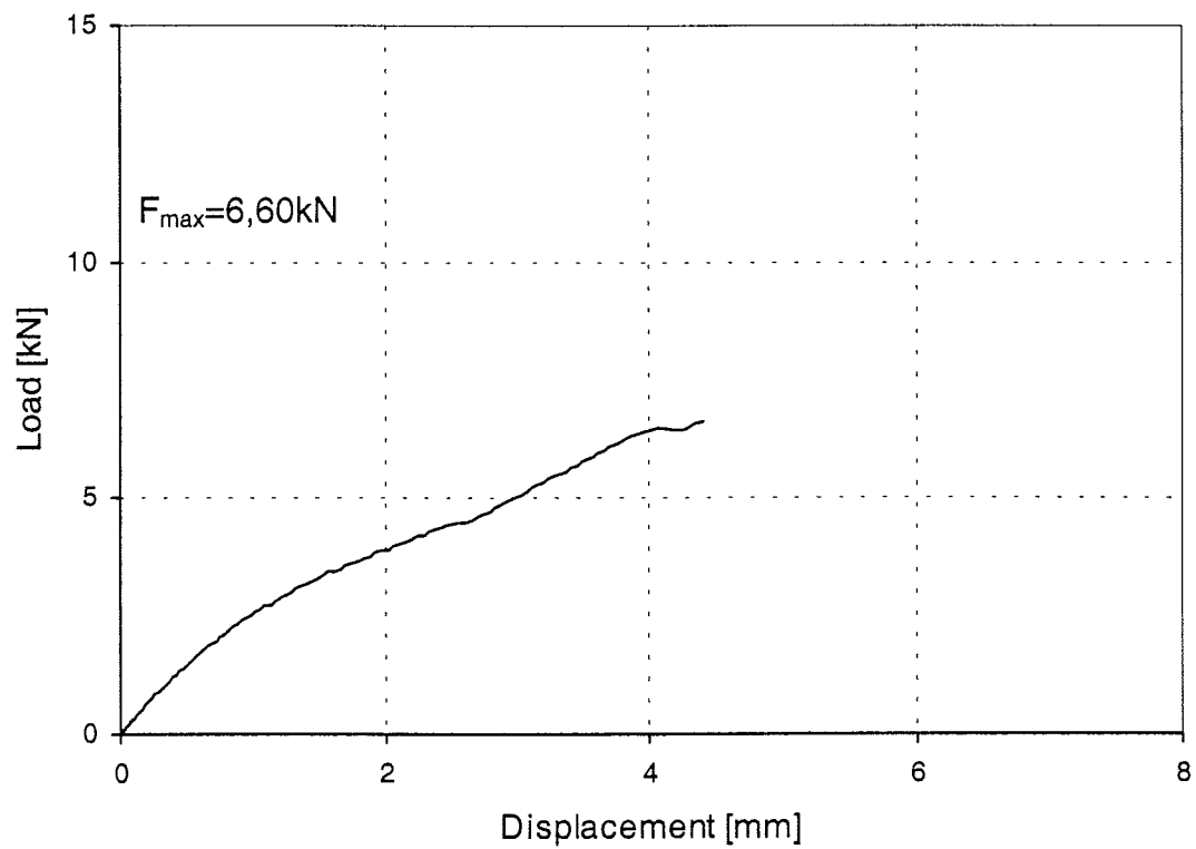
Figure 114: Load-displacement-curve of test Gil8.8-2-2
