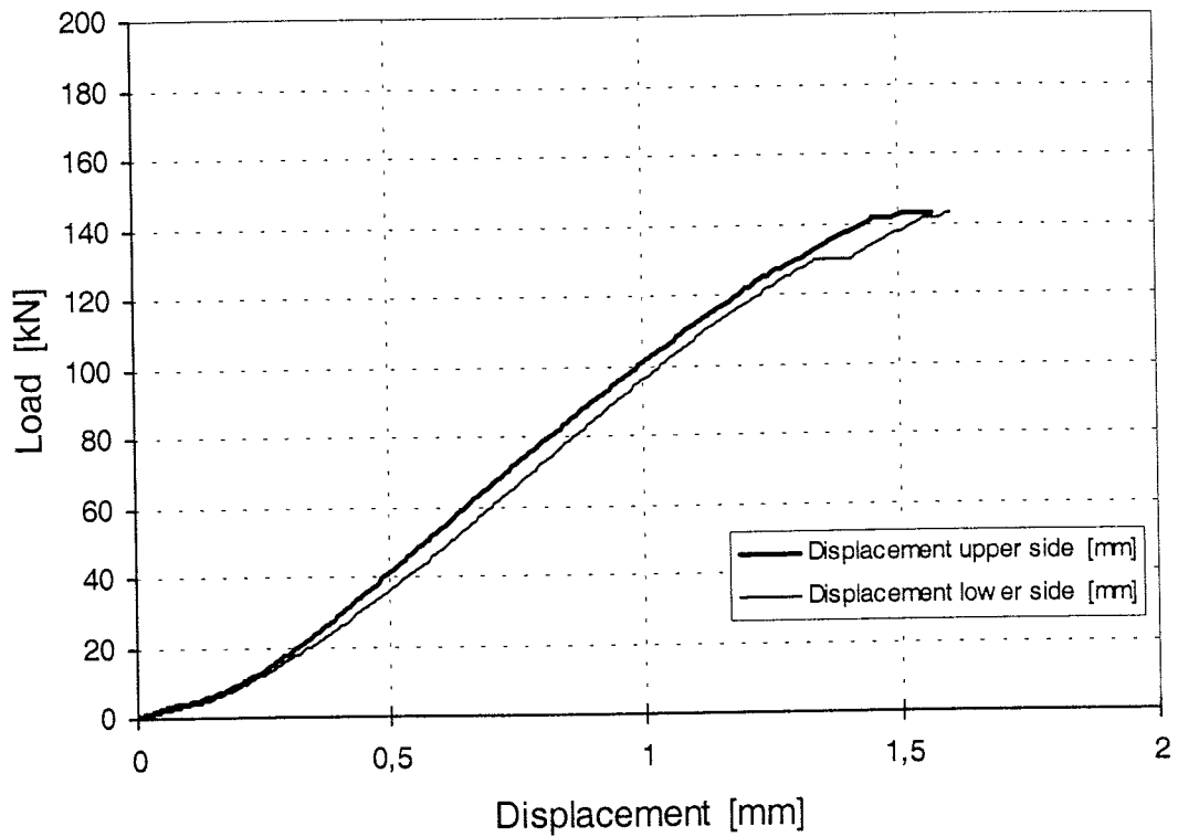
Figure 5: Load-displacement-curve of test Gi1-3
