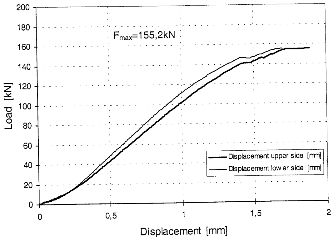
Figure 6: Load-displacement-curve of test Gi1-4
