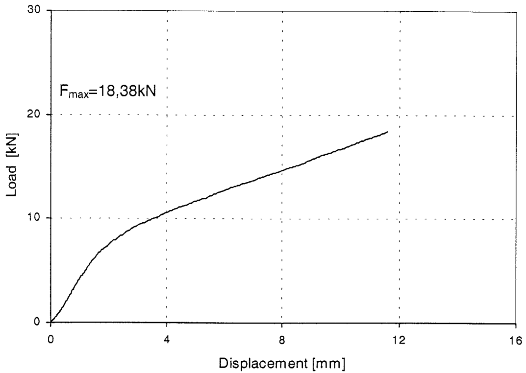
Figure 109: Load-displacement-curve of test Gil8.8-1-1
