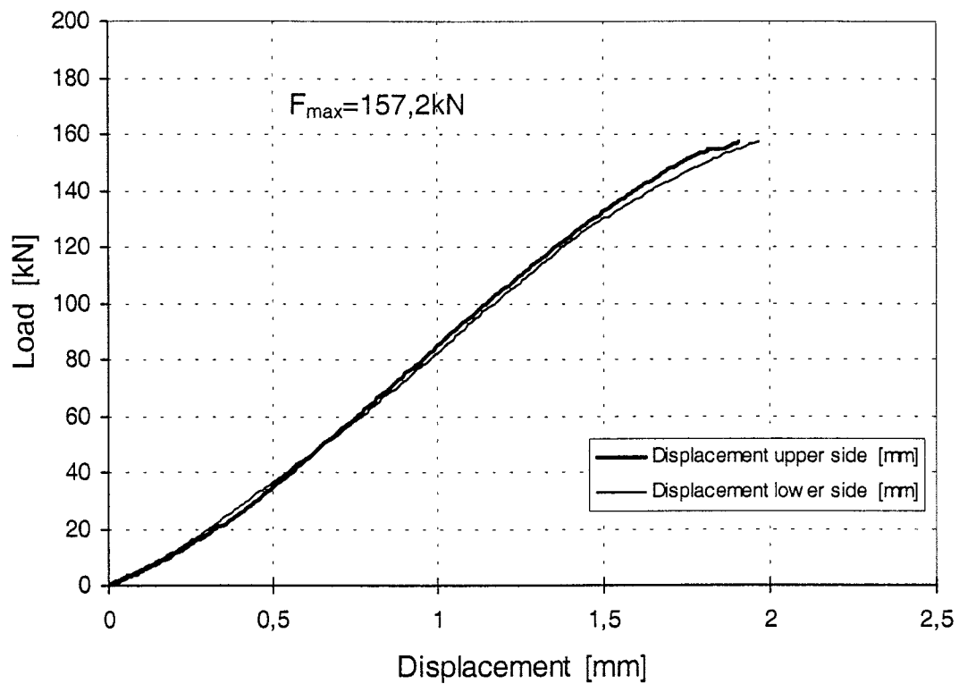
Figure 14: Load-displacement-curve of test Gi3-2
