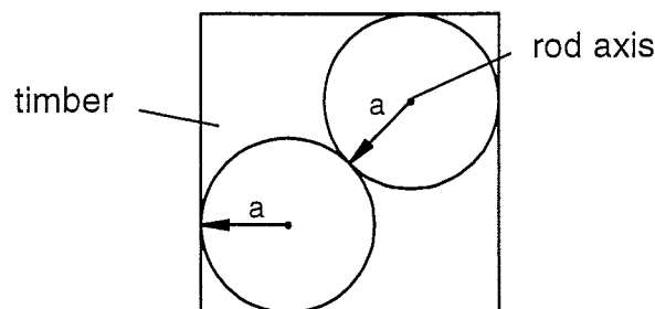
Figure 13: Definition of distance a
