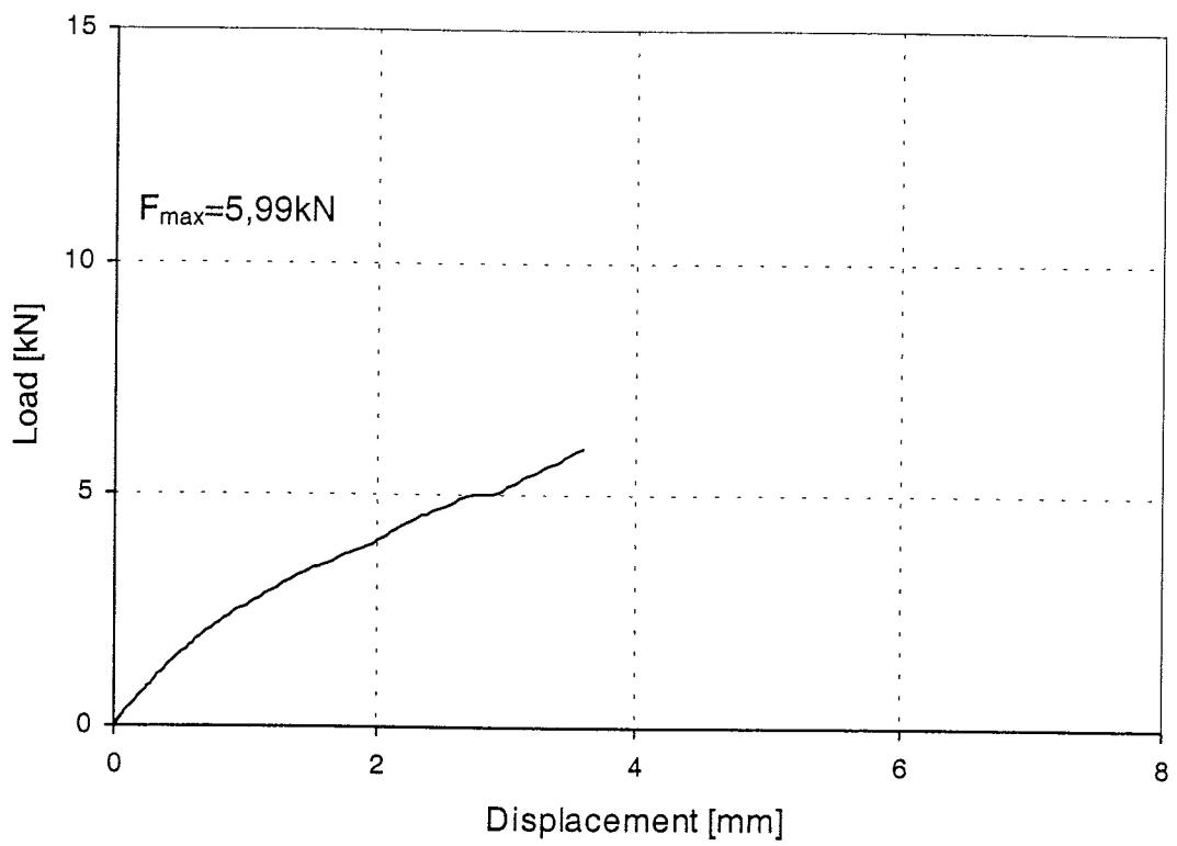
Figure 117: Load-displacement-curve of test Gil8.8-2-5
