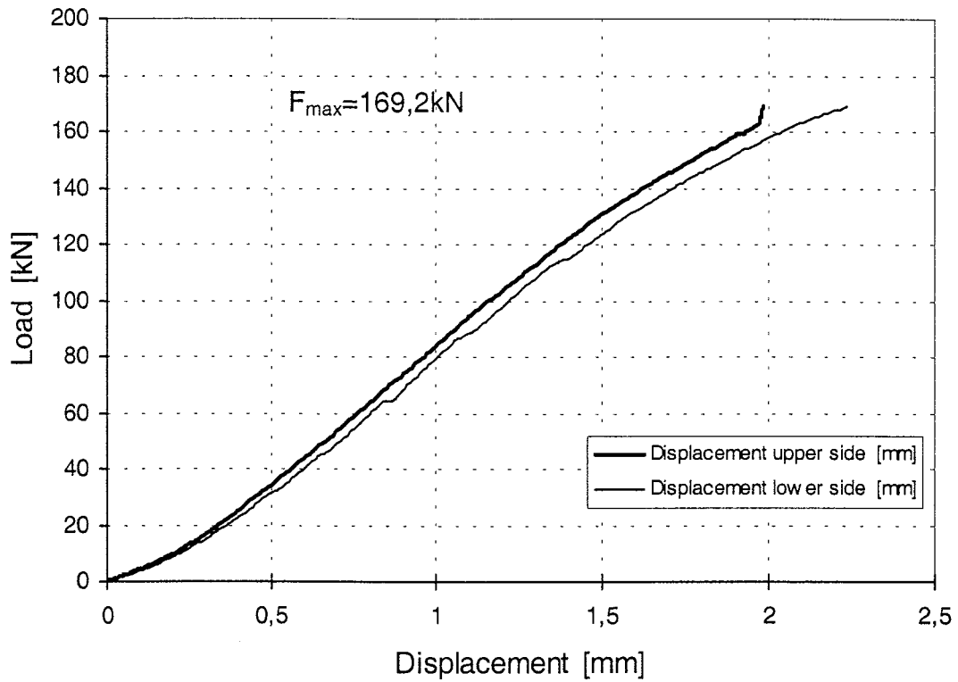
Figure 13: Load-displacement-curve of test Gi3-1
