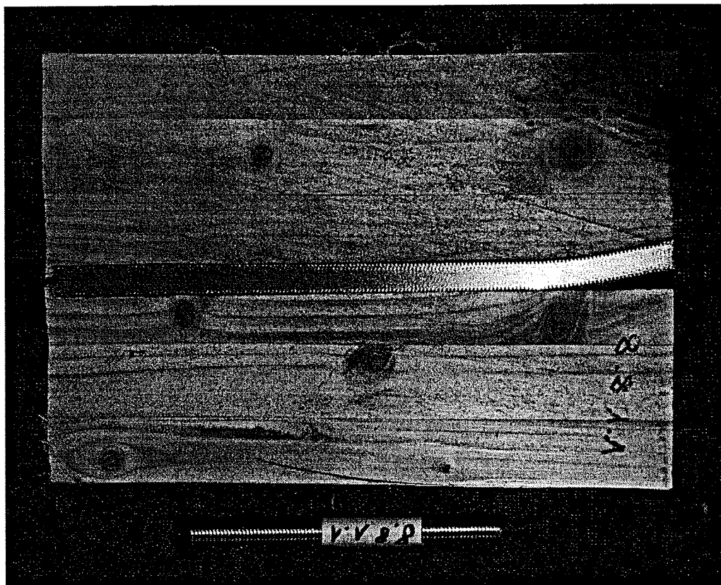
Figure 28: Opened specimen
